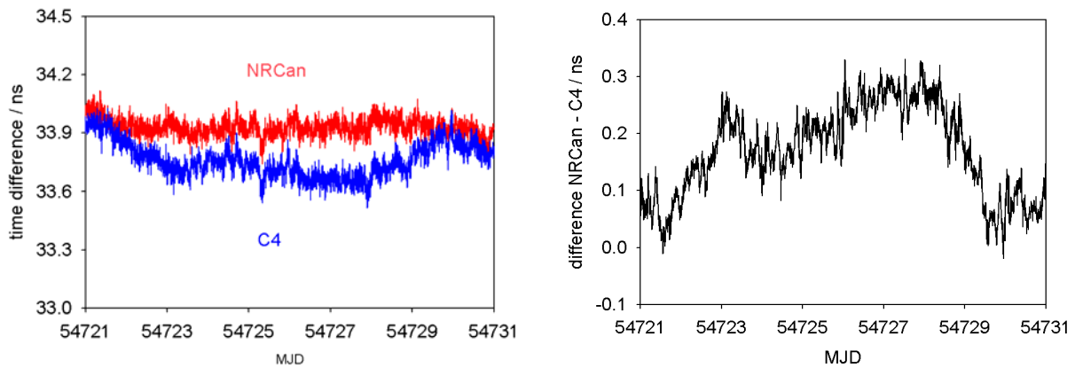
Figure 4. Cutout from a longer period with a typical divergence between C4 and NRCAN-PPP common-clock zero-baseline solution.
