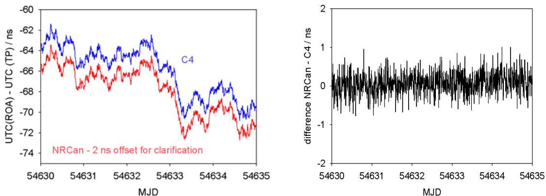
Figure 5. Takeout from a longer GPSCP measurement ranging from MJD 54584 to 54648 between ROA and UFE. The results are on a 5 min basis. These data are by courtesy of ROA and UFE.
