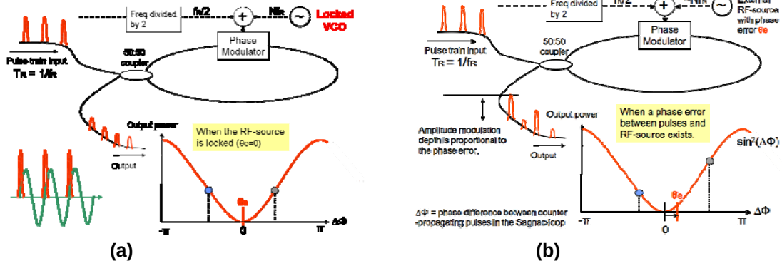
Figure 1. Loop diagram for an optical phase-locked oscillator for locking a Voltage-Controlled Oscillator (VCO) to a mode-locked laser pulse stream. A pulse stream from a mode-locked laser is fed into a Sagnac loop mirror with a phase-shifter offset within the loop. A microwave VCO drives the phase modulator. When the VCO is synchronous (a) with the timing of the mode-locked laser pulse train, the clockwise and counter-clockwise pulses receive the identical phase shift and no modulation of the output is observed. However, when a timing error between the VCO and the mode-locked laser exists (b), a non-zero output signal at the frequency f_R/2 is produced, which is multiplied down to baseband to produce an error signal that then drives the VCO back into synchronization with the mode-locked laser.
