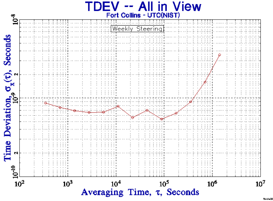
Figure 10. The time deviation of the difference (Fort Collins – Boulder) using weekly steering.
