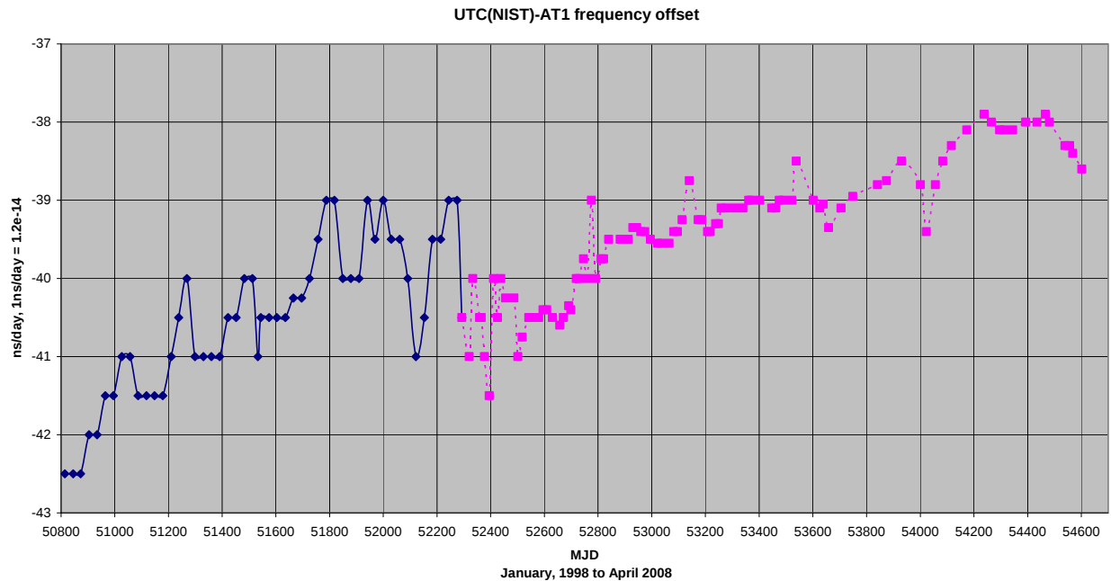
Figure 2. Steering corrections UTC (NIST) - AT1. Blue is slow steering; pink is moderate steering.
