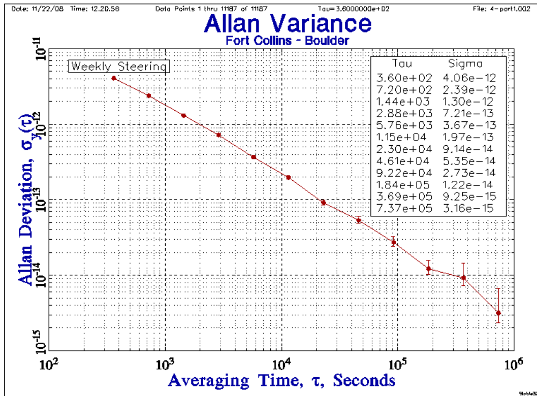
Figure 8. The Allan deviation of the difference (Fort Collins – Boulder), weekly steering at Fort Collins.
