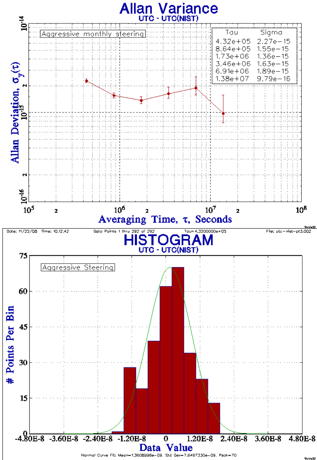
Figure 5. Allan deviation and histogram of time differences with aggressive steering.
