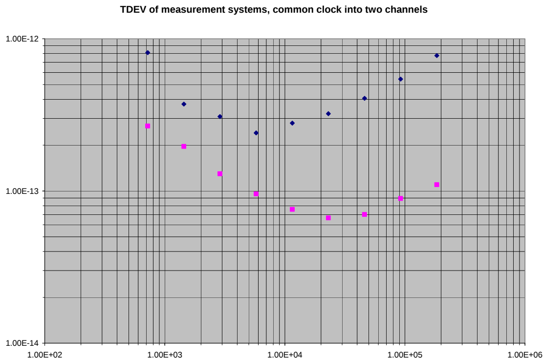
Figure 1. The best and worst TDEV (s) vs. averaging time (s) of time difference between same clock in two channels.
