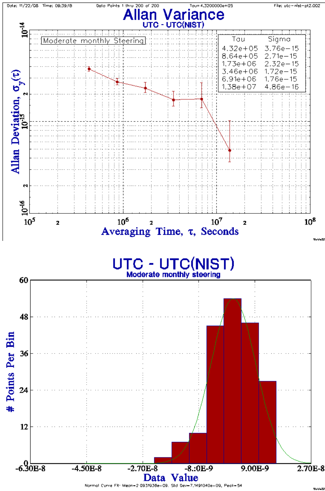
Figure 4. Allan deviation and histogram of time differences for moderate monthly steering.
