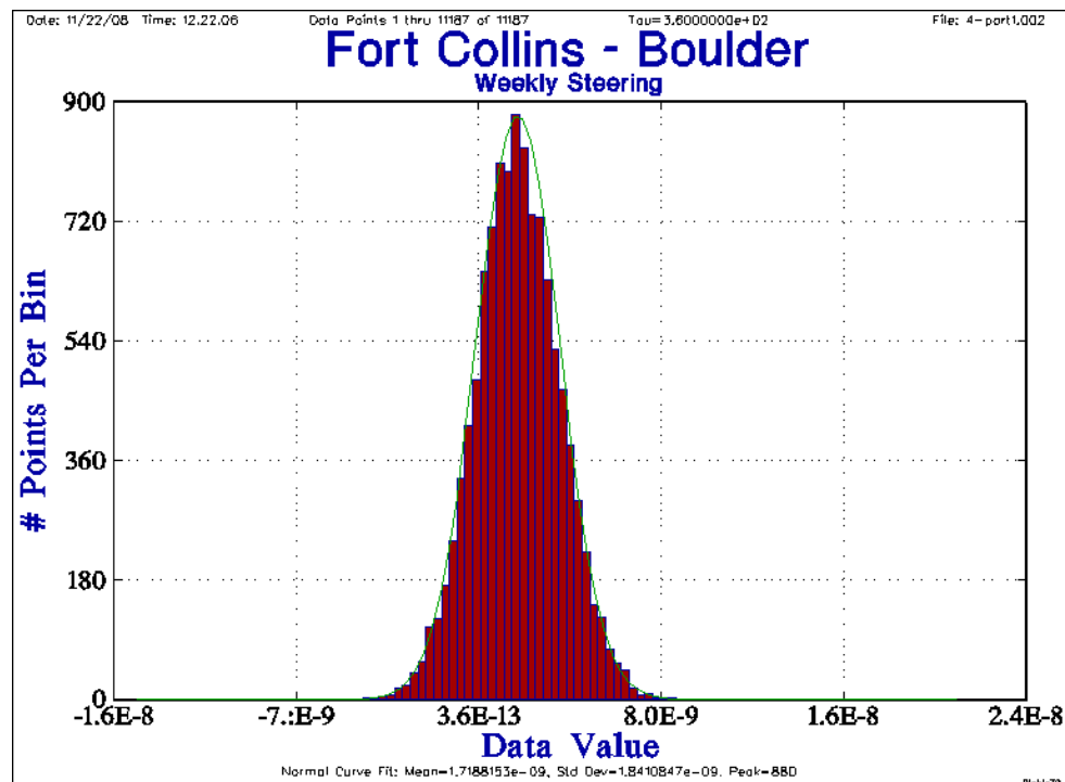
Figure 9. The histogram of the difference (Fort Collins – Boulder) using weekly steering at Fort Collins.
