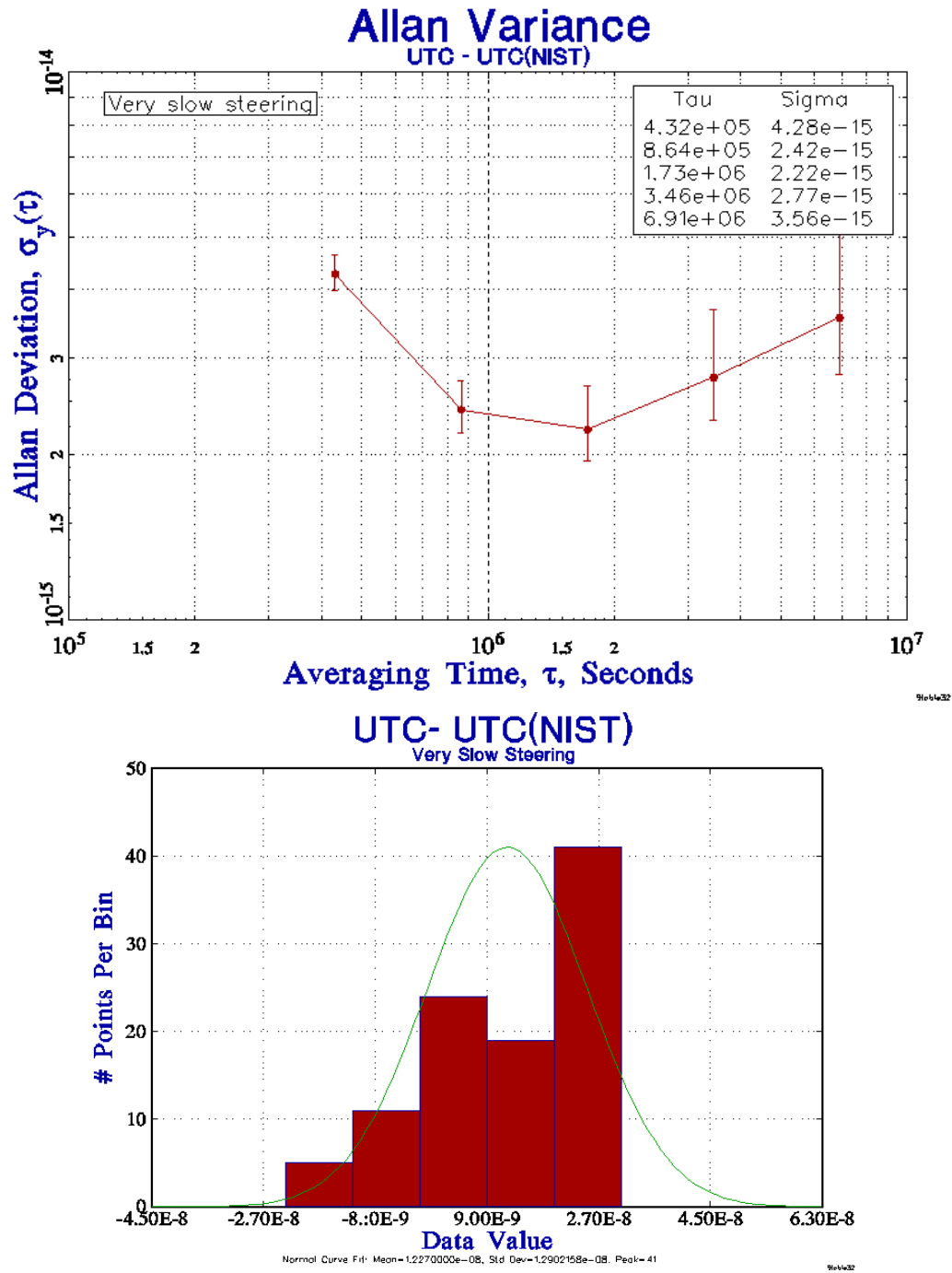
Figure 3. Allan Deviation and histogram of time differences with slow steering.
