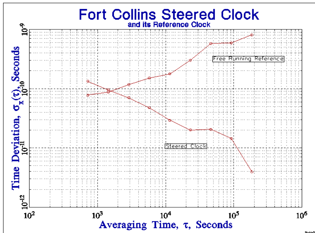
Figure 6. The time deviation of the steered clock compared to the clock used as its reference.
