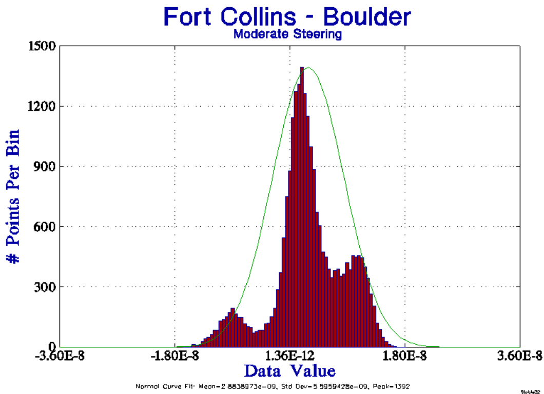
Figure 7. The histogram of the time differences when very slow steering is used.
