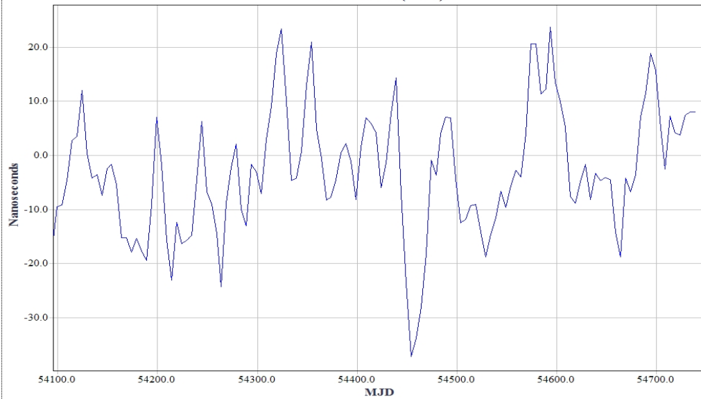
Fig. 9. Past 2 years of UTC – UTC (APL) accuracy.
