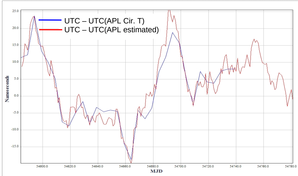
Fig. 6. Comparison of UTC – UTC (APL estimated) and UTC – UTC (APL) as reported in the Circular T. Note continuing estimation of UTC (APL) over 40 days following last Circular T reported data.
