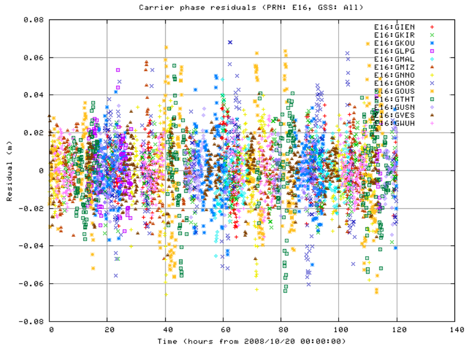
Figure 6. Carrier-phase residuals.
