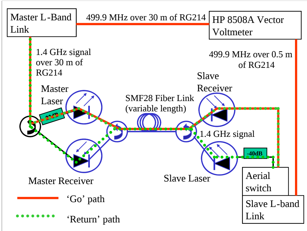
Figure 1. Experimental setup.
