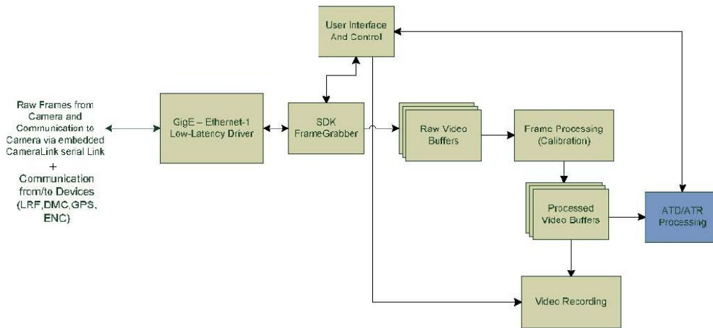
Fig. 4 Data acquisition and control processing
