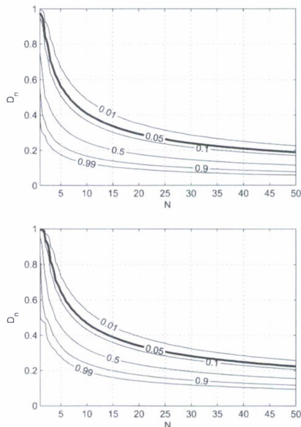
Fig. 3. Contour plots of the confidence level \alpha as a function of N and D_n for the one-dimensional (upper panel) and two-dimensional (lower panel) Kolmogorov–Smirnov test. For a given N and D_n , the latter gives a higher confidence level.
