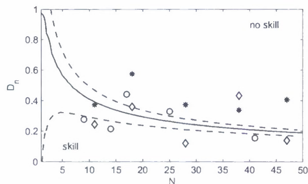
Fig. 6. Combinations of drifting buoy data set length N and test statistic D_n for the five sections of Fig. 4 and Table 1 for NCOM (circles), the ORCA model (asterisks) and the AGO1 model (diamonds). The thick black line is the line where \alpha = 0.05 , the divider between a model that lacks or might have skill according to the decision rule, Eq. (3). The area between the dashed lines denotes the region where in the worst-case scenario one extra drifting buoy could make \alpha cross the 0.05 line. Only decisions inside this area are subject to change when an extra drifter is introduced.
