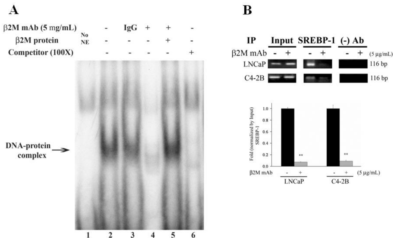
Fig. 5. \beta 2M mAb inhibited the interaction between SREBP-1 and its binding cis -acting element located in the 5'-flanking hAR promoter region in prostate cancer cells. A, Electrophoretic Mobility Shift Assay (EMSA). LNCaP cells were exposed to \beta 2M mAb, control IgG (5 \mu g/mL) or vehicle for 24 h in a serum-free condition. Cells were harvested and nuclear extracts were prepared. EMSA was performed by incubating nuclear extracts with the ^{32} P-labeled SREBP-1 oligo-DNA probe and Novex TBE system (Invitrogen). Lane 1 was no nuclear extracts added. Lanes 2 and 3 showed the nuclear protein-SREBP-1-oligo-DNA complex was formed and this complex did not affect by control IgG. Lane 4 showed \beta 2M mAb greatly inhibited this nuclear protein-DNA complex formation. Purified \beta 2M protein could rescue the inhibitory effect by \beta 2M mAb (lane 5). This complex was competed off by adding 100-fold of the ^{32} P-unlabeled specific SREBP-1 oligo-DNA probe (lane 6). B, Chromatin Immunoprecipitation Assay (ChIP). LNCaP and C4-2B cells were treated with or without \beta 2M mAb (5 \mu g/mL) for 24 h. The chromatin and nuclear proteins were cross-linked by formaldehyde and sheared by Enzymatic Shearing Cocktail (ChIP-IT kit, Active Motif, Inc.), and subjective to immunoprecipitation assay by using anti-SREBP-1 antibody or without antibody as a negative control. Analysis of the PCR product from chromatin DNA fragments immunoprecipitated by anti-SREBP-1 antibody as templates, a predicted single DNA band (116 bp, top panel) was amplified and visualized in LNCaP and C4-2B cells. This PCR product was decreased by treated with \beta 2M mAb in prostate cancer cells. In addition, quantitative real-time PCR of ChIP was performed (bottom panel). Quantitative PCR showed that \beta 2M mAb significantly caused downregulation of the interaction between SREBP-1 and SREBP-1 binding site at the 5'-flanking region of hAR promoter by 13.3 and 11.0-fold decrease in LNCaP and C4-2B cell, respectively. The quantitative PCR data were normalized by input and assigned as 1.0-fold without treating \beta 2M mAb for each prostate cancer cell line. **, P < 0.005 .
