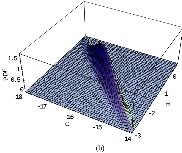
Figure 9. Examples of input to the simulation of the life-limiting probability density, f_i(x) ; (a) The crack initiation size distribution for the NMP initiated cracks in terms of the diameter of the equivalent circle, and (b) The joint PDF of the small crack growth variables, C and m for the case of 0 dwell time.
