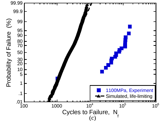
Figure 10. The CDFs of the calculated life-limiting probability densities for the case of no-dwell; (a) \sigma_{\max} = 1200 MPa, (b) \sigma_{\max} = 1150 MPa, and (c) \sigma_{\max} = 1100 MPa.
