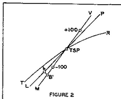
TR—Normal trajectory TSP—Expected point of burst LP—Line of position from the gun MV—Differential effect line from muzzle velocity. B'—Point of burst for low muzzle velocity.
