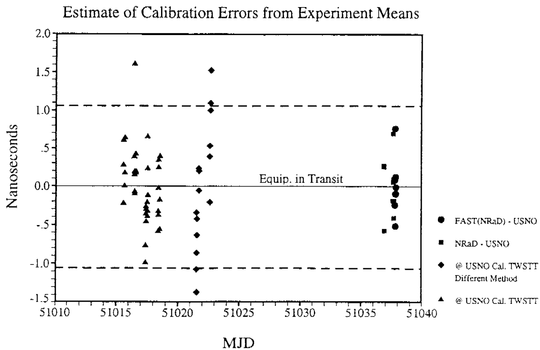
Fig. 10 USNO - NRaD Syntonization and Single-Shot Synchronization
