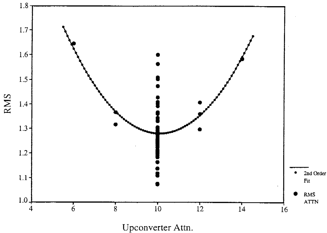
X-Band (FX2) Baseline TWSTT Experiment RMS Behaviour w/Signal Varied into HPA
