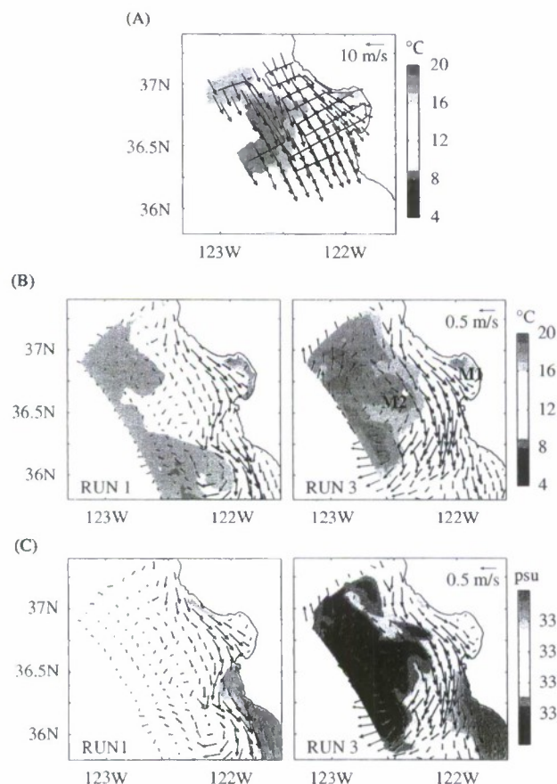
Fig. 8. Comparisons of aircraft and model-predicted SSTs for August 15, 2003. (A) Aircraft measured SSTs with wind velocities overlay. (B) Model-predicted SSTs and surface currents for Runs 1 and 3. (C) Model-predicted surface salinity and currents for Runs 1 and 3.
