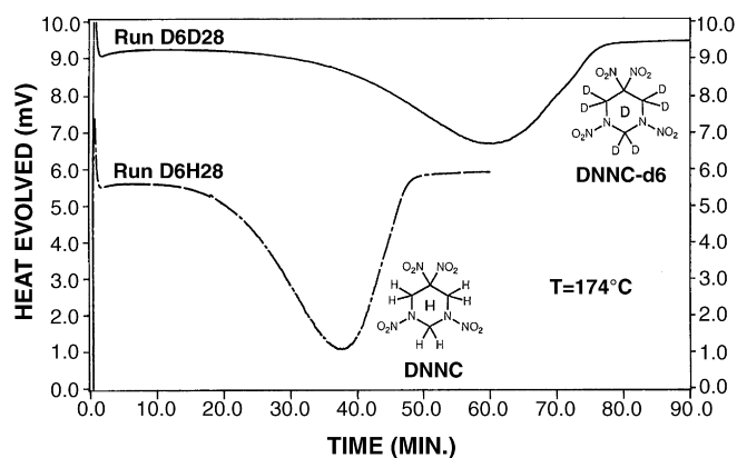
Fig. 7. Individual DNNC and DNNC- d_6 IDSC thermograms compared at 174 °C.
