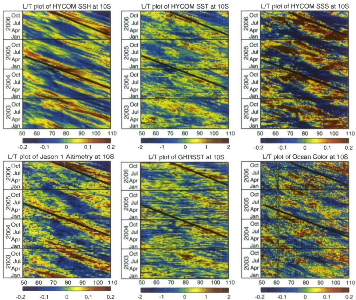
Fig. 1. Longitude–time plots at 10°S of parameter anomalies. (Top panel) HYCOM simulations of SSH, SST, SSS, and (bottom panel) satellite-derived parameters of Jason-1 altimetry, GHRST, and Log of chl- a concentration. The solid lines represent Rossby waves' propagation.
