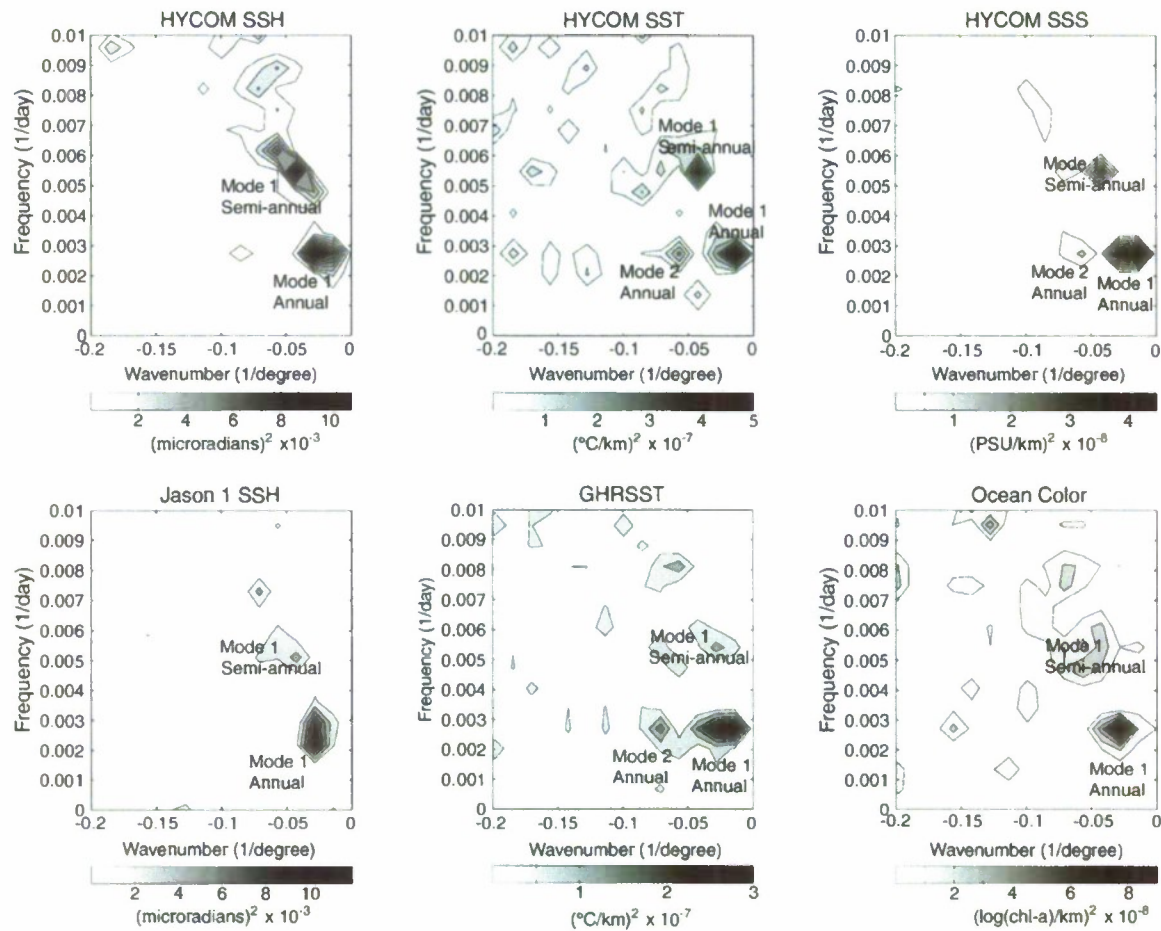
Fig. 3. Fast Fourier Transform (FFT) of (top panel) HYCOM simulations, and (bottom panel) satellite-derived parameter gradients from longitude/time plots at 10°S.
