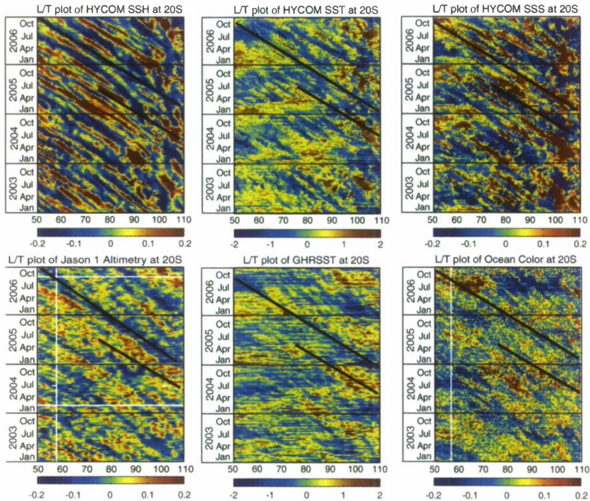
Fig. 2. Longitude–time plots at 20°S of parameter anomalies. (Top panel) HYCOM simulations of SSH, SST, SSS, and (bottom panel) satellite-derived parameters of Jason-1 altimetry, GHRST, and Log of chl- a concentration. The solid lines represent Rossby waves' propagation.
