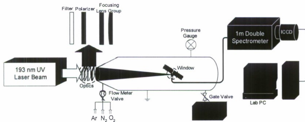
Fig. 9: Experimental setup for focused laser breakdown.
