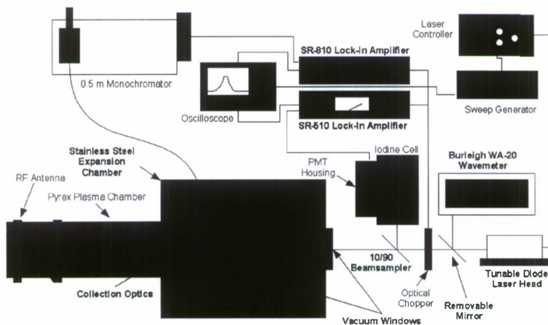
Figure 17: Laser-induced fluorescence diagnostic (DURIP-funded additions have blue captions)
