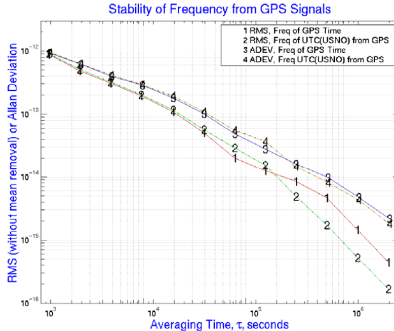
Figure 7. RMS fractional frequency external precision and the fractional frequency stability, as measured by the Allan deviation, of GPS Time and for GPS's delivered prediction of UTC (USNO), using TTR-12 data since 7 February 2005. The reference frequency is that of UTC (USNO).
