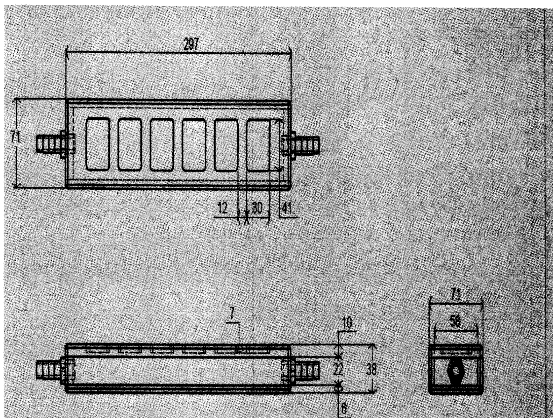
Fig. 2. Blood-feeding reservoir design. All measurements are in centimeters.
