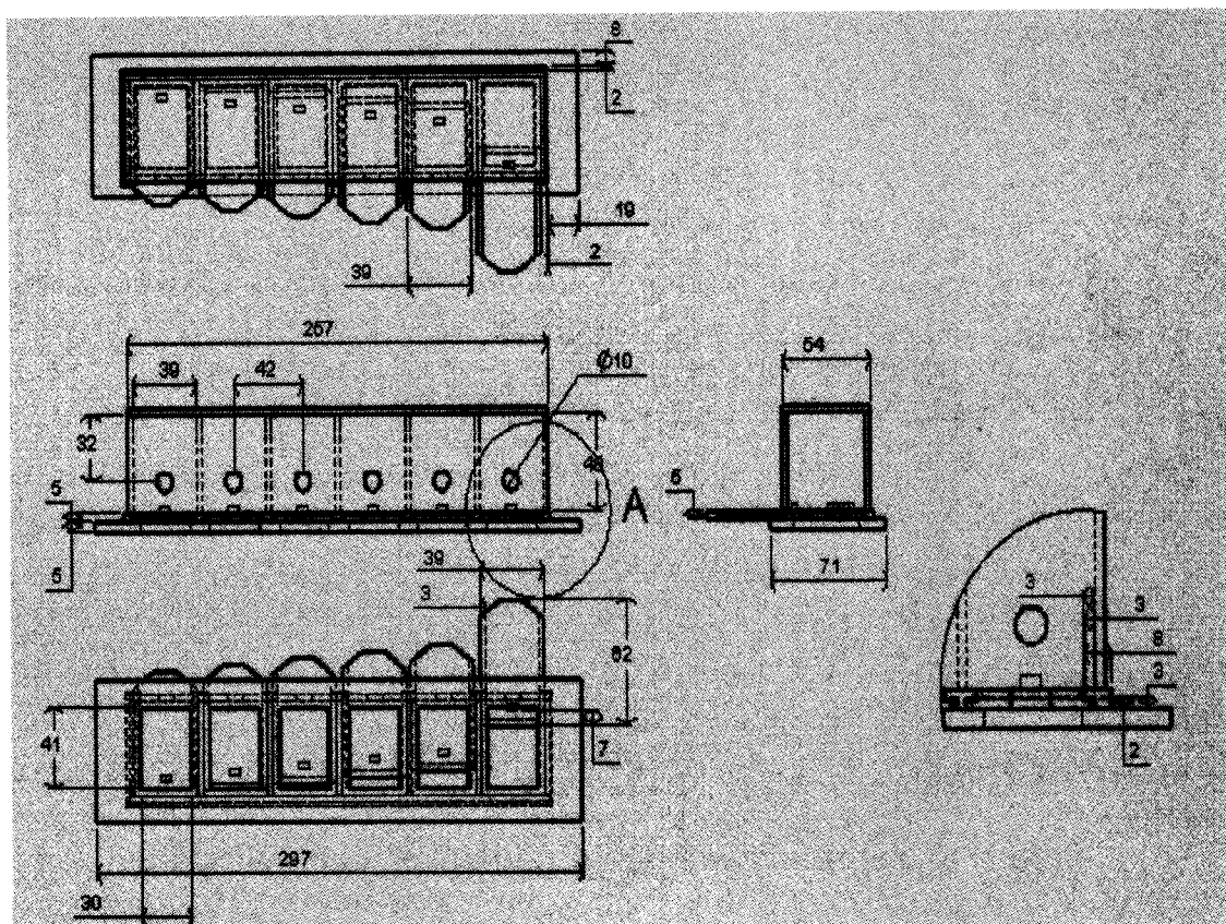
Fig. 1. Modified 6-celled Klun & Debboun module design. All measurements are in centimeters.
