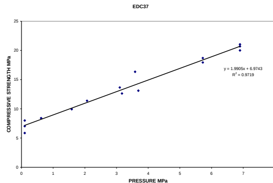
Figure 2. Compressive strength versus pressure for pressures in the low pressure range.
