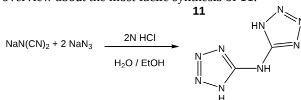
Scheme 5. Synthesis of H 2 bta ( 11 )
