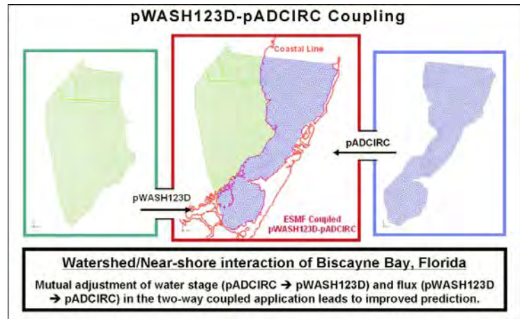
Figure 5. Computational meshes
