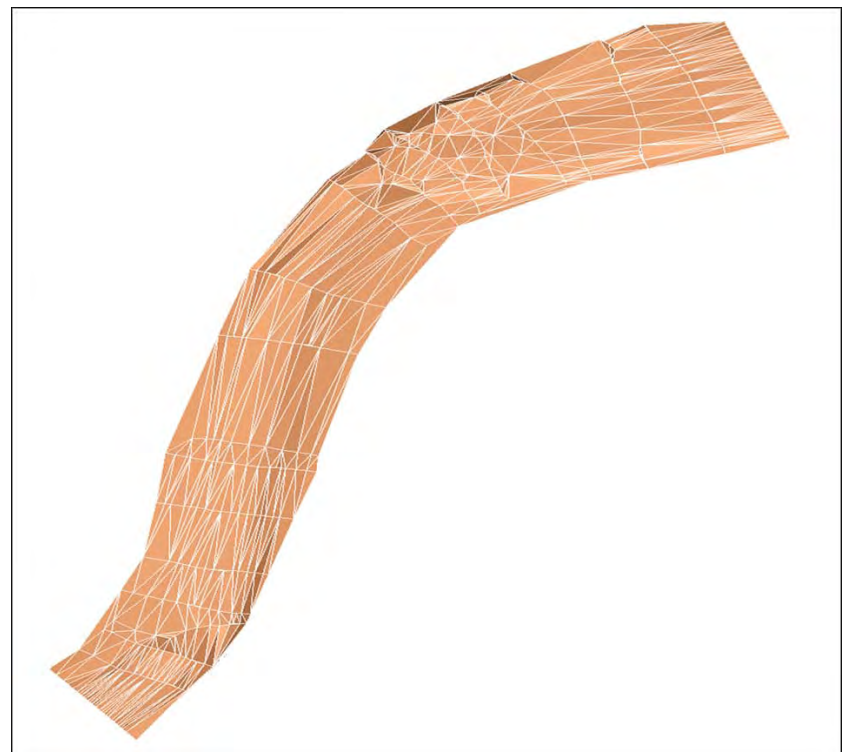
Figure 2. Initial triangulation
