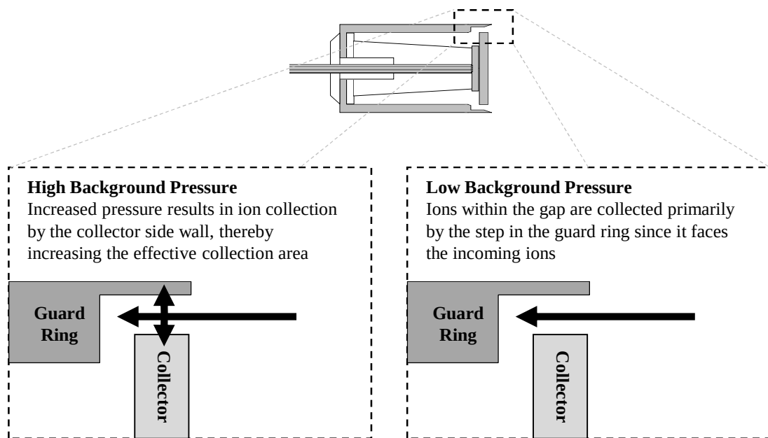
Figure 4-25 Illustration of the distribution of ions in the gap volume of the JPL Faraday probe for high and low facility background pressure.
