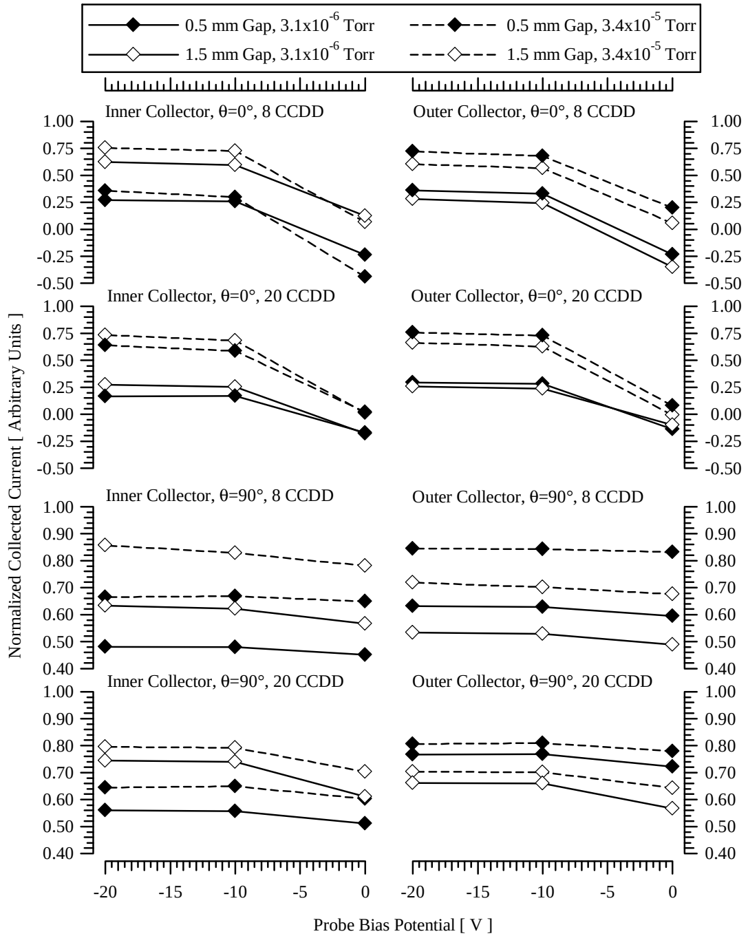
Figure 3-27 Nested Faraday probe bias voltage characterization of the inner collector (left) and the outer collector (right) for the 0.5 mm and 1.5 mm gap configurations at 3.1 \times 10^{-6} Torr and 3.4 \times 10^{-5} Torr. Normalized current is shown at the location of largest Debye length in the plume at \theta=0 degrees and the location of smallest Debye length in the plume at \theta=90 degrees at 8 CCDD and 20 CCDD.
