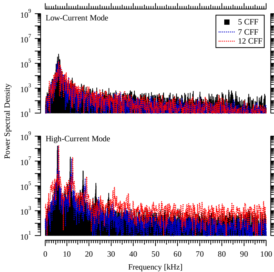
Figure 6-8 Comparison of discharge current oscillation spectra in the low-current mode (top) and high-current mode (bottom) for 120 V, 10 mg/s at 5, 7, and 12 CFF.
