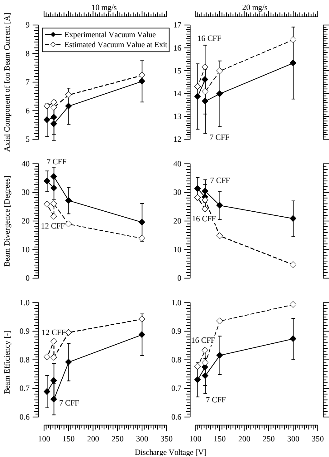
Figure 5-29 Comparison of the axial component of ion beam current (top), beam divergence half-angle (middle), and beam efficiency (bottom) as a function of voltage at 10 mg/s (left) and 20 mg/s (right) anode flow rate. Values calculated from Faraday probe measurements extrapolated to vacuum are compared to the values required to equate performance parameters based on plume measurements with those based on thrust measurements.
