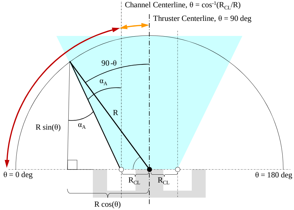
Figure 4-37 Diagram of the axial component of beam current relative to channel centerline.
