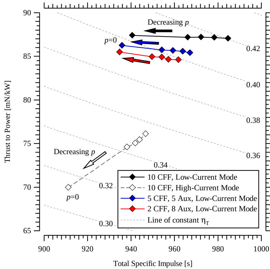
Figure 6-17 Ratio of thrust to power and total specific impulse with variation in cathode flow and auxiliary neutral propellant for 105 V, 20 mg/s operation in the high-current and low-current regimes. The total combined flow to the cathode and auxiliary port is fixed and equivalent to 10 CFF, such that the total propellant flow to the thruster is constant. Performance parameters are extrapolated to vacuum conditions.
