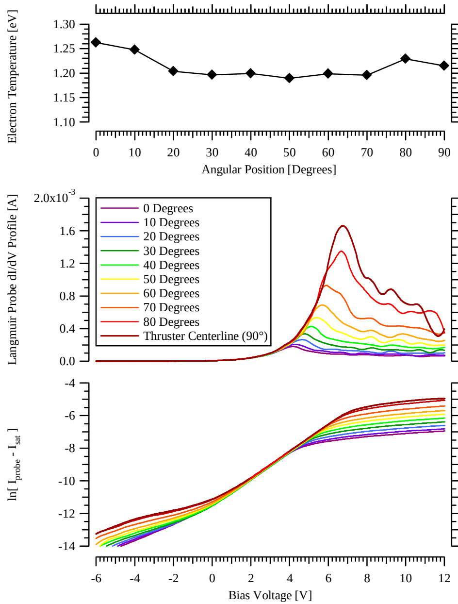
Figure 6-11 Angular variation of electron temperature from 0° to thruster centerline (top). Langmuir probe traces of normalized dI/dV (middle) and the natural logarithm (bottom) located 1-m downstream of the exit plane for 100 V, 20 mg/s, 7 CFF in the high-current operating regime.
