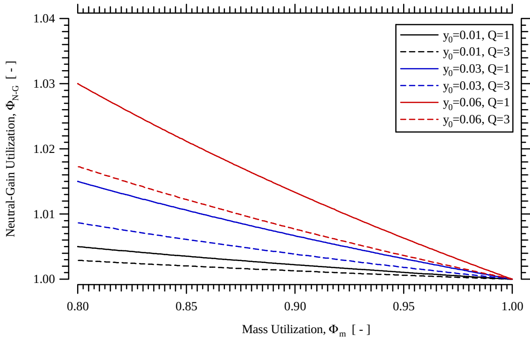
Figure 2-2 Neutral-gain utilization as a function of mass utilization with variations in neutral speed from y_0=0.01 to y_0=0.06 for Q=1 and Q=3 , which are limiting cases for a trimodal ion population.
