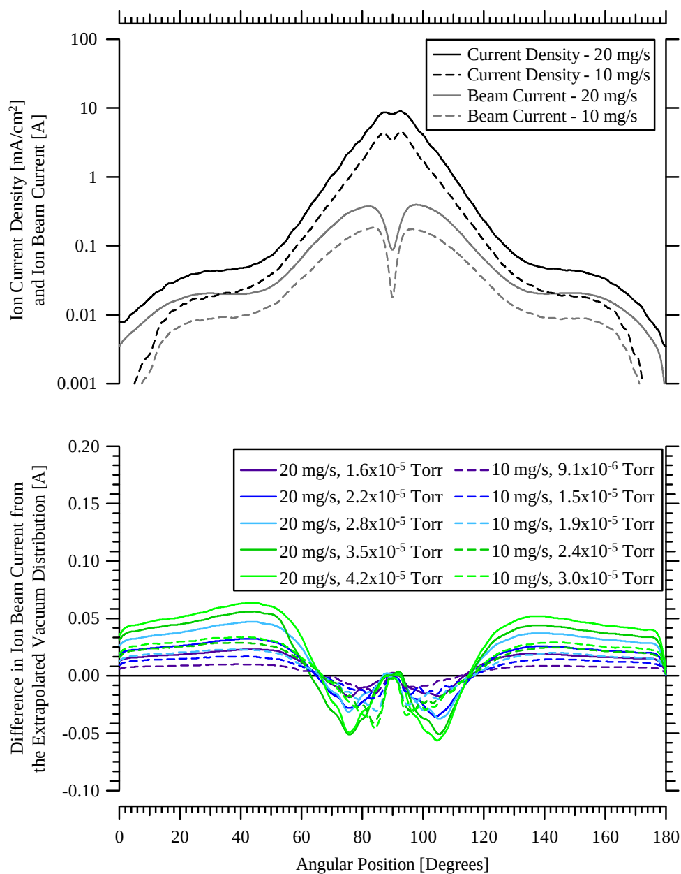
Figure 5-4 Angular distributions of ion beam current extrapolated to vacuum and the angular difference in ion beam current with increasing background pressure for 300 V, 7 CFF at 10 and 20 mg/s anode flow rate.
