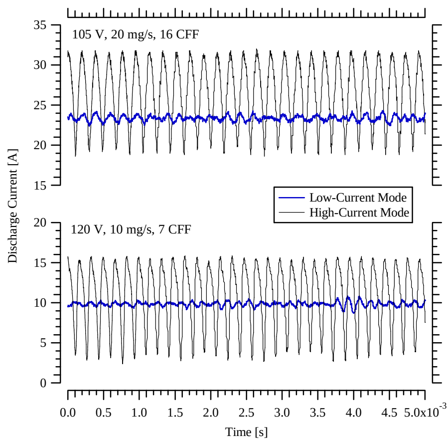
Figure 6-5 Comparison of discharge current oscillations in the low-current and high-current modes for 105 V, 20 mg/s, 16 CFF operation (top) and 120 V, 10 mg/s, 7 CFF operation (bottom) during a 5 ms time period.
