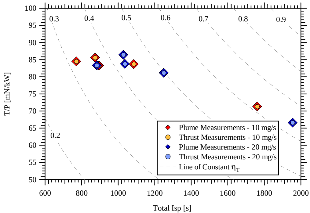
Figure 5-30 Thrust to power ratio, total specific impulse, and total thruster efficiency calculated with plume measurements based on the estimated axial component of ion beam current at the exit compared to calculations based on thrust measurements for 105 V to 300 V at 10 mg/s and 20 mg/s anode flow rate.
