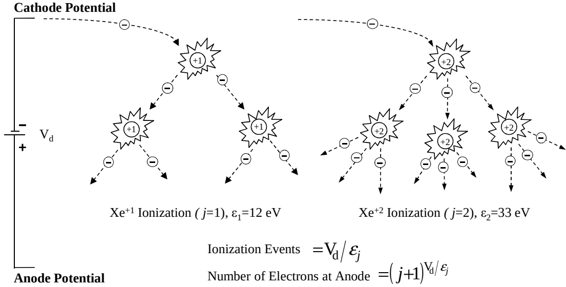
Figure 2-3 Illustration of cascade ionization of singly and doubly charged ions in the Hall thruster discharge.
