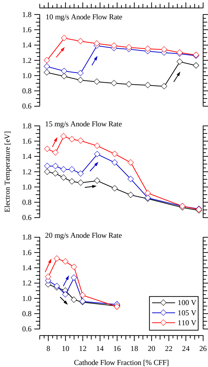
Figure 6-12 Electron temperature on thruster centerline located 1-m downstream of the exit plane for 100 V, 105 V, and 110 V at 10 mg/s (top), 15 mg/s (middle), and 20 mg/s (bottom) with cathode flow fraction ranging from 8 CFF to 26 CFF. Transitions from operation in high-current mode to low-current mode are shown with arrows, indicating the direction of increasing cathode flow fraction.
