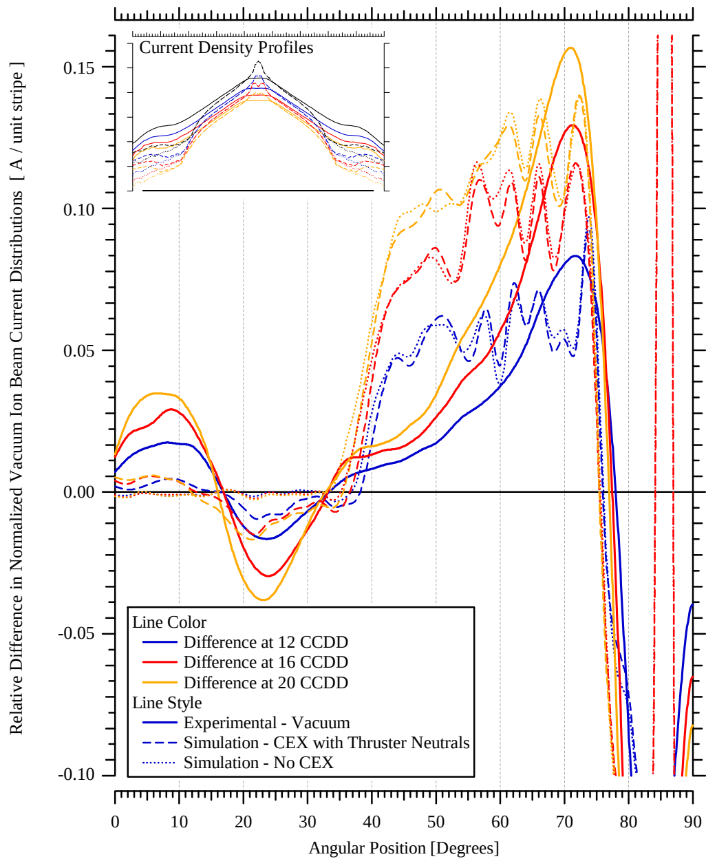
Figure 4-36 Comparison of the simulated and experimental normalized differences in vacuum ion beam current at 12, 16, and 20 CCDD relative to the profile at 8 CCDD as a function of angular position. All profiles are normalized to the maximum extrapolated experimental vacuum beam current at 8 CCDD. The simulated and experimental normalized current density profiles are shown in the small window for reference.
