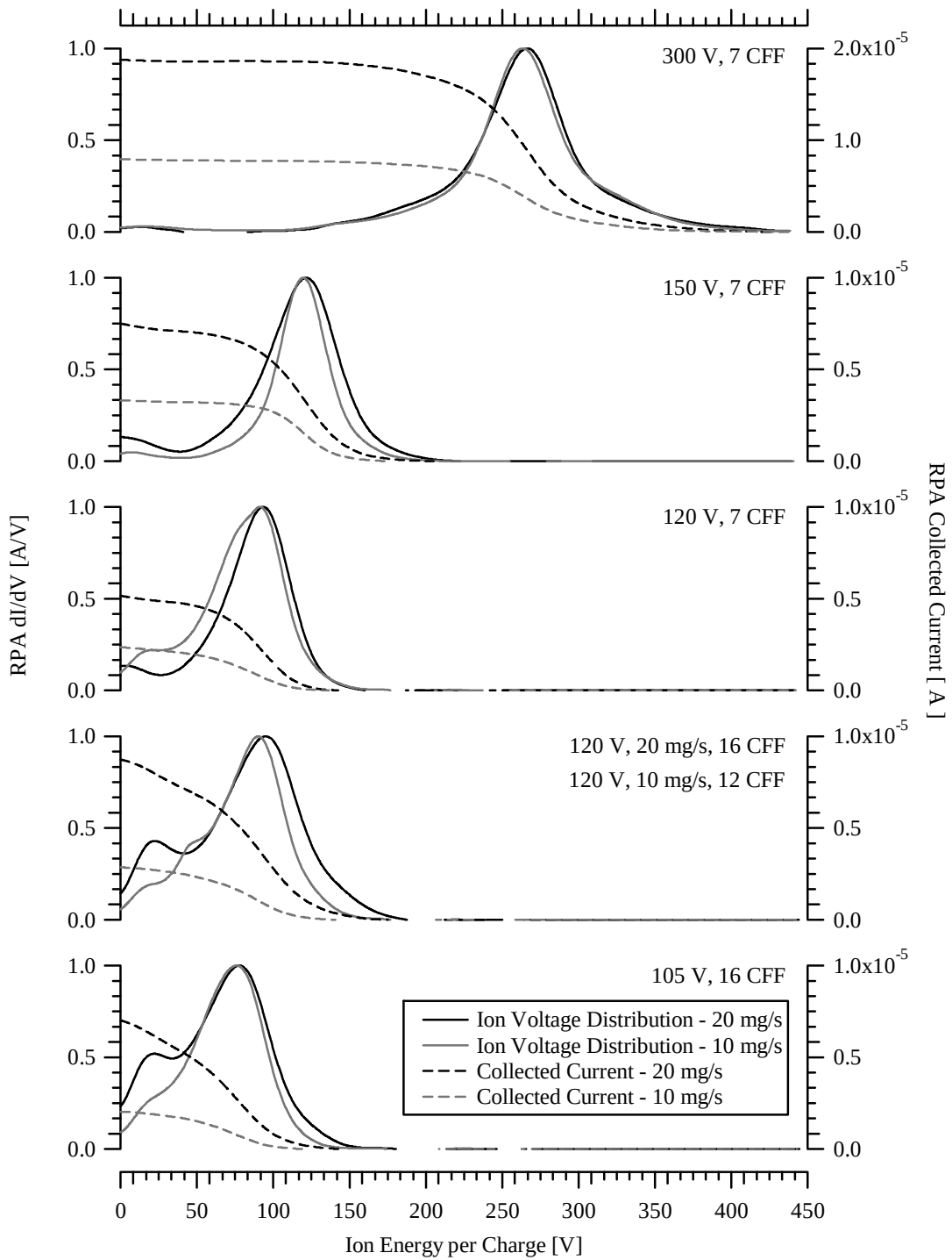
Figure 5-21 RPA collected ion current traces and Normalized RPA ion energy per charge distributions on thruster centerline located 1-m downstream of the exit plane for 105 V to 300 V discharge at 10 mg/s and 20 mg/s anode flow rate.
