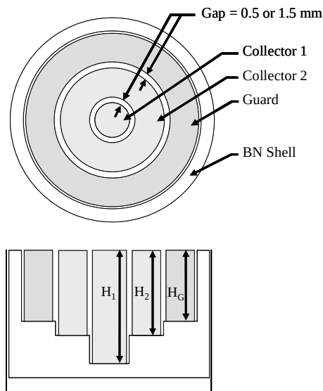
Figure 3-23 Top view and cross-sectional diagrams of the AFRL nested Faraday probe.
