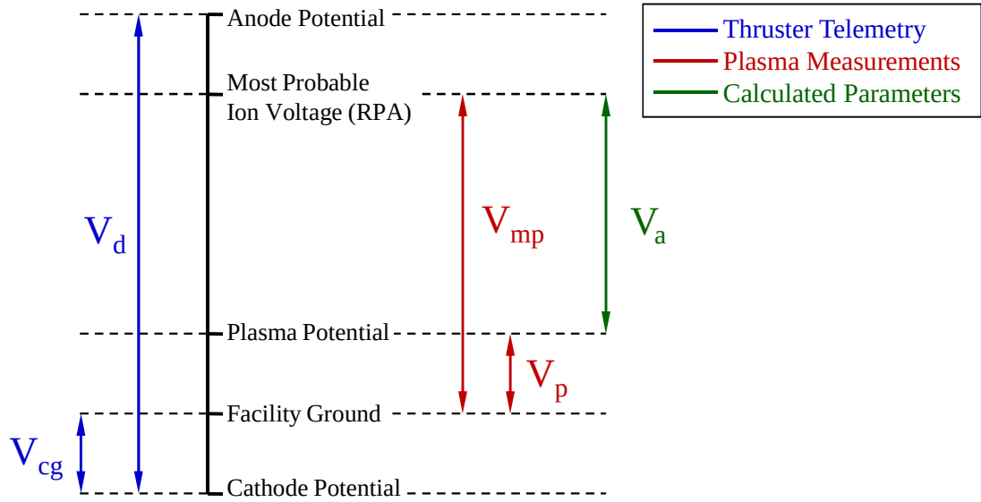
Figure 3-16 Potential diagram illustrating the relationship between measured voltages ( V_d , V_{cg} ), plume measurements ( V_{mp} , V_p ) and calculated potentials ( V_a , V_{loss} ).
