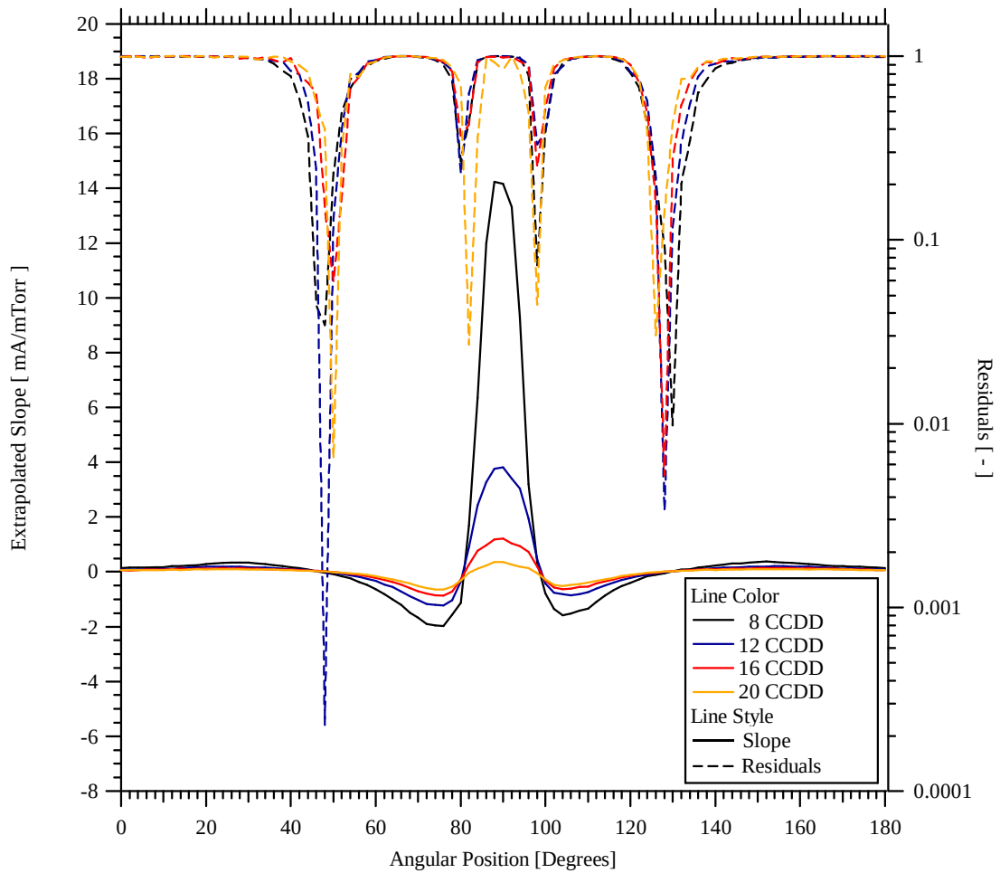
Figure 4-27 Residuals and slope of the extrapolated collected ion current of the nested Faraday probe configuration 1 as a function of angular position at 8, 12, 16, and 20 CCDD.
