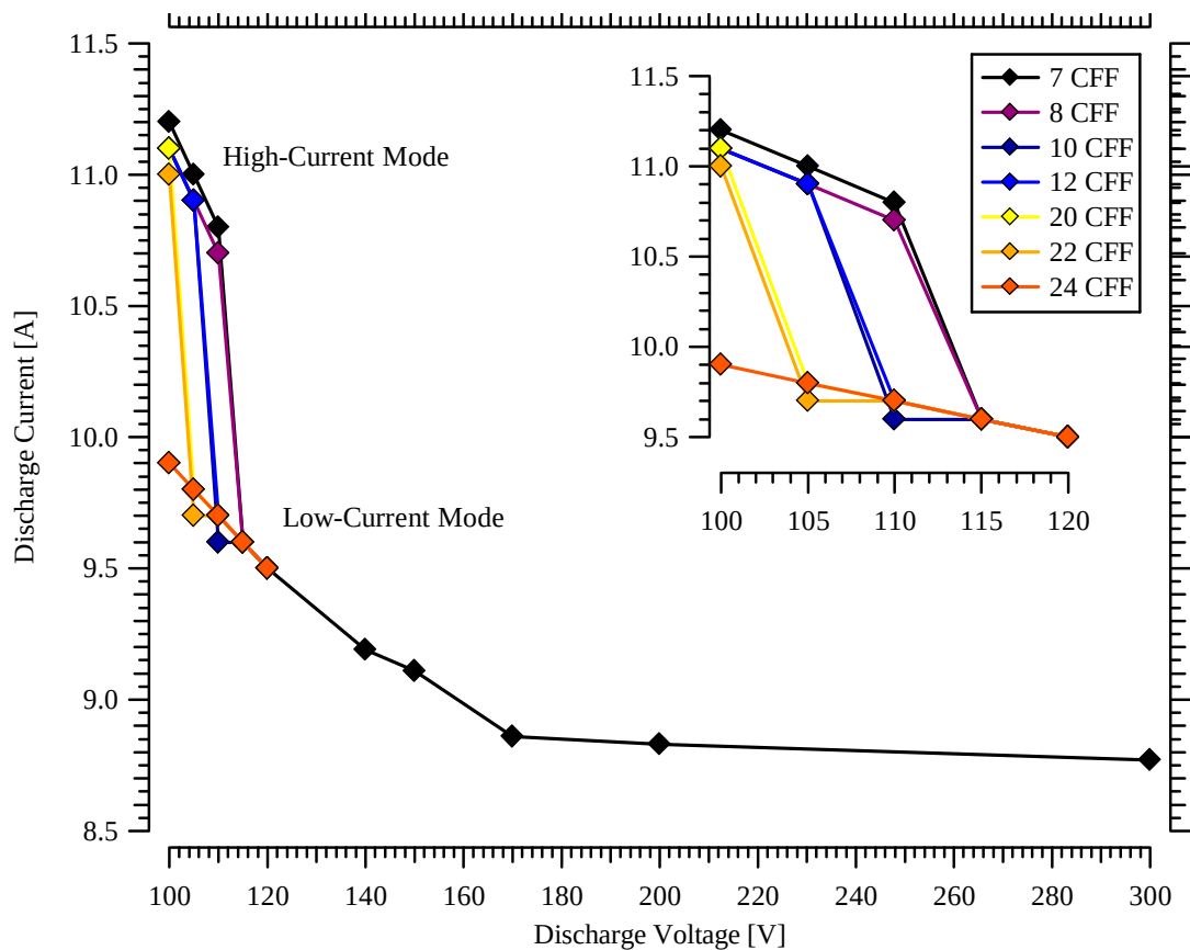
Figure 6-4 Thruster I-V characteristics at 10 mg/s anode flow rate. Lines of constant cathode flow rate operation are shown as a function of discharge voltage from 100 V to 300 V. Low discharge voltage operation is magnified from 100 V to 120 V discharge.
