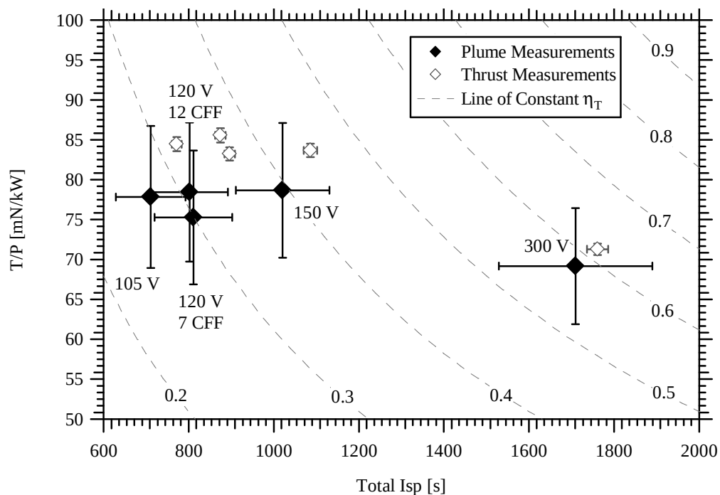
Figure 5-26 Comparison of thrust to power ratio, total specific impulse, and total thruster efficiency calculated with plume properties and thrust measurements for 105 V to 300 V discharge at 10 mg/s anode flow rate.
