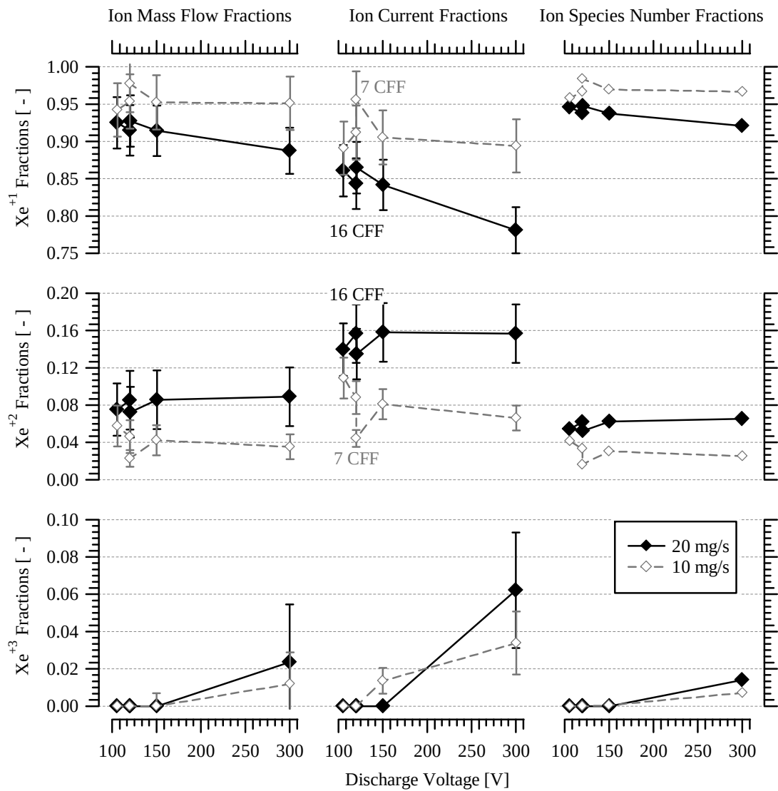
Figure 5-23 Ion mass flow fractions (left), ion current fractions (middle), and ion species number fractions (right) of \text{Xe}^{+1} , \text{Xe}^{+2} , and \text{Xe}^{+3} from ExB measurements of ion energy distribution on channel centerline 1 meter downstream of the exit plane for 105 V to 300 V discharge at 10 mg/s and 20 mg/s anode flow rate. Labels for increased CFF at 120 V operation are listed on ion current fractions, and may be used to determine the operating condition on traces of ion mass flow fractions and ion species number fractions.
