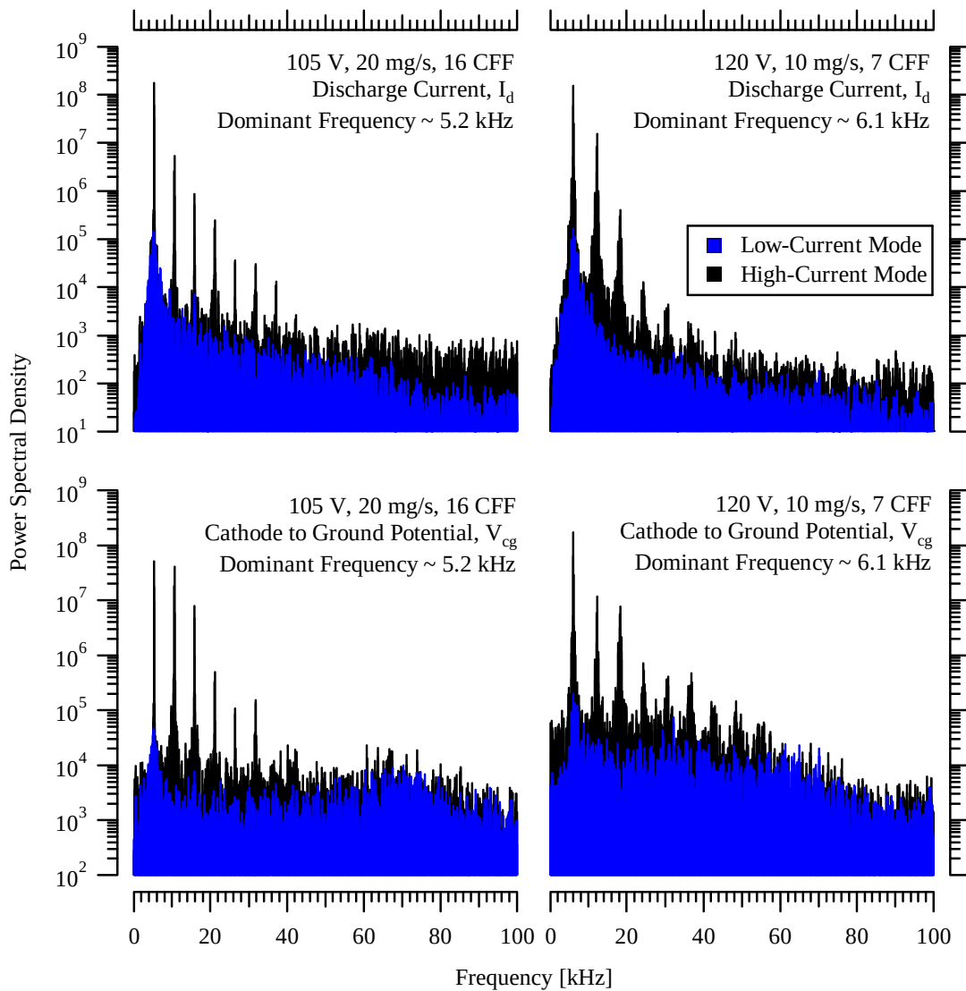
Figure 6-6 Comparison of discharge current oscillation spectra (top) and cathode to ground potential oscillation spectra (bottom) in the low-current and high-current modes for 105 V, 20 mg/s, 16 CFF operation (left) and 120 V, 10 mg/s, 7 CFF operation (right) from 0 to 100 kHz.
