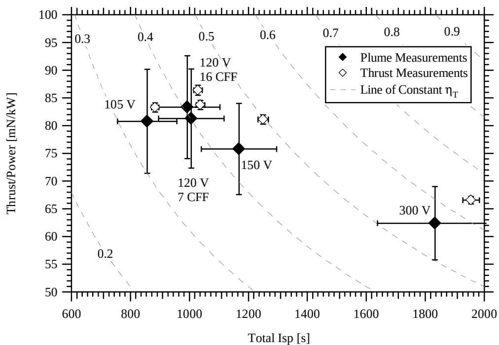
Figure 5-25 Comparison of thrust to power ratio, total specific impulse, and total thruster efficiency calculated with plume properties and thrust measurements for 105 V to 300 V discharge at 20 mg/s anode flow rate.
