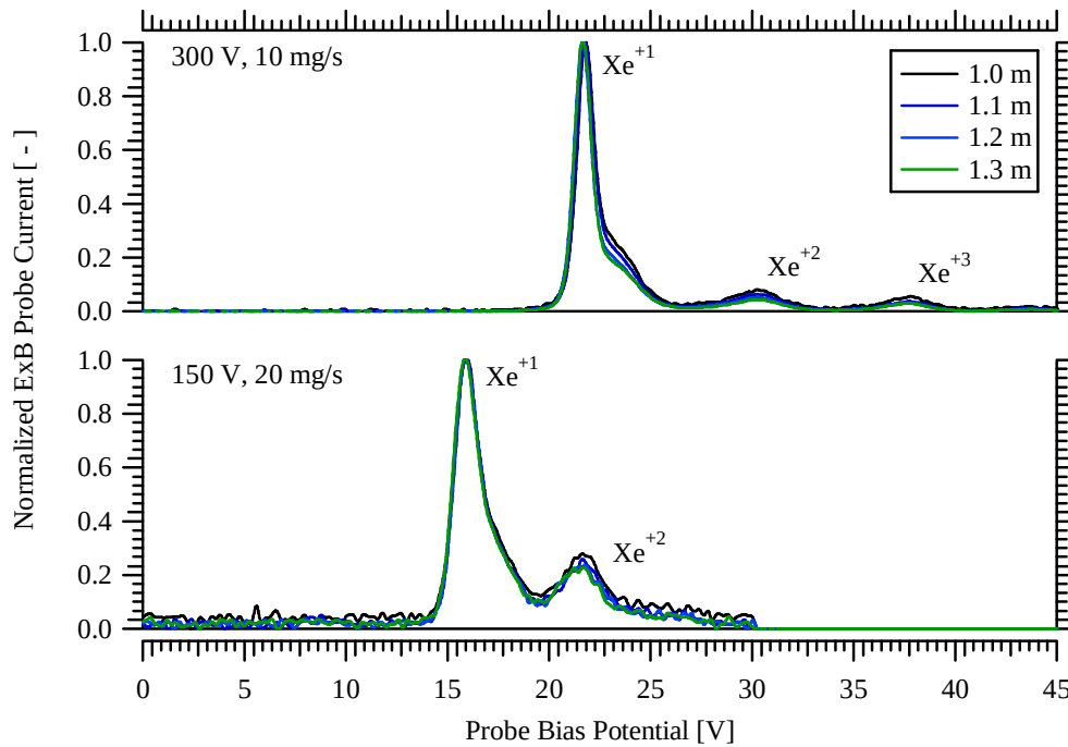
Figure 3-21 Normalized ExB probe traces on thruster centerline from 1.0 to 1.3 meters downstream of the 6 kW HET operating at 300 V, 10 mg/s and 150 V, 20 mg/s in Chamber 3.
