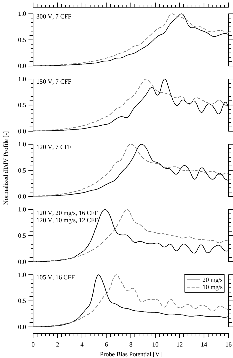
Figure 5-20 Langmuir probe traces of dI/dV on thruster centerline located 1-m downstream of the exit plane for 105 V to 300 V discharge at 10 mg/s and 20 mg/s anode flow rate.
