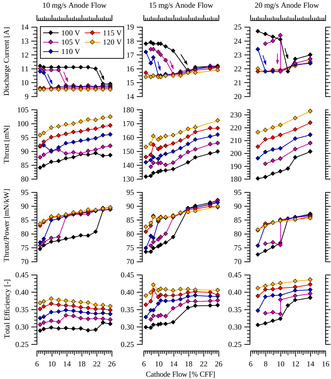
Figure 6-2 Mapping of anode and cathode thruster operating characteristics at 100, 105, 110, 115, and 120 V discharge. Discharge current, thrust, T/P, and total thruster efficiency are shown for lines of constant discharge voltage as a function of cathode flow fraction during 10 mg/s (left column), 15 m/gs (middle column), and 20 m/gs (right column) anode mass flow rate operation. Operating characteristics are reported for facility background pressure in the range of 0.8 \times 10^{-5} to 1.2 \times 10^{-5} Torr. Transitions from the operation in low-current to high-current mode are shown with arrows.
