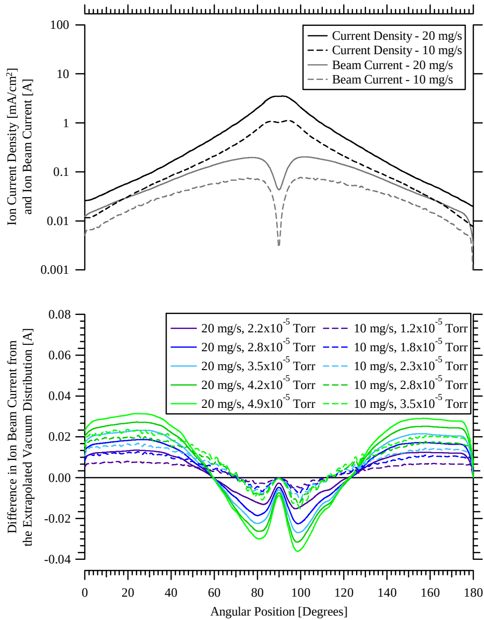
Figure 5-5 Angular distributions of ion beam current extrapolated to vacuum and the angular difference in ion beam current with increasing background pressure for 105 V, 16 CFF at 10 and 20 mg/s anode flow rate.
