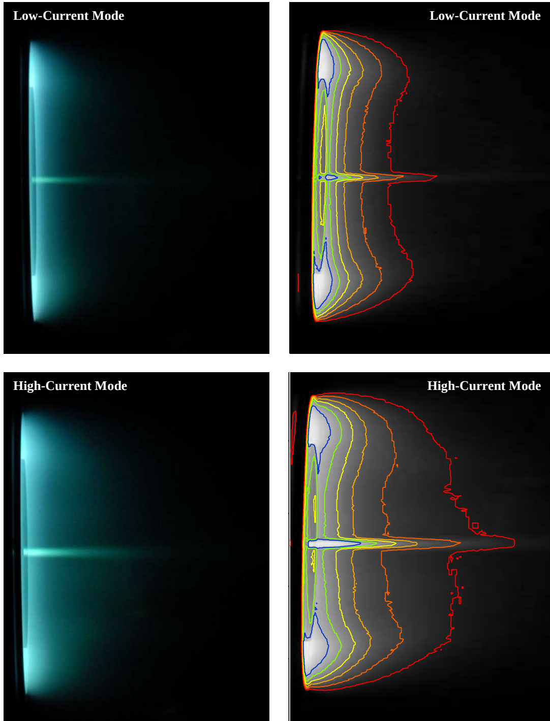
Figure 6-1 Photographs of the 6 kW Hall thruster jet-mode plume structure for the low-current mode (top left) and high- current mode (bottom left) during 105 V, 20 mg/s operation. Contours of constant image intensity are shown for the low-current mode (top right) and the high-current mode (bottom right). Photos were taken with identical settings on a tripod mounted Nikon D200 DSLR using a 70 mm lens with manual focus at F/5, ISO-400, and exposure time of 1/2000 sec.
