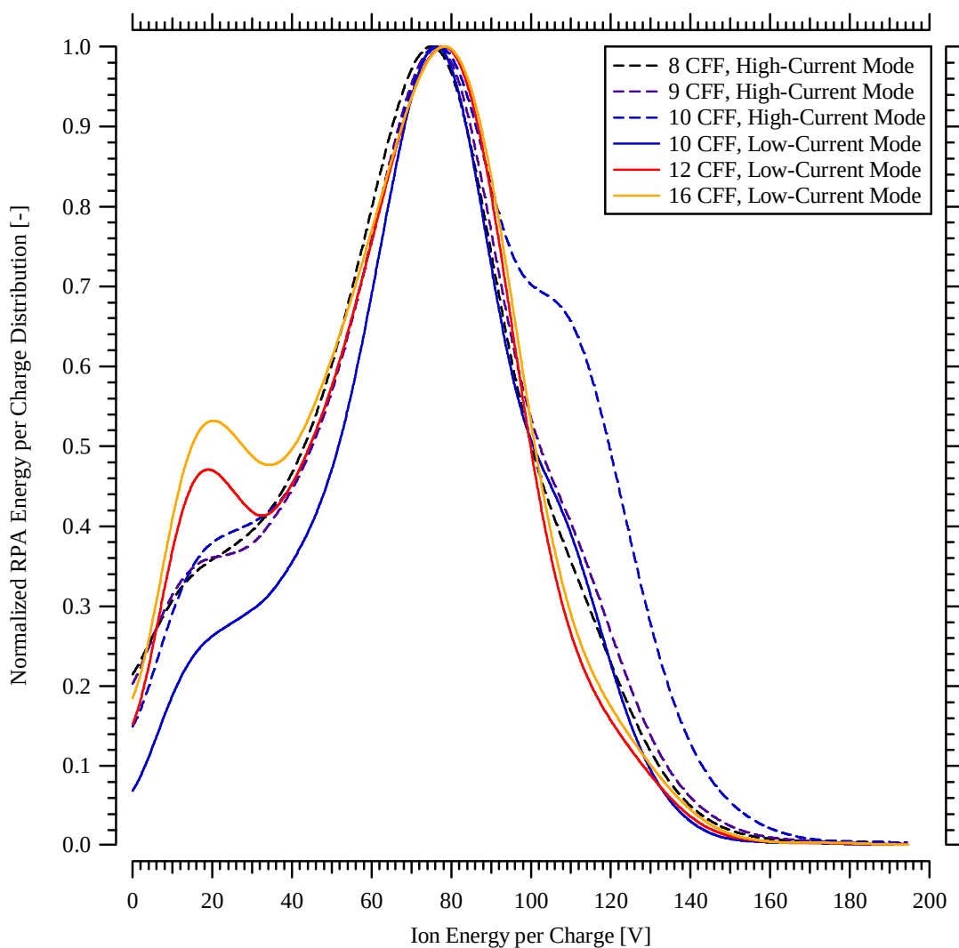
Figure 6-13 Normalized RPA ion energy per charge distributions on thruster centerline located 1-m downstream of the exit plane for 105 V, 20 mg/s operation with cathode flow fraction ranging from 8 CFF to 16 CFF. The ion energy per charge has been corrected for local plasma potential at the probe.
