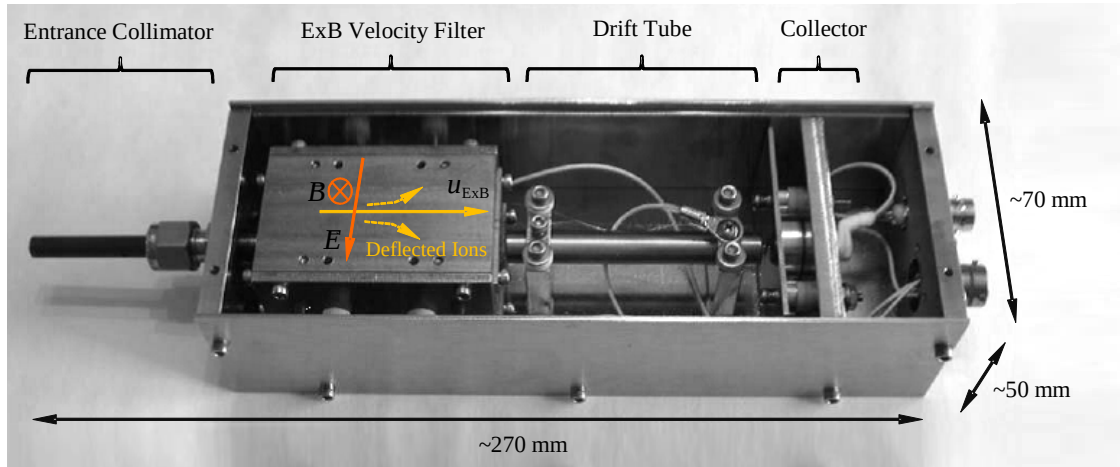
Figure 3-18 Photograph of the ExB probe build by Plasma Controls, LLC. The top cover is removed to illustrate the electromagnetic fields in ion velocity filter and regions of ion collimation, drift, and collection.
