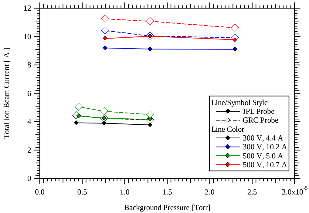
Figure 4-23 Total ion beam current of the NASA173M-v1 as a function of background pressure for the JPL and GRC nude Faraday probes from Walker et al. 117
