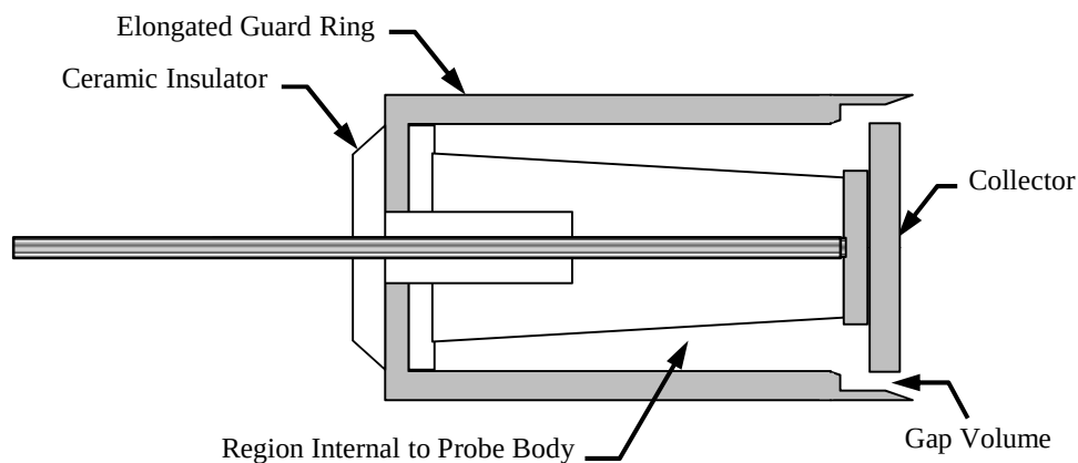
Figure 4-21 Diagram of the JPL nude Faraday probe.
