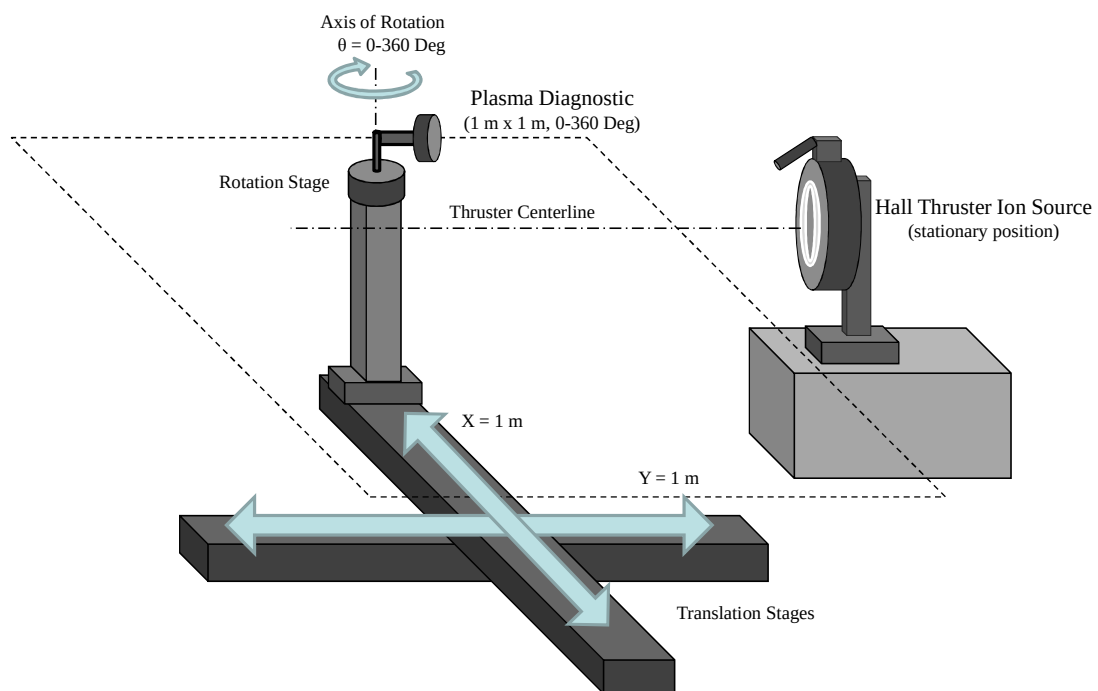
Figure 3-8 Diagnostic positioning system in Chamber 3 with X,Y, \theta -coordinate axis control.
