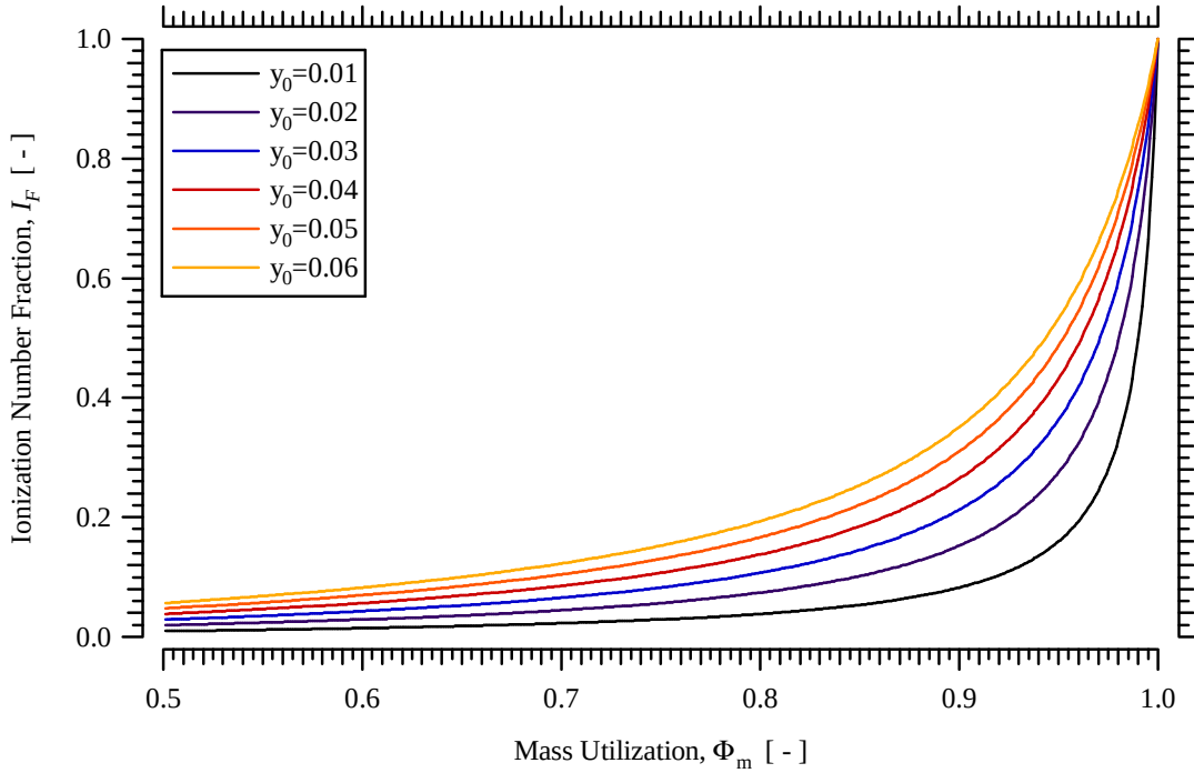
Figure 2-1 Ionization number fraction as a function of mass utilization with lines of constant neutral velocity ratio, y_0 , for a singly-charged plasma ( Q=1 ).
