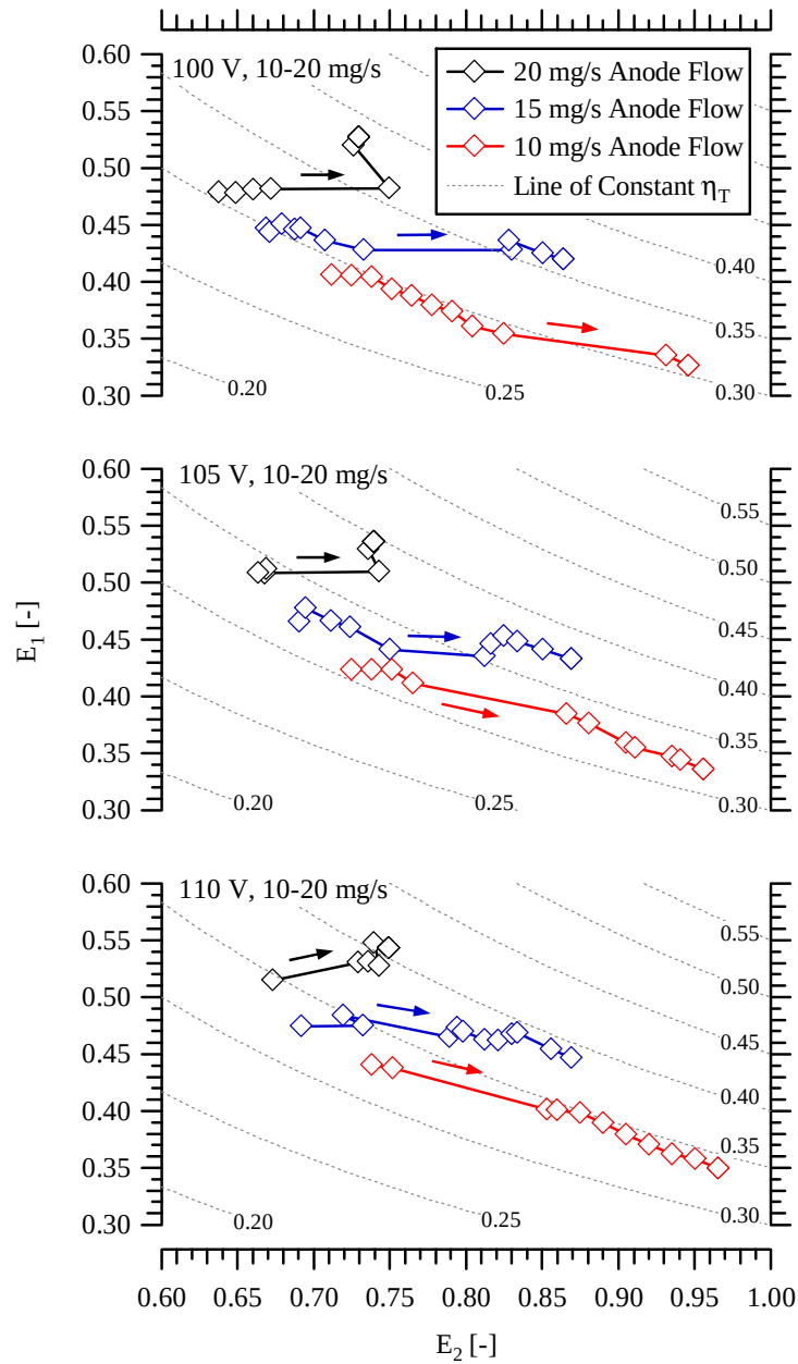
Figure 6-3 Voltage exchange parameter and mass exchange parameter at 100 V (top), 105 V (middle), and 110 V (bottom) thruster operation for lines of increasing cathode flow during 10, 15, and 20 mg/s anode flow. Operating characteristics are reported for facility background pressure in the range of 0.8 \times 10^{-5} to 1.2 \times 10^{-5} Torr. Transitions from the operation in high-current to low-current mode are shown with arrows, indicating the direction of increasing cathode flow fraction.
