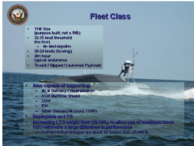
Figure 35 - Fleet Class USV
