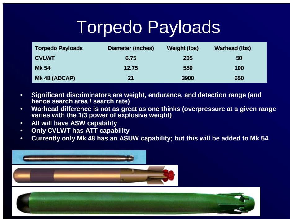
Figure 18 – Example Torpedo Payloads for ASW Mission
