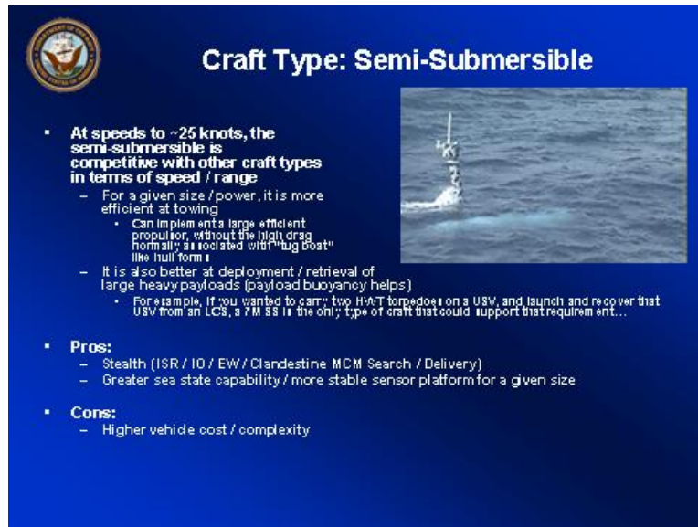
Figure 27 – Semi-Submersible Hull Type
