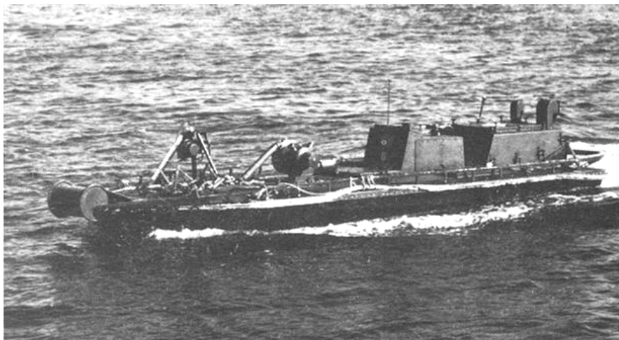
Figure 3 - Minesweeping Drone (MSD)
