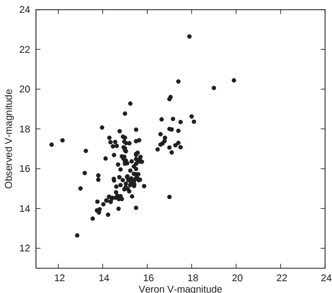
Figure 5. Plot of observed V magnitudes vs. Veron catalog V magnitudes.
