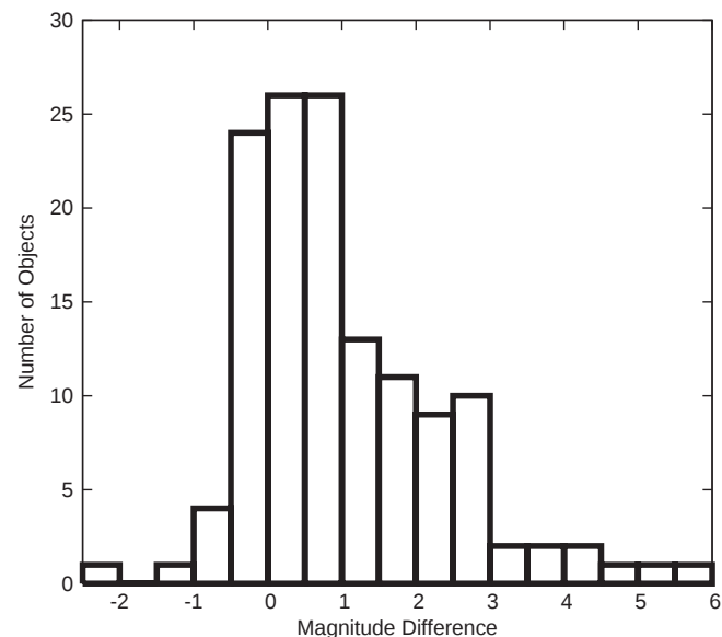
Figure 7. Histogram of magnitude differences between observed V magnitudes and Veron catalog V magnitudes. A positive difference indicates a larger observed V magnitude (fainter) as compared to the Veron value.
