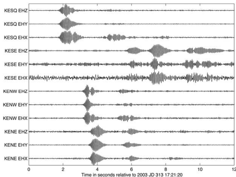
Figure 2. Examples of a fin whale vocalization recorded on four three-component seismometers (the labels EHZ, EHY and EHX indicated the vertical (Z) and horizontal channels (X and Y) of stations KESQ, KESE, KENW and KENE). The records have been adjusted to equal maximum amplitude. The fin whale was located near the network. Note that the 1 st and 2 nd water column multiples are clearly visible following the direct arrival.
