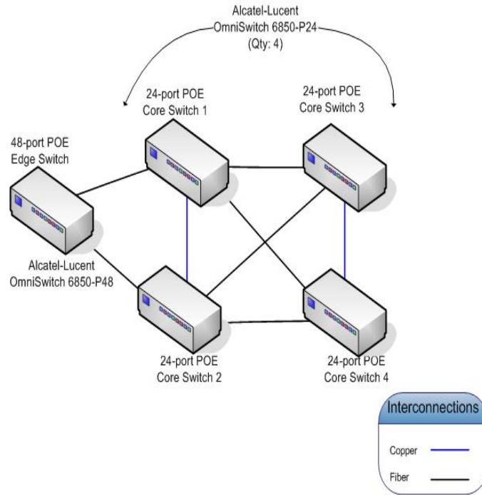
Figure 4-1 Switch Layout
