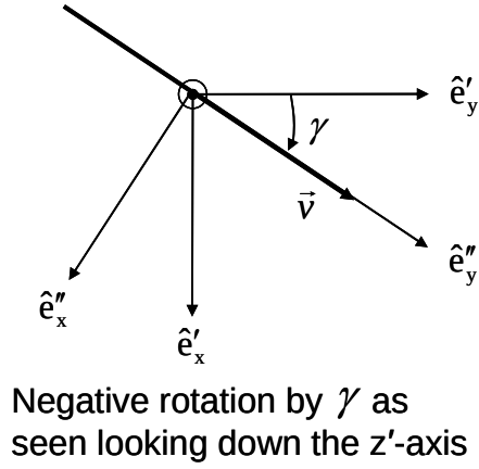
Figure 3-5: Rotation of the OX'Y'Z' System About the z' -axis
