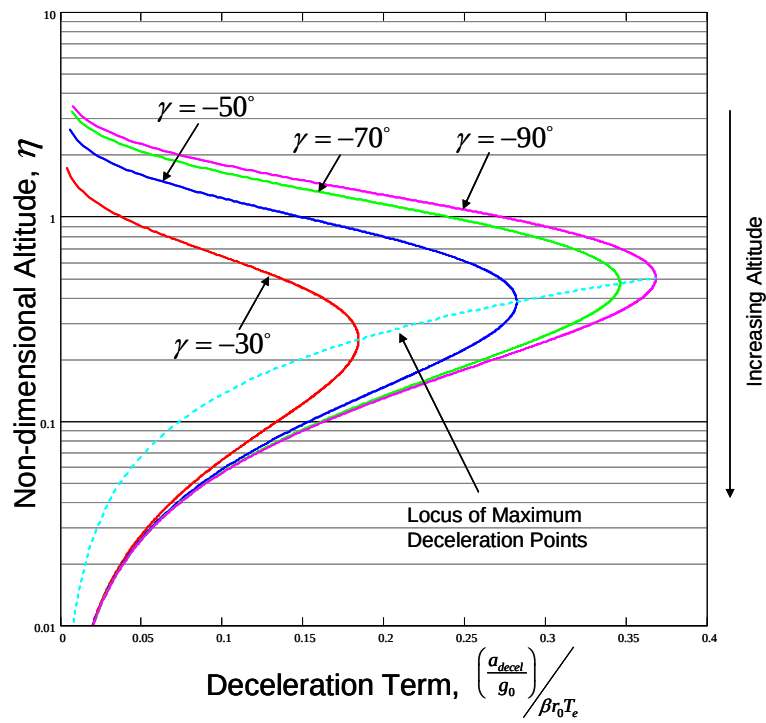
Figure 5-21: Deceleration During Steep Ballistic Entry (Ignoring Gravity)
