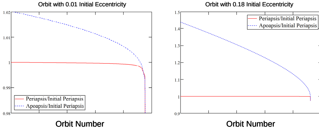
Figure 11-6: Circularization of Two Orbits
