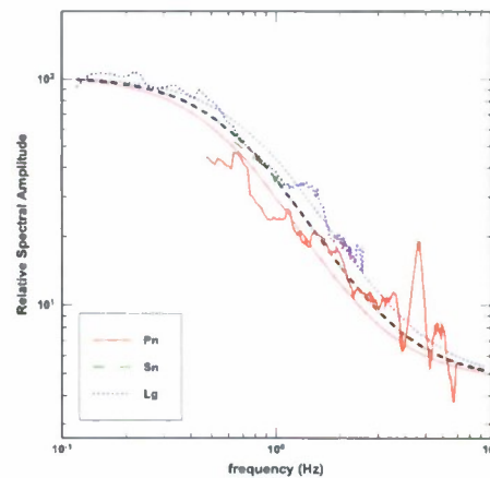
Figure 3. Example of relative spectra for a pair of M_w 6.0 and 4.7 earthquakes. Model fits are shown for each phase and using all phases (black dashed).
