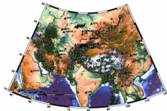
Figure 6. Events and stations used to process relative spectra and fit corner frequencies and estimate stress drop. The cluster highlighted in red and the path along two clusters to MAKZ are discussed below.
