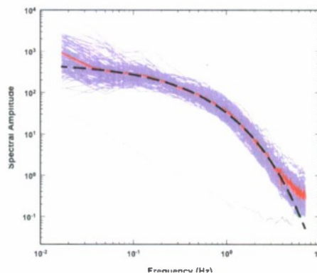
Figure 9. Lg spectra at BRVK, corrected for response and source terms, for all events in the cluster (blue), the median (red), and a model fit of the combined distance and site effects (black dashed).
