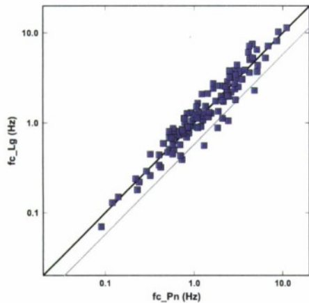
Figure 4. Estimated Lg versus Pn corner frequencies, indicating similar values for most of the earthquakes. Black and gray lines represent ratios of 1.0 and 1.73.
