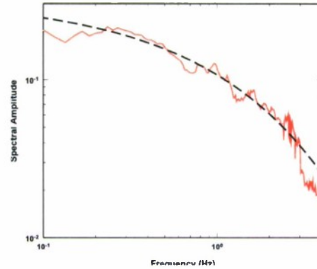
Figure 17. Ratio of source-corrected median spectra at MAKZ for two clusters along the great-circle path in Figure 6. The relative spectrum factors out the site term and allows a robust estimate of Q for this path.
