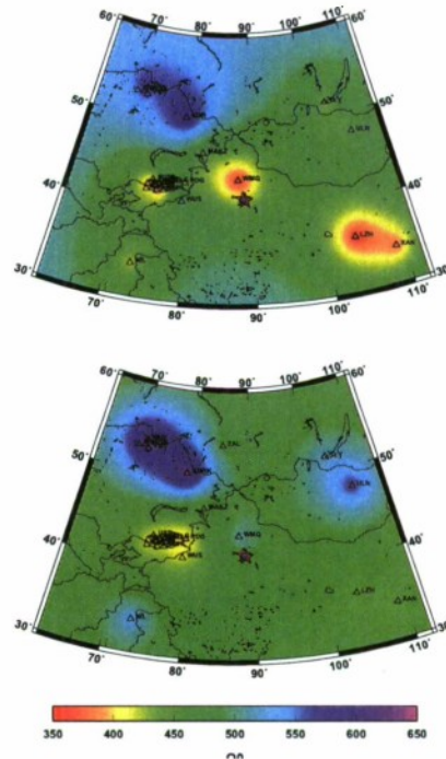
Figure 12. Interpolated grids of effective Lg Q_0 for paths from LNTS to regional stations from our analysis (top) and based on Q tomography (bottom).
