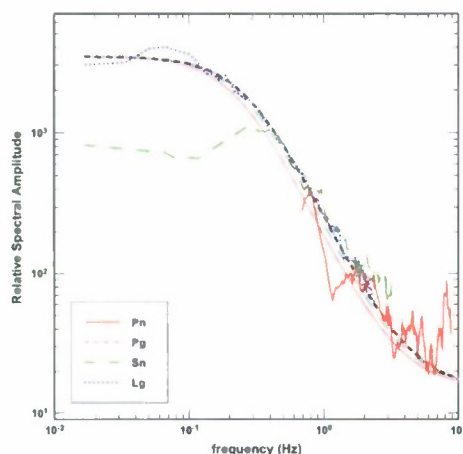
Figure 7. Network-median relative spectra of Pn, Sn, and Lg and model fits (smooth curves) for an event pair in the highlighted cluster in Figure 6.
