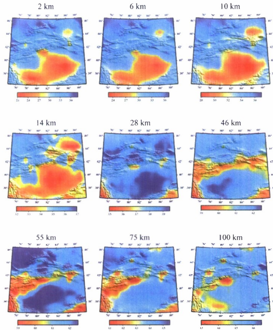
Figure 3. S-wave velocity model at constant depth slices. The depth of each image is shown at the top of each map. Velocity values are expressed in km/s. Note the color scheme is different for each image. The high wavenumber features at depth are clearly artifacts of the simple smoothing scheme used in the current inversion algorithm – none of the data (long-period surface wave dispersion or gravity) can constrain such sharp features at those depths.
