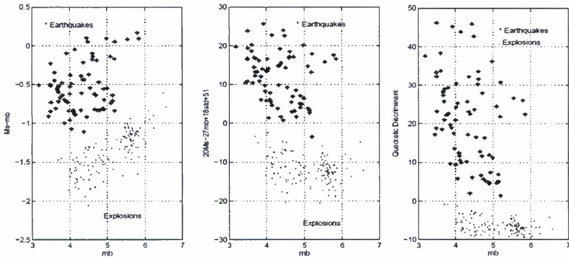
Figure 9. Conventional multivariate discriminant analysis combining M_s(\text{VMAX})-m_b (left), M_s(\text{VMAX}) , m_b and standard deviation (std) (middle), and multivariate linear-quadratic discriminant analysis (right) for 73 WUS earthquakes and 131 explosions.
