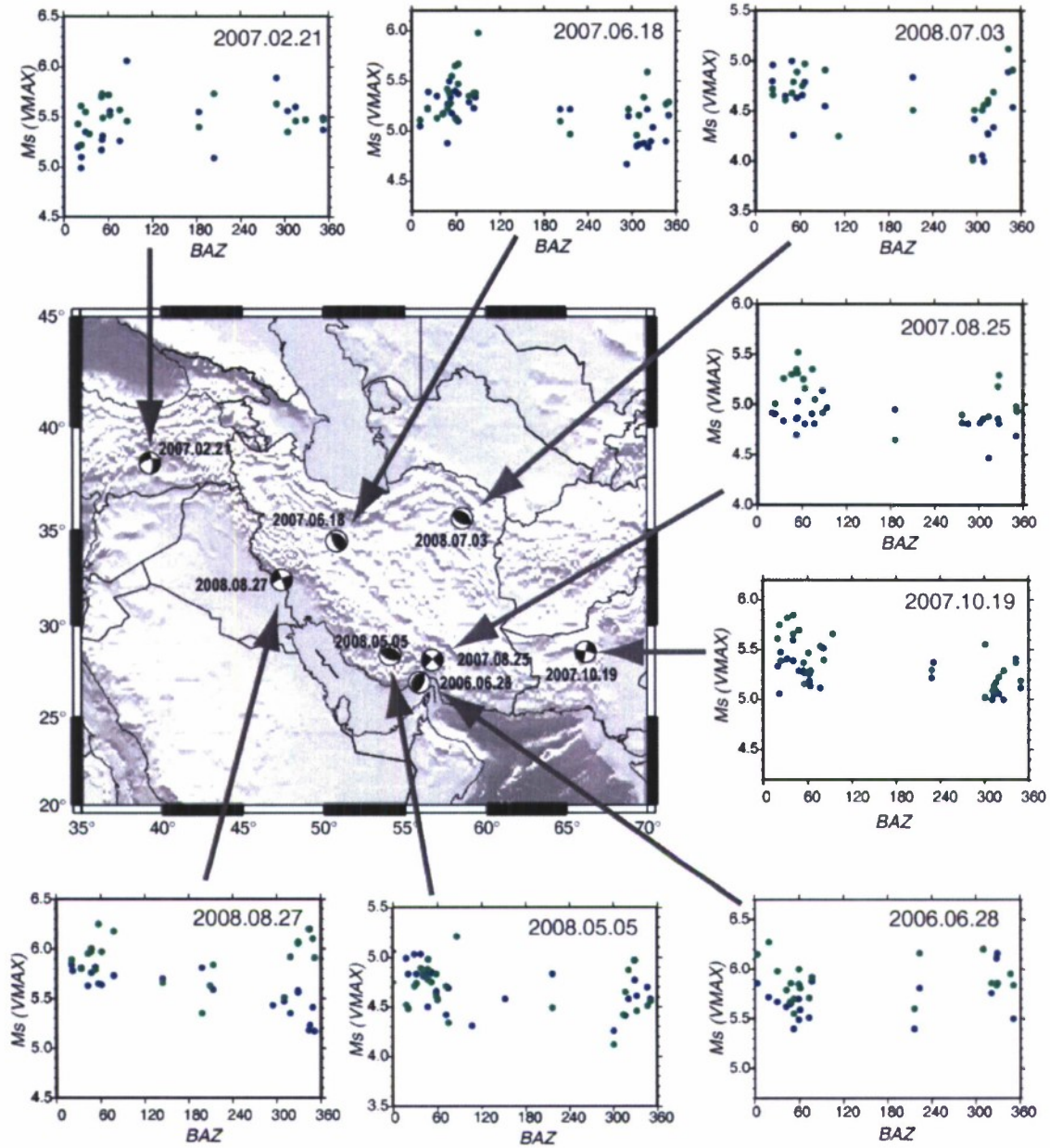
Figure 3. Azimuthal dependence of M_s(\text{VMAX}) for some events with known focal mechanisms. Blue and green circles show Rayleigh and Love M_s(\text{VMAX}) estimates, respectively.
