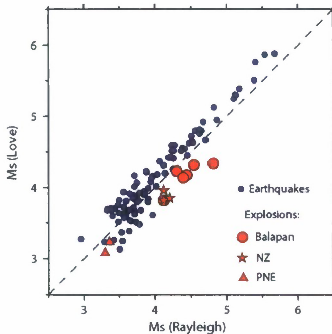
Figure 2. Comparison of M_s(\text{VMAX}) computed using Rayleigh and Love waves. Small blue circles show earthquakes, the red symbols show M_s estimate using one station (BRVK) for some Soviet nuclear explosions.
