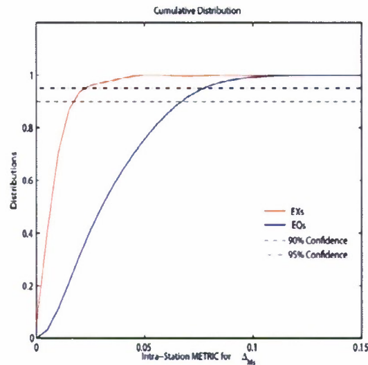
Figure 12. Cumulative distribution functions for metric M (Equation 3; Figure 11) for WUS earthquakes and NTS explosions.
