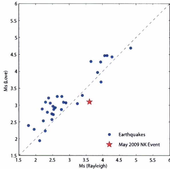
Figure 6. Comparison of M_s (VMAX) computed using Rayleigh and Love waves for the Korean Peninsula region. Small circles show earthquakes while the star shows the M_s estimate for the 25 May 2009 announced nuclear test.
