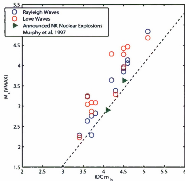
Figure 7. Comparison of network M_s (VMAX) estimates for Rayleigh- and Love-waves versus International Data Centre (IDC) body wave magnitude m_b for Korean Peninsula earthquakes and the two announced North Korean nuclear explosions. The dashed line represents the event screening line proposed by Murphy et al. (1997).
