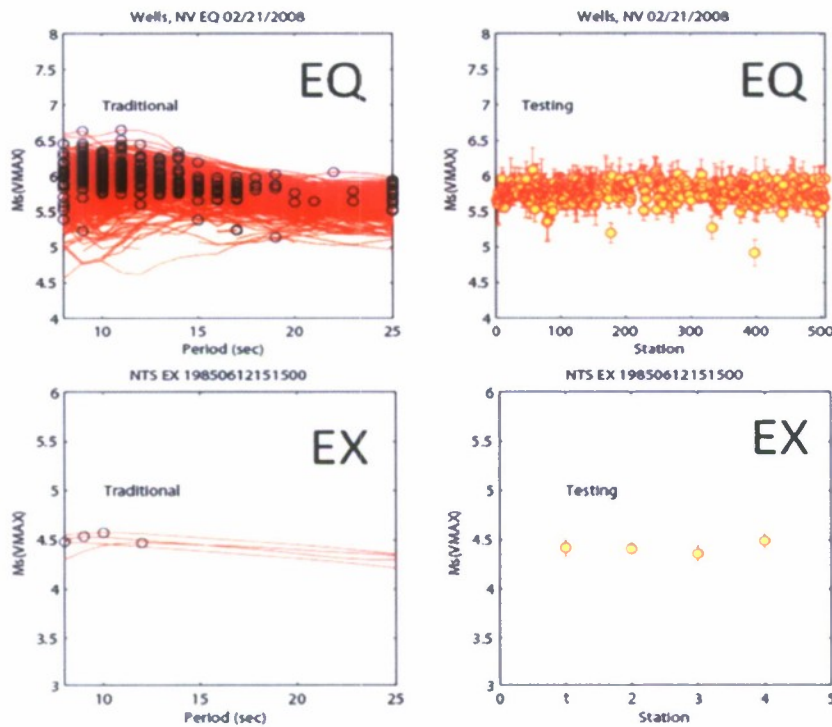
Figure 10. A proposed new approach for improved discrimination. (Left Column) Traditional M_s(VMAX) where the circle is the period of maximum amplitude. (Right Column) The mean of a station's estimate and its standard deviation are formed. Our results suggest that the intrastation standard deviation is typically less for explosions than earthquakes for our WUS database.
