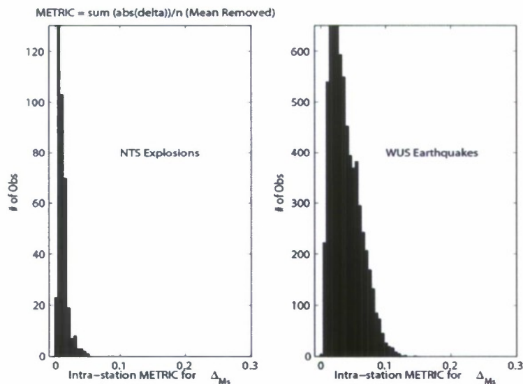
Figure 11. Comparison of the new intrastation metric \Delta_{Ms} for NTS explosions (left) and WUS earthquakes (right).
