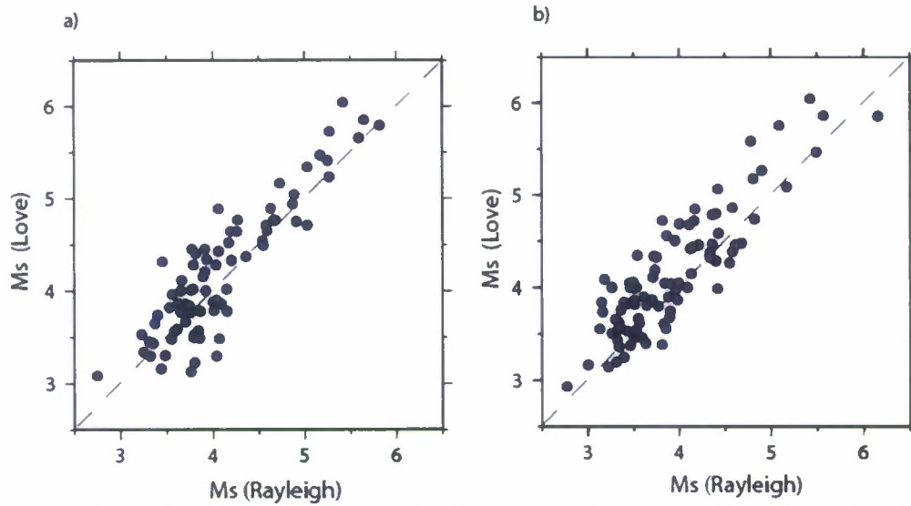
Figure 4. Comparison of M_s(\text{VMAX}) computed using Rayleigh and Love waves for individual stations: a) stations located to the NE from the events (back azimuth ranges between 20^\circ and 70^\circ ); b) stations located to the NW (back-azimuth ranges between 270^\circ and 360^\circ ).
