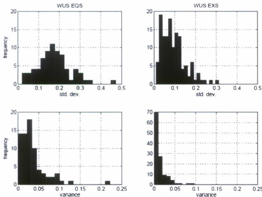
Figure 8. Frequency histograms for the station standard deviations (top) and variances (bottom) for 73 WUS earthquakes and 131 explosions.
