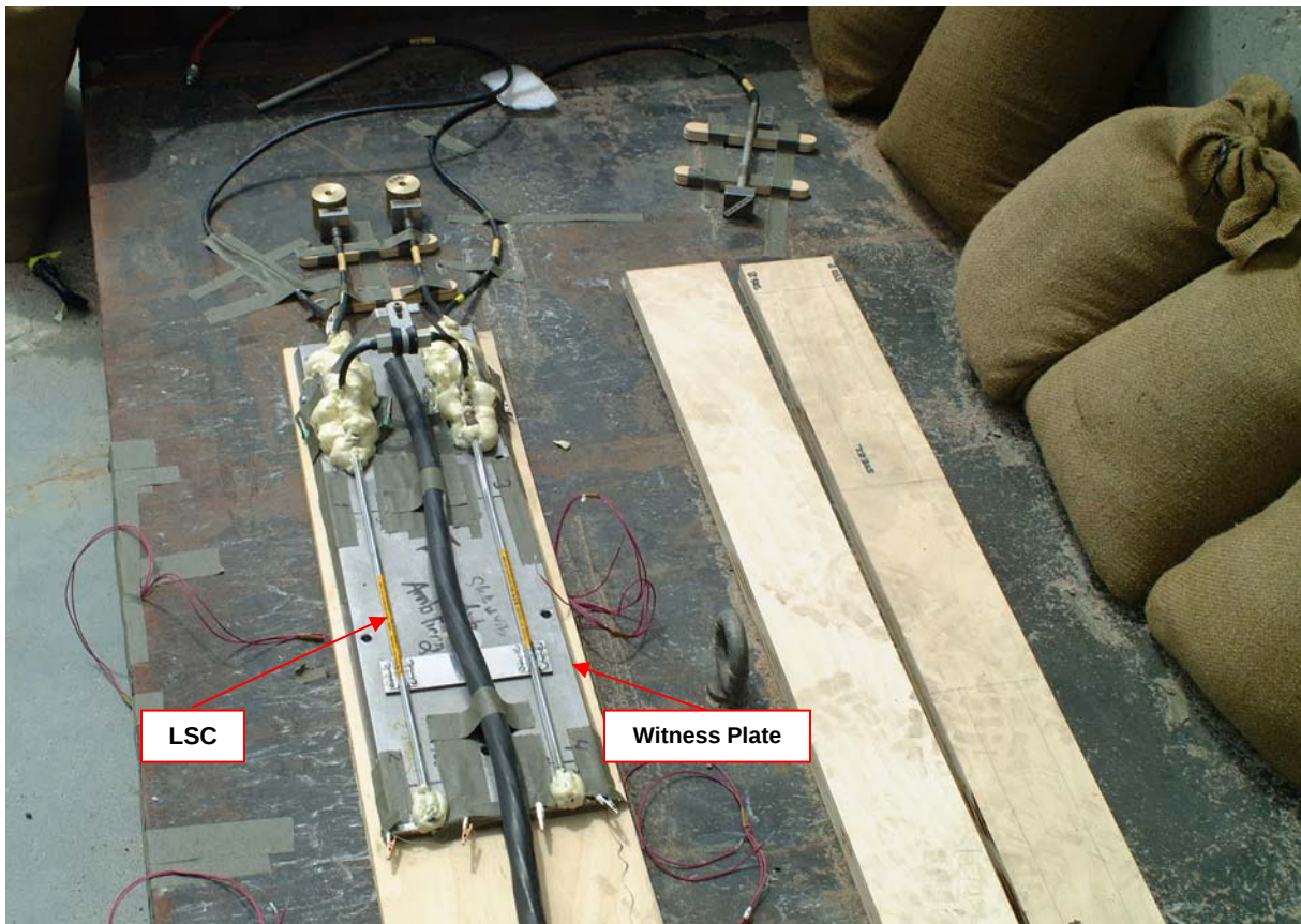
Figure 6. LSC Pre- Function Test Setup
