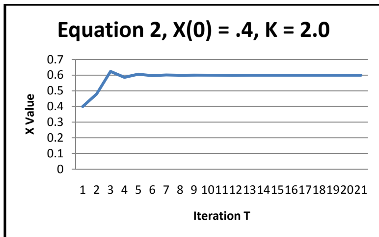
Figure 6: The Logistics Equation: The Move to Chaos through Period Doubling, K=2.0
