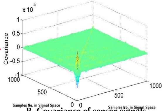
B. Covariance of sensor signals at a typical time instance
