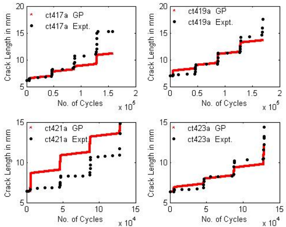
Figure 14B. Continuous crack growth estimation based on KPCA features
