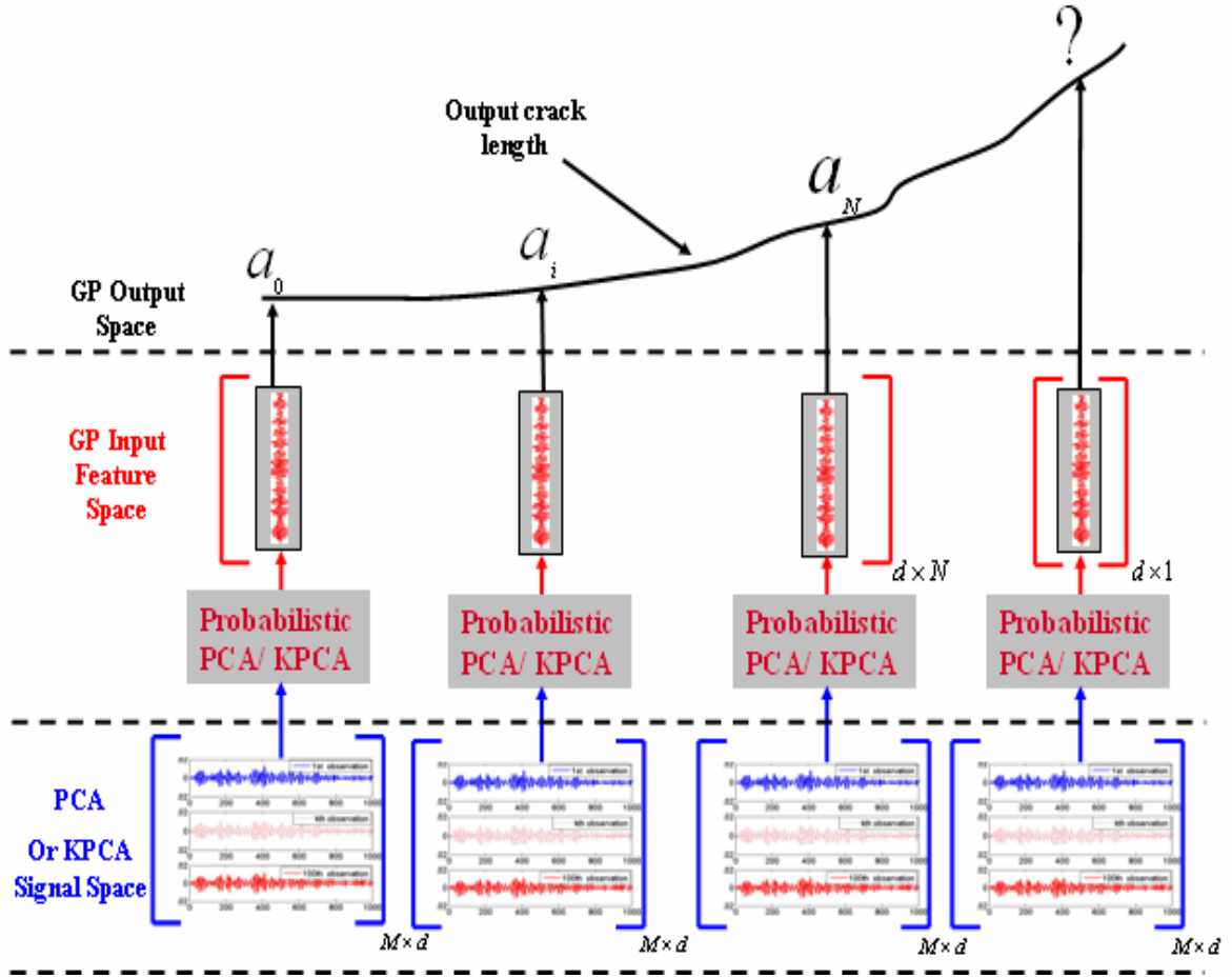
Figure 3. General architecture for on-line predictive model
