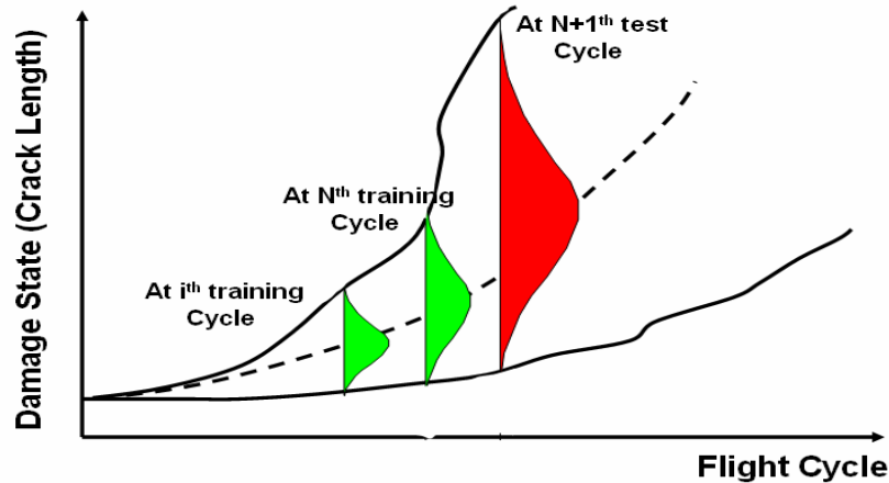
Figure 2. Gaussian process combines individual distributions at various instances of time.
