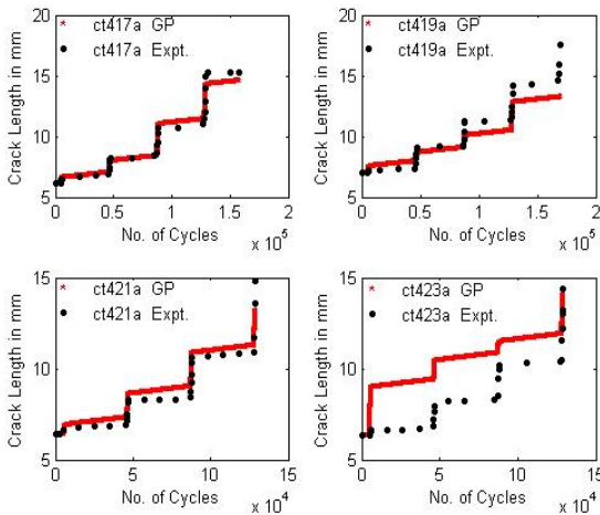
Figure 14A. Continuous crack growth estimation based on PCA features
