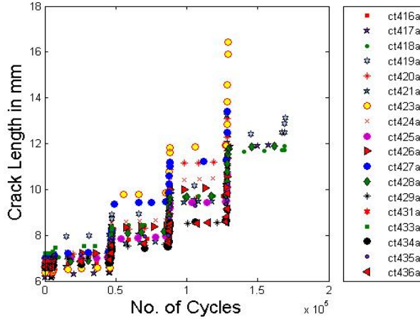
Figure 9B. Discrete crack lengths (at experimental stopping instances) captured from Fig.9A
