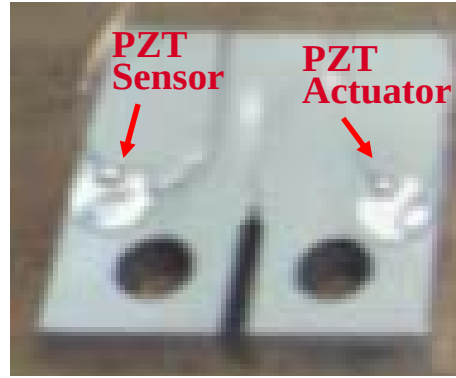
Figure 6. Instrumented CT specimen
