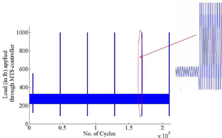
Figure 4. Loading spectrum programmed to load frame controller
