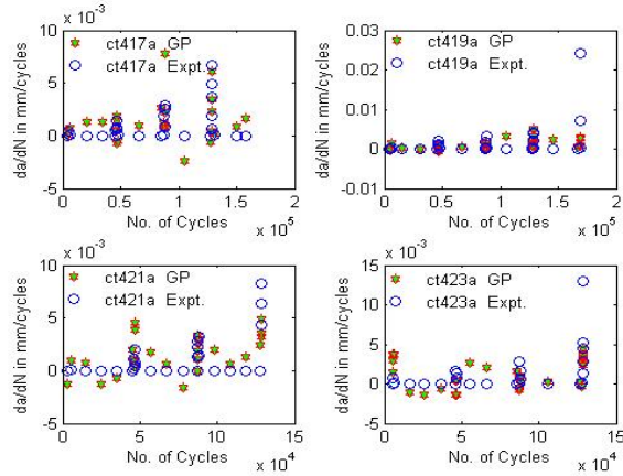
Figure 13A. Rate prediction based on PCA features
