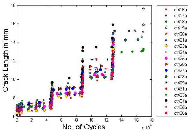
Figure 5. Experimental crack length data
