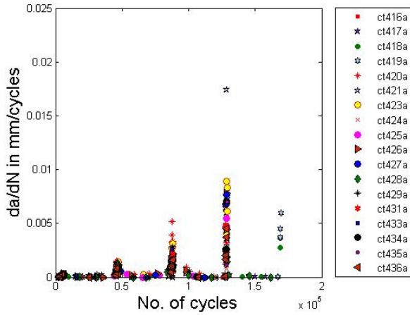
Figure 8A. Predicted rate from multivariate GP
