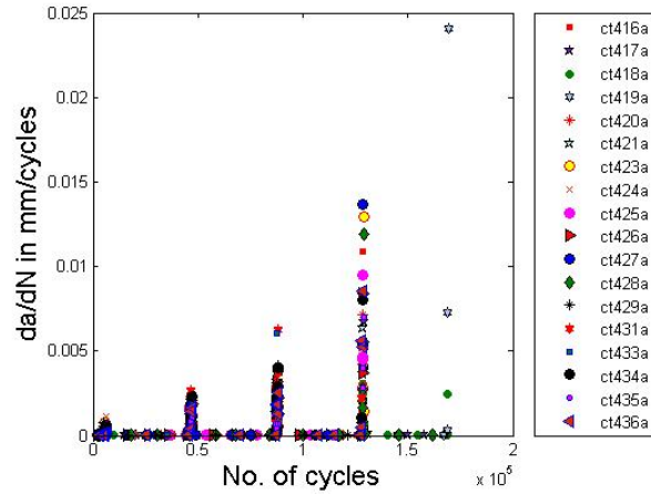
Figure 8B. Rate from experimental observation
