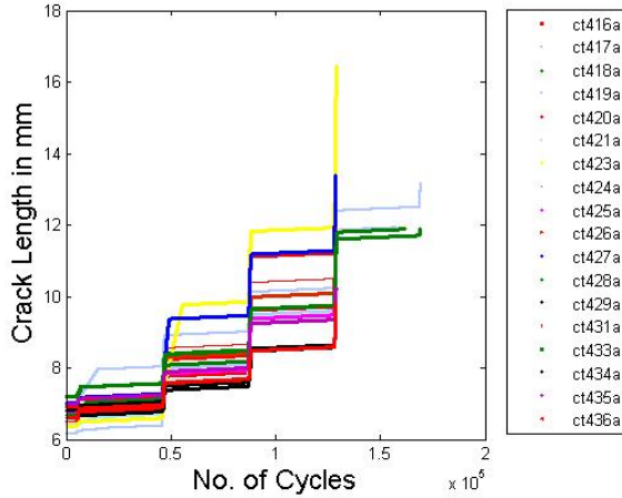
Figure 9A. Continuous crack length from integration of GP estimated rate
