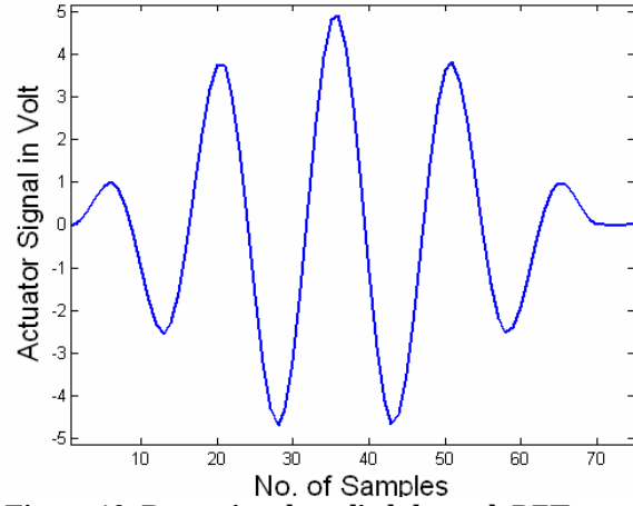
Figure 10. Burst signal applied through PZT actuator
