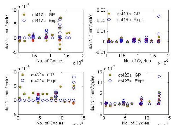
Figure 13B. Rate prediction based on KPCA features
