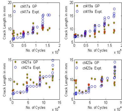
D. Predicted crack length from GP
