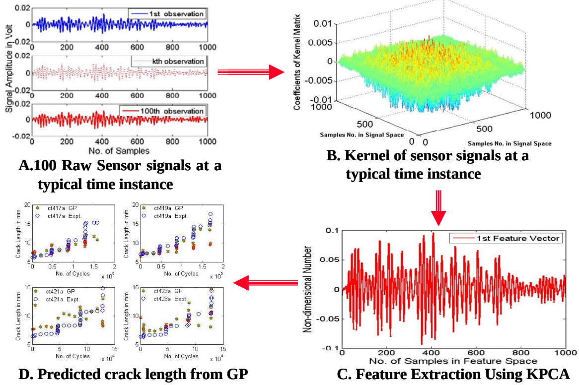
Figure 12. Hierarchical feature extraction and crack growth prediction using KPCA and GP
