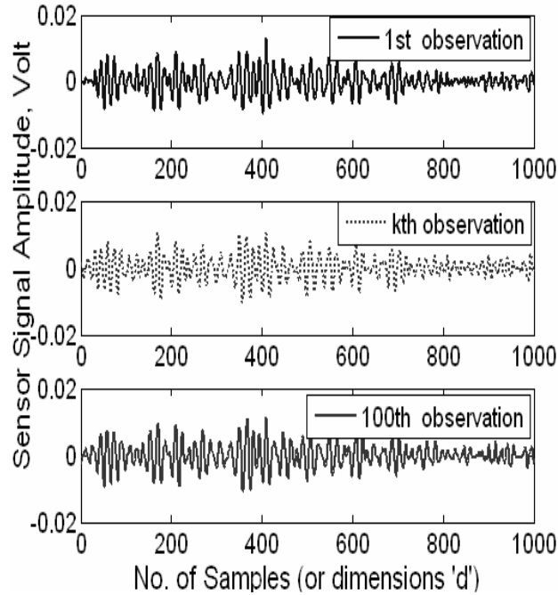
Fig. 11 Representative Sensor Signal for Feature Extraction
