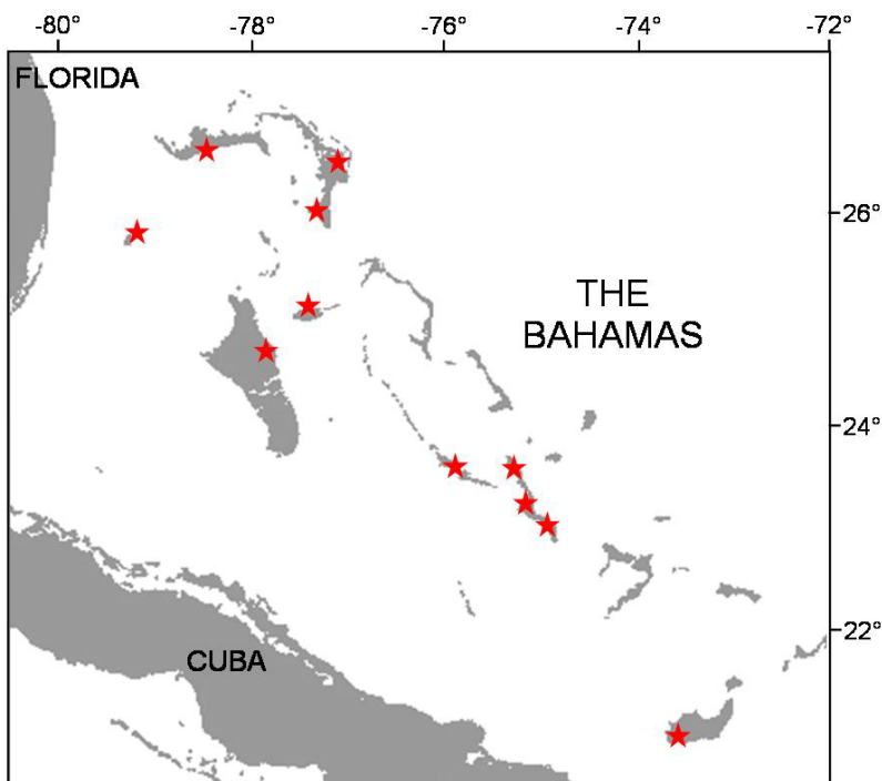
Figure 1. Map of the Bahamas showing each island that was represented at the Stranding Workshop by local participants. Each of these islands now has a large stranding kit and at least one small kit (depending on the size of the island). The map shows how the project has successfully trained individuals and distributed stranding kits throughout the island archipelago.
