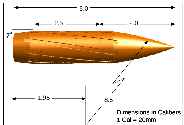
Figure 5. Geometric features of the boattailed Army-Navy spinner rocket.
