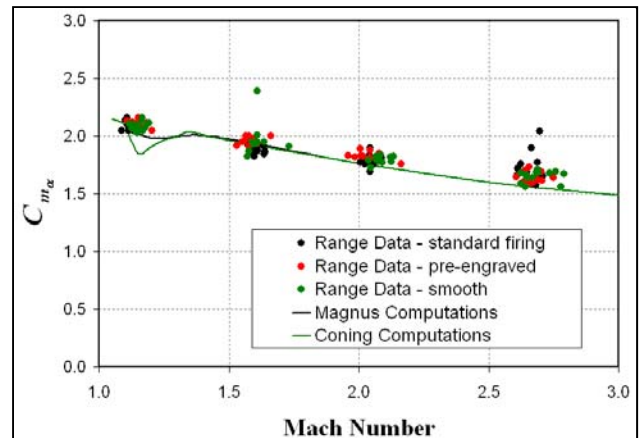
Figure 11. Pitching moment coefficient slope versus Mach number, M193.
