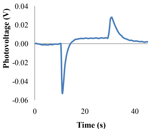
Fig. 7. Photoelectric response of a 12 bilayer bR/PDAC I-SAM film excited by a 50mW incident halogen light source. AC-coupled measurement mode.
