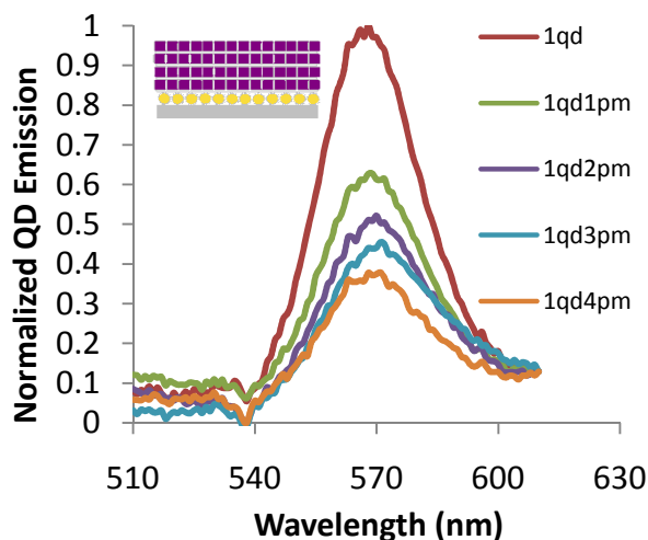
Fig. 8. QD fluorescence reduction with respect to added PM layers. The first PM layer resulted in a 39% reduction in QD emission intensity, while all subsequent layers induced less than 10% QD quenching.
