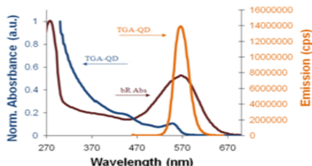
Fig. 1. Optical absorption and emission properties of size selected TGA-capped CdSe/ZnS QDs along with the absorbance spectra of bR.
