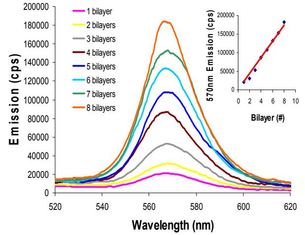
Fig 4. QD fluorescence emission for each QD/PDAC I-SAM bilayer as it is assembled. Inset displays linear trend in QD monolayer assembly.
