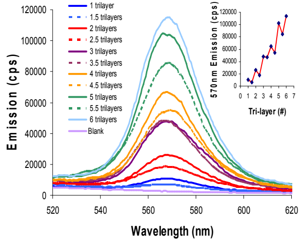
Fig 5. QD fluorescence emission for each bR/PDAC/QD I-SAM trilayer as it is assembled. Inset displays effects of bR on QD emission during tri-layer assembly.
