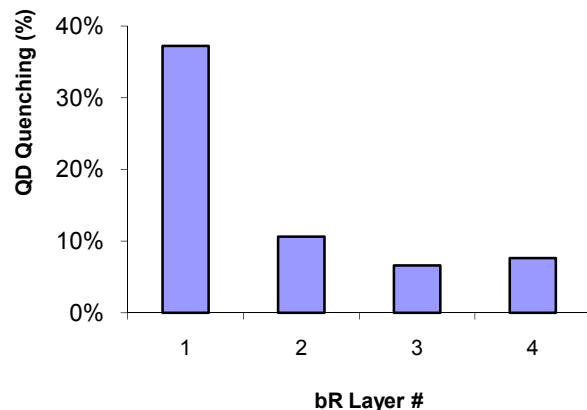
Fig. 9. Quenching effects of consecutive bR monolayers deposited on a single QD monolayer.
