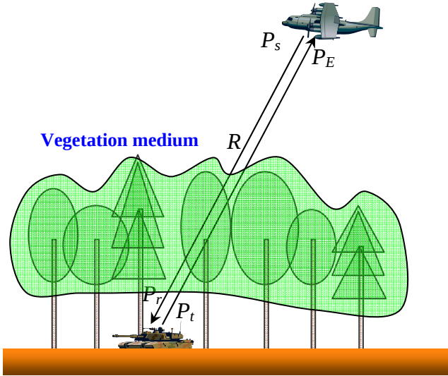
Fig. 7 A diagram showing the transmitted signal and received signal through the vegetation medium. The attenuation by the vegetation medium is approximated by SLR, and is squared due to the two-way path.
