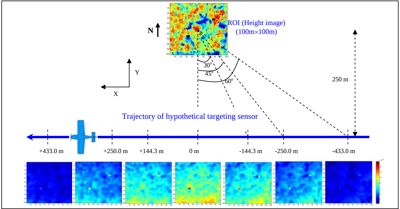
Fig. 9 A 100\text{ m} \times 100\text{ m} region of interest is shown at top depicting the above-ground tree heights (same as Fig. 5). Elevations range from zero (dark blue) to approximately 30 m (red). (Bottom row) The received power maps in watts, using (11) for a hypothetical L-band radar sensor flying at 500 m AGL, with the same targets as in Fig. 8. Relative target detectability can be seen to vary with both the targeting sensor location and local clutter.
