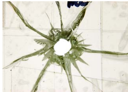
Figure 2. Brittle Failure observed from the impact of blunt nosed 17-gr. RCC.
