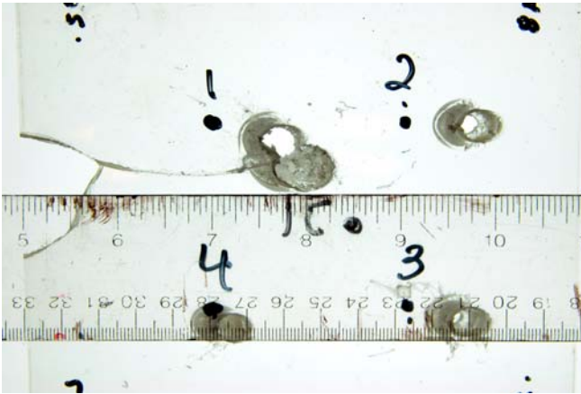
Figure 10. Ductile failure observed on 45° obliquity angle impact of 64-grain RCC.
