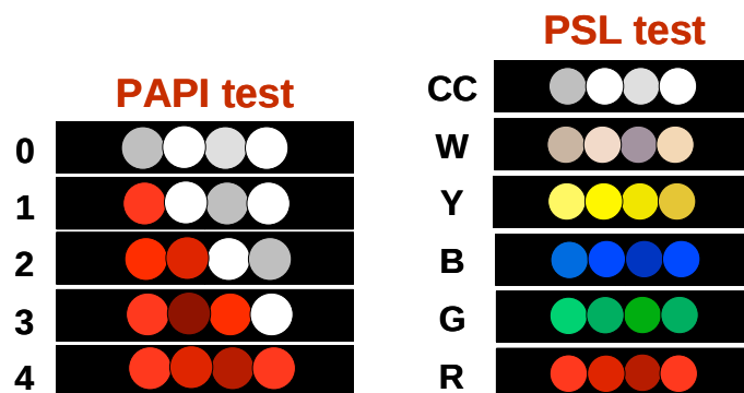
Figure 18: Schematic representation of the Precision Approach Path Indicator (PAPI) simulator test (left) and PAPI Signal Lights (PSL) test (right). The PAPI test presents 5 different conditions (as shown) twelve times giving a total of 60 presentations. The PSL presents 6 different conditions (as shown) twelve times giving a total of 72 presentations. The intensities of the colored lights varied randomly by \pm 0.3 OD with respect to the nominal values to eliminate the detection of brightness cues.
