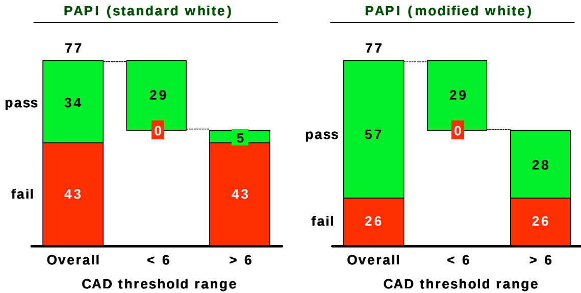
Figure 27: Summary of deutan subjects' results if the proposed pass/fail criterion of 6 RG CAD threshold units is accepted.
