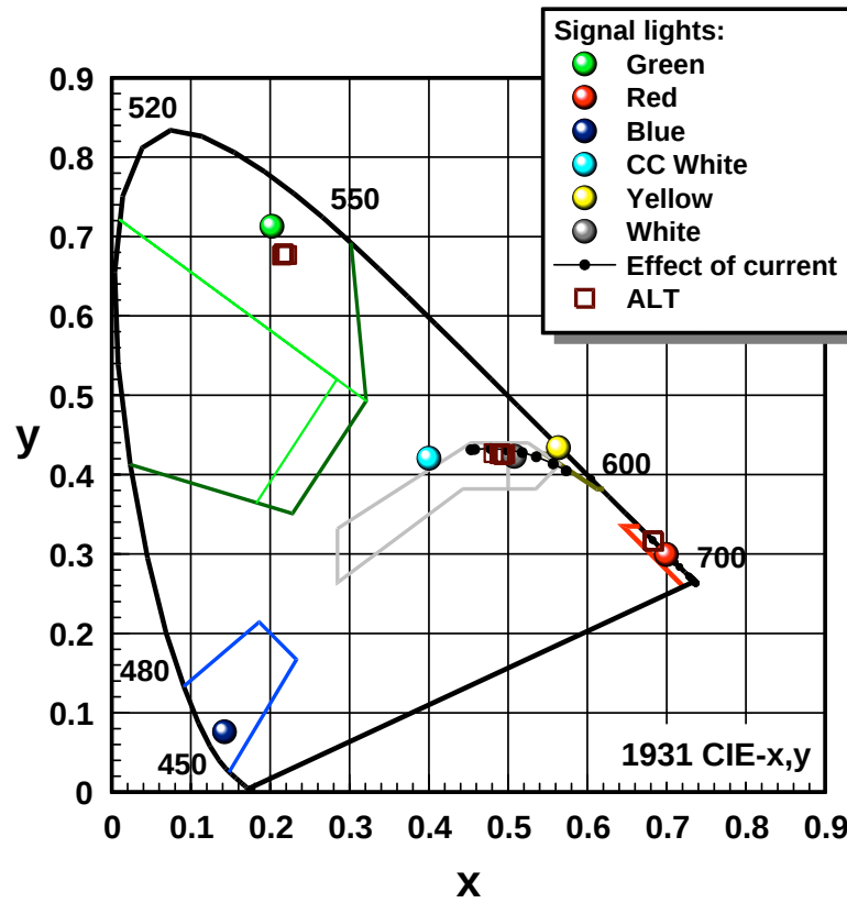
Figure 15: 1931 CIE-x,y color space diagram showing the recommended chromaticity boundaries for the colors of light signals (CIE, 2001a; CIE, 2001b). The signal colors used in the laboratory set-up are also plotted and the effect of varying the current (i.e., the output intensity of the lamps) is shown for the white light.
