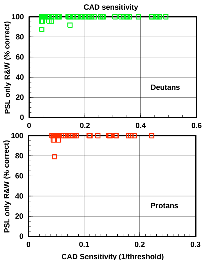
Figure 25: Graphs showing R=W and W=R errors only made on the PSL versus the RG CAD sensitivity.
