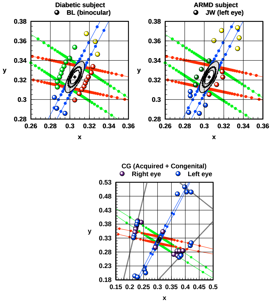
Figure 14: Examples of subjects with acquired loss of chromatic sensitivity. The data shown on the top left graph is from a subject with diabetes; top right shows data from the left eye from a subject with Age Related Macular Degeneration (ARMD); and bottom graph shows data from a subject with both congenital and acquired color vision loss (note the difference between the two eyes).
