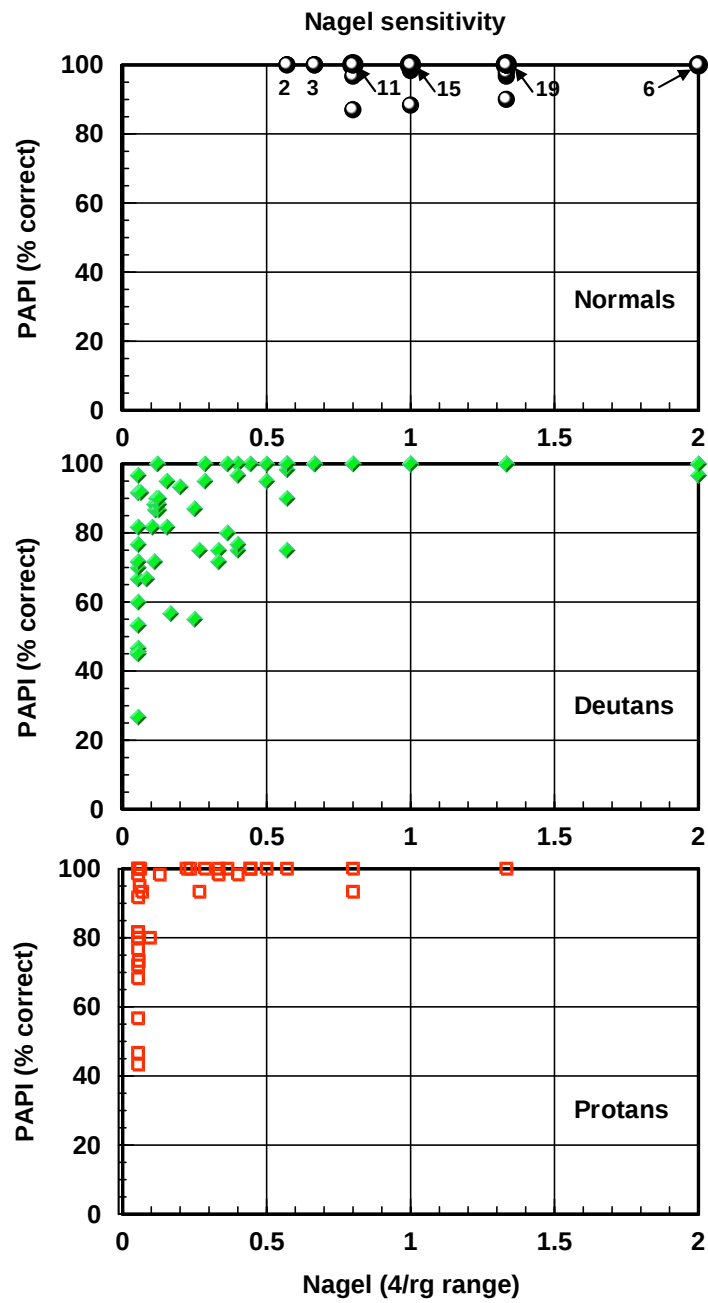
Figure 22: PAPI test scores plotted against an index of red-green chromatic sensitivity based on the Nagel anomaloscope range. Results are again shown separately for normals, deutan and protan observers. Numbers next to some symbols indicate number of subjects with overlapping data points.
