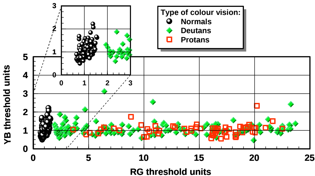
Figure 12: Graph showing Red-Green (RG) and Yellow-Blue (YB) thresholds expressed in CAD Standard Normal units for the population of subjects tested as part of this study. The spread of the data along the abscissa illustrates the large variation that exists among subjects with deutan- and protan-like deficiencies.
