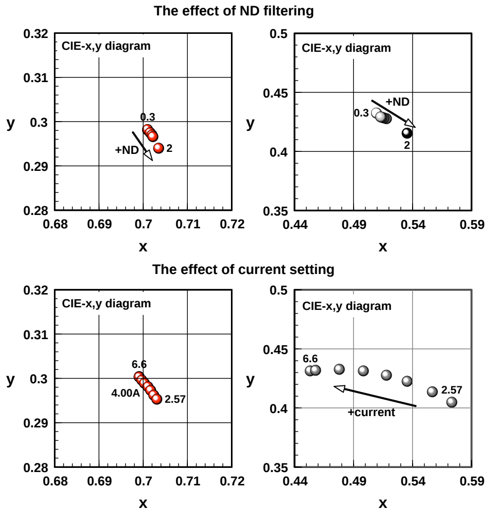
Figure 17: Graphs showing the CIE-x,y chromaticity coordinates of the Red and White lights under the effect of neutral density (ND) filtering and the effect of the current setting (intensity) on the lamp in amps (A).
