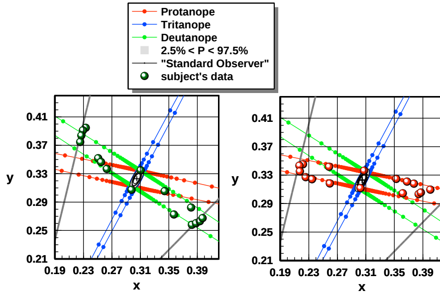
Figure 11: Chromatic thresholds for two color vision deficient observers with severe color vision deficiency. The largest chromatic displacements away from background chromaticity, as set by the isoluminant condition and the limits imposed by the phosphors of the display, are shown as grey lines. The extent of color vision loss is related to the elongation along the protanopic or the deuteranopic confusion band and suggests that the greater the elongation, the lower the level of chromatic sensitivity.
