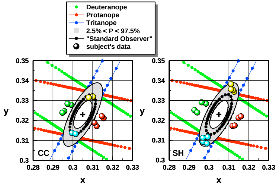
Figure 10: Chromatic thresholds for two color vision deficient observers with minimal color vision deficiency. The data for the average normal trichromat is shown as a black contour.
