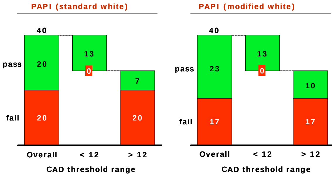
Figure 28: Summary of protan subjects' results if the proposed pass/fail criterion of 12 RG CAD threshold units is accepted.
