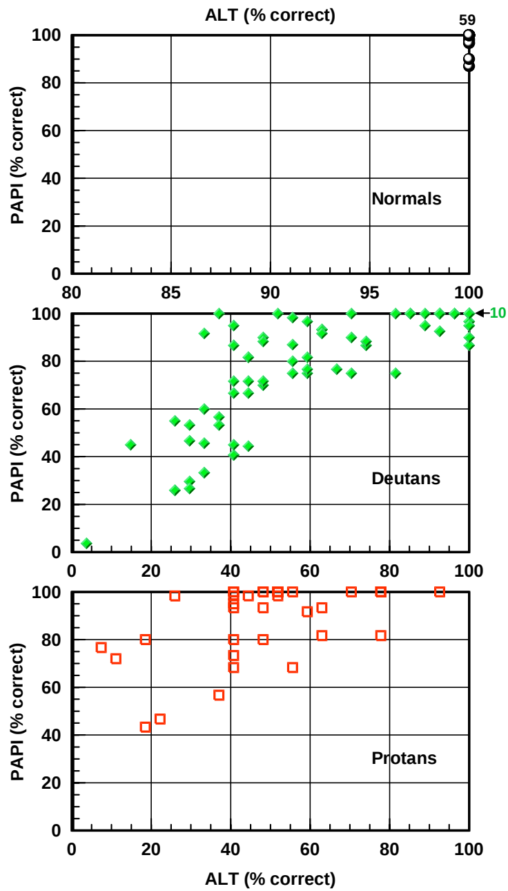
Figure 21: The number of presentations identified correctly on the Aviation Light Test (ALT) from a total of 27 presentations is compared to performance on the PAPI simulator test separately for normals, deutan and protan color vision observers.
