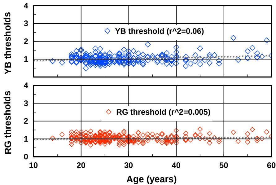
Figure 13: Effect of age on the YB and RG chromatic thresholds for normal trichromats under normal daylight conditions. The best-fit line is shown for both sets of data. The correlation coefficients ( r^2 ) for the YB and RG thresholds are 0.06 and 0.005, respectively.
