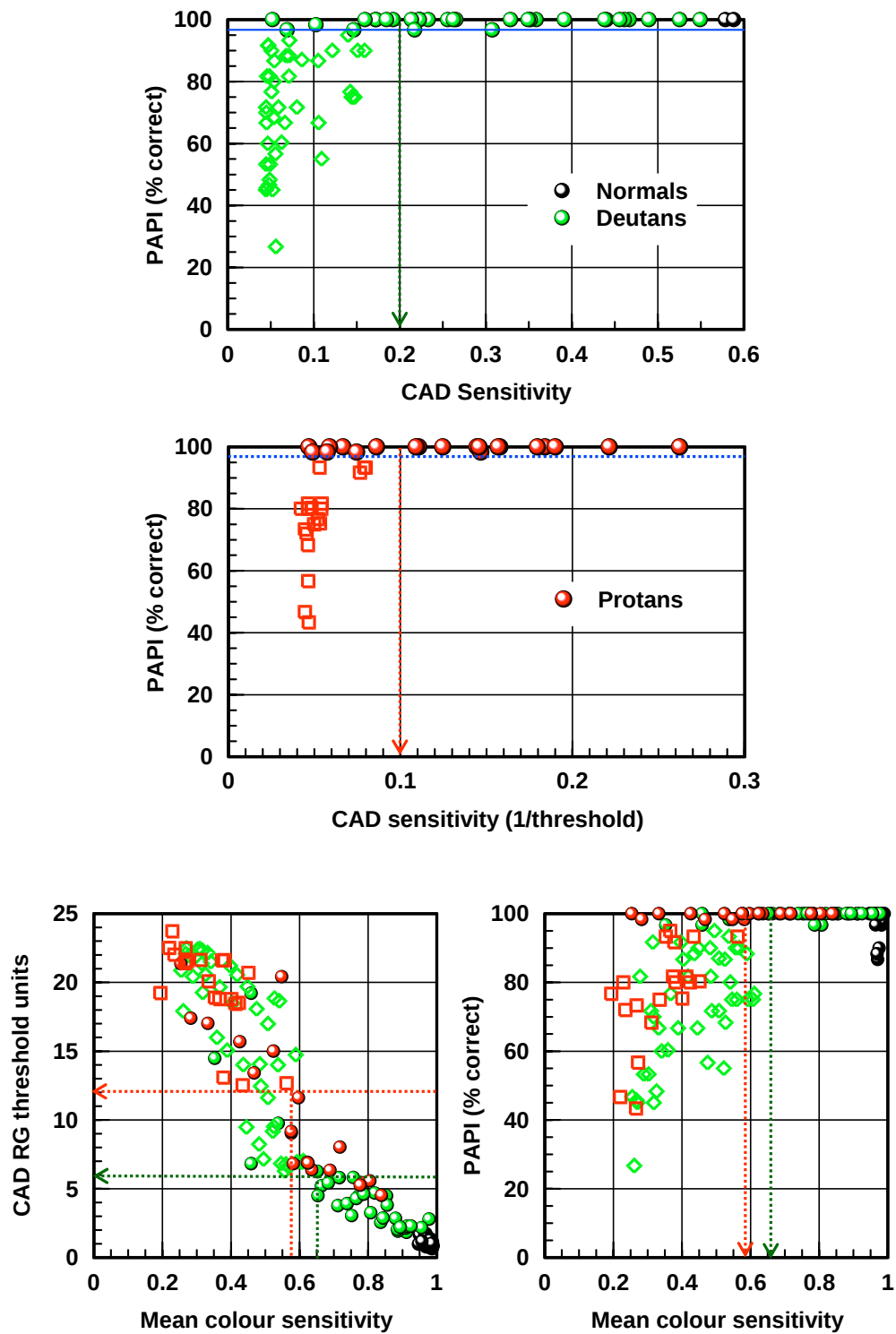
Figure 26: Justification for limits chosen. The top two diagrams compare PAPI (% correct) versus CAD test (sensitivity units=1/RG CAD threshold); color deficient subjects to the right of the dotted line perform the PAPI test as well as normal trichromats do. CAD sensitivity of 0.2 and 0.1 corresponds to 6 and 12 CAD threshold units, respectively, for deutans and protans. Note the change of horizontal scale units for protan observers. The bottom diagrams compare: left, CAD RG threshold units and right, PAPI performance, versus the “mean” or overall color sensitivity as computed by averaging the subject’s performance on the Ishihara, Dvorine, ALT and Nagel anomaloscope tests.
