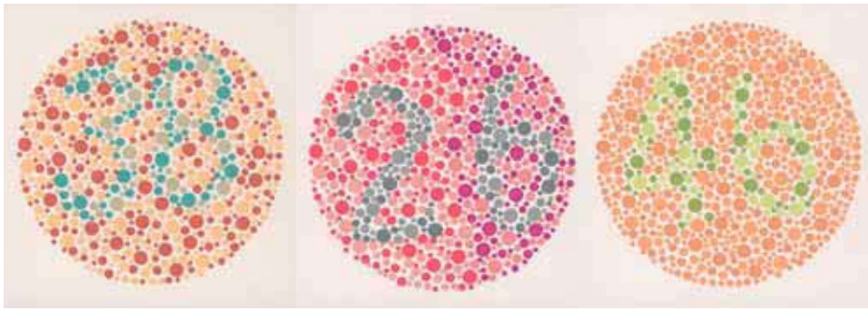
Figure 4: Dvorine pseudoisochromatic plates; left and right, vanishing design; middle, protan/deutan classification plate. Please note that the color of the plates may not be reproduced accurately in this document or in print since the printed reflectances and the viewing illuminant will be different.
