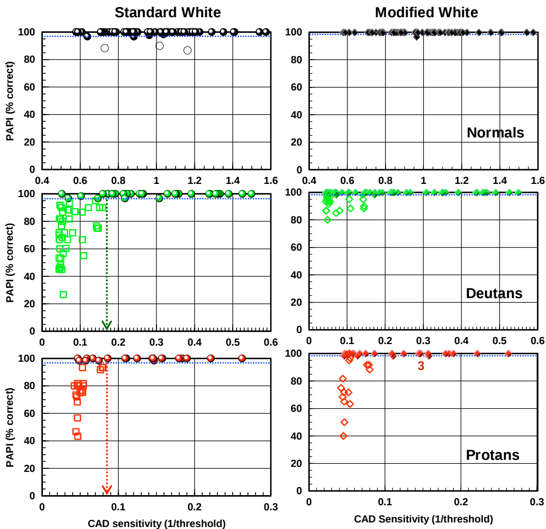
Figure 24: Graphs showing comparisons between standard and modified white (color-corrected white) versus the CAD test sensitivity values.
