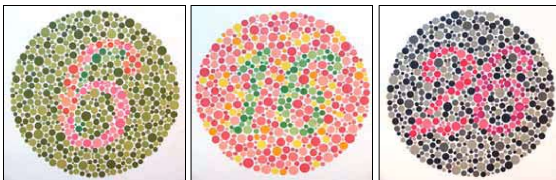
Figure 3: Ishihara pseudoisochromatic plates; left, transformation design; middle, vanishing design; right, protan/deutan classification plate. Please note that these may not be reproduced accurately as the printed color and the viewing illuminant will be different.
