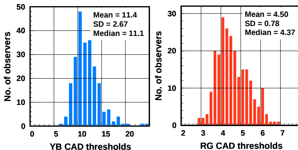
Figure 8: Frequency distributions of the YB and RG chromatic thresholds obtained in 250 observers with ‘normal’ trichromatic vision. The mean, standard deviation (SD) and median are shown.
