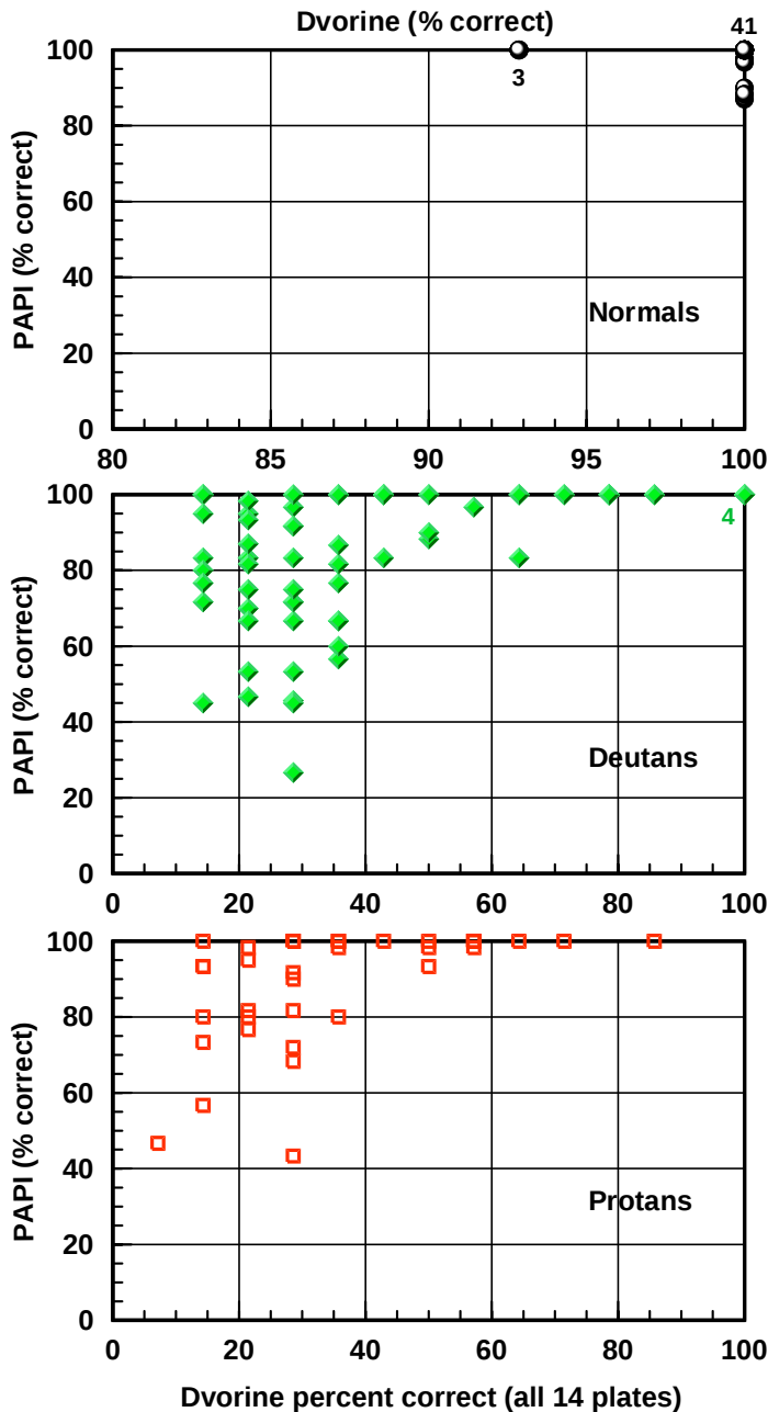
Figure 20: PAPI percent correct scores plotted as a function of the number of plates read correctly on the Dvorine test (expressed as a percentage) for normals, deutan and protan observers.
