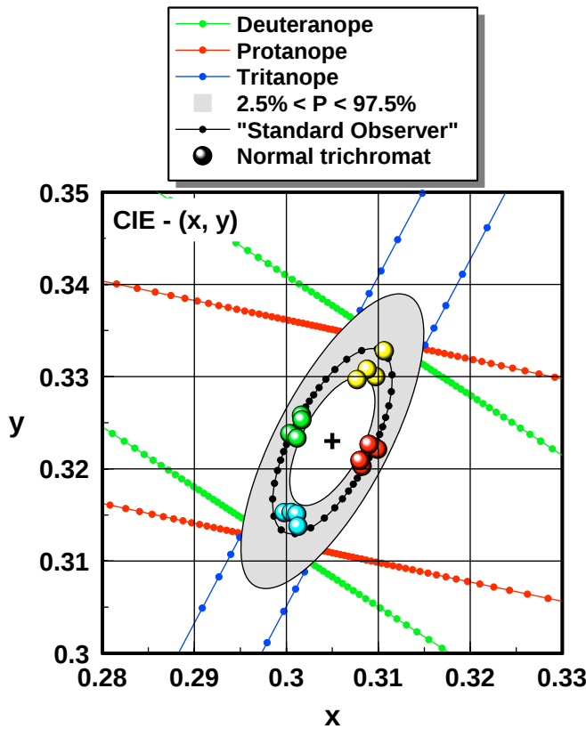
Figure 9: Data showing the 97.5 and 2.5% statistical limits that define the “standard” normal CAD test observer. The dotted, black ellipse is based on the median RG and YB thresholds measured in 250 observers. The grey shaded area shows the limits of variability of 95% of these observers. The deuteranopic, protanopic and tritanopic confusion bands are displayed in green, red and blue, respectively. The background chromaticity (x,y) is indicated by the black cross (0.305, 0.323). The colored symbols show data measured for a typical normal trichromat.
