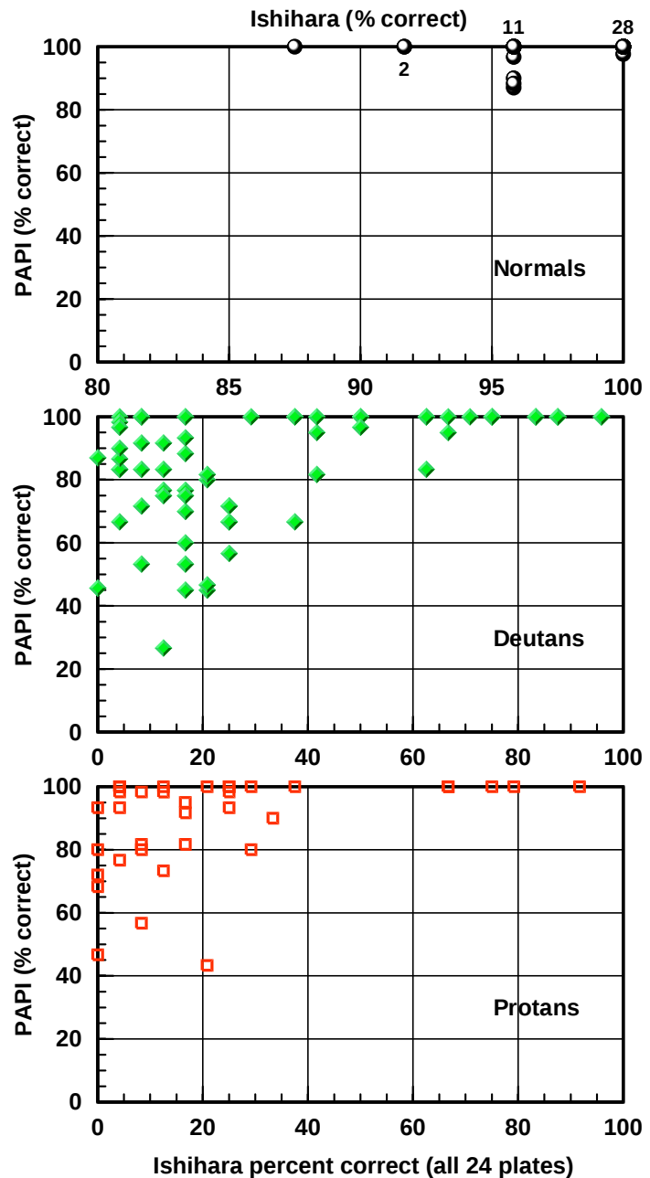
Figure 19: The number of plates read correctly expressed as a percentage on the Ishihara test (24 plates) is compared to performance on the PAPI simulator test separately for normals, deutan and protan color vision observers. The x-axis for the top graph has been expanded to show clearer the errors made by normals.
