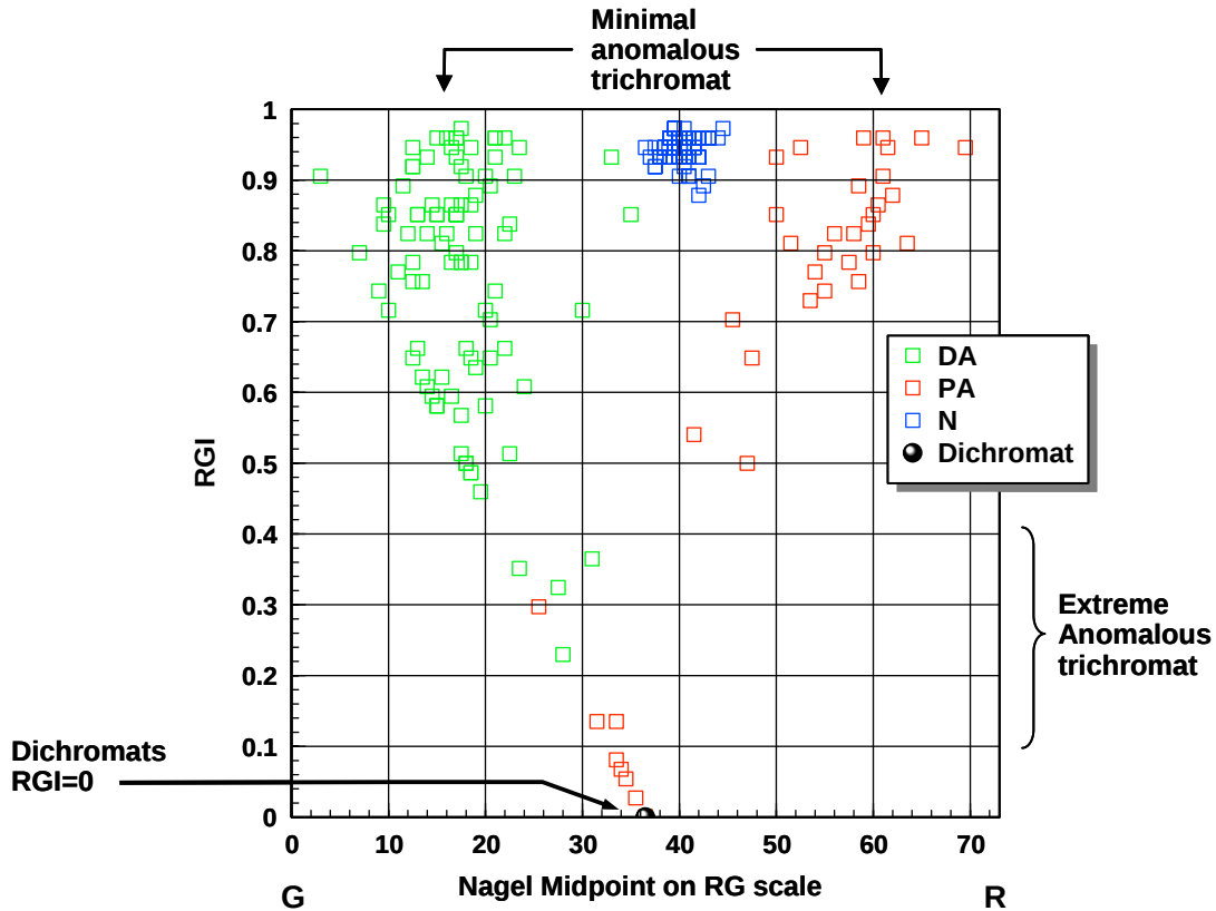
Figure 6: Scatter plot of matching midpoints versus RGI for 231 observers; 70 subjects formed a cluster that is separated from all other subjects by having a midpoint around 40 and a high RGI. The abbreviations in the legend refer to deutanomalous (DA), protanomalous (PA), and normal trichromat (N) subjects. The value of the luminance setting on the yellow scale provides additional information to separate deutan and protan color deficient observers. The data show clearly that according to the Nagel test, many deutan and protan subjects have RG chromatic sensitivity that is indistinguishable from the range of values measured in normal trichromats.
