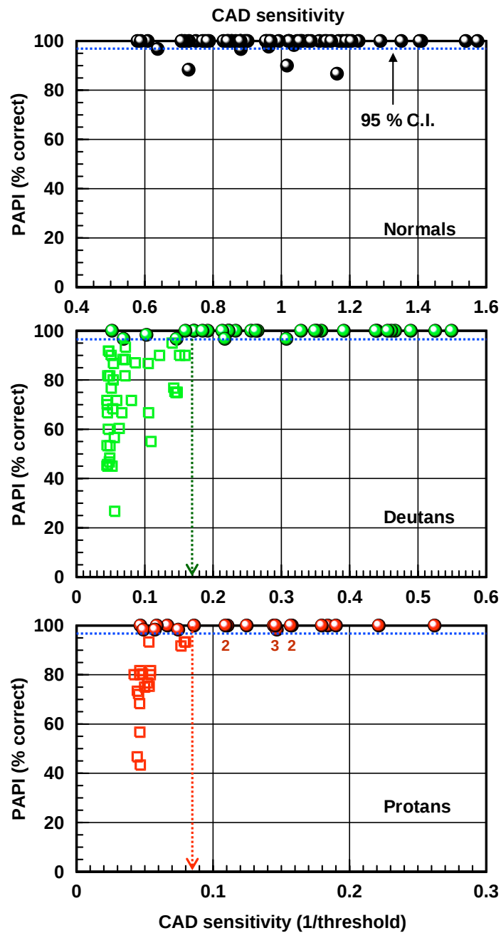
Figure 23: Graphs showing performance of normal, deutan and protan observers on the PAPI (standard white) versus CAD test sensitivity (1/threshold). Note the scale of the x-axis is different for the three graphs for clarity of presentation.
