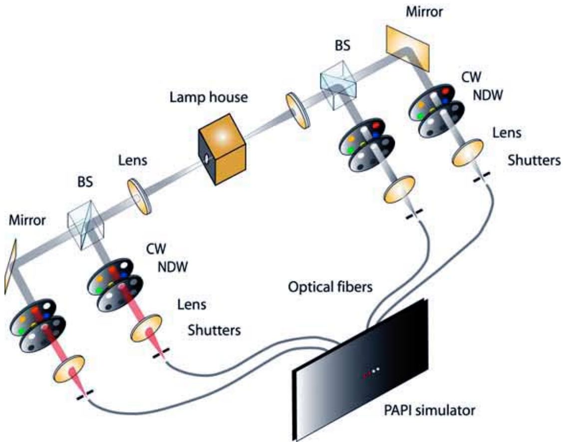
Figure 16: Schematic representation of PAPI simulator designed and constructed for this study. Light emerging from each arm of the lamp house is divided into two channels via beam splitters (BS) to produce four independent channels. Each channel has a color wheel (CW) and a neutral density wheel (NDW) which are controlled by the computer. After passing through appropriate filters, the light from each channel is focused into an optical fiber head which are attached to the viewing panel so as to simulate the PAPI lights.
