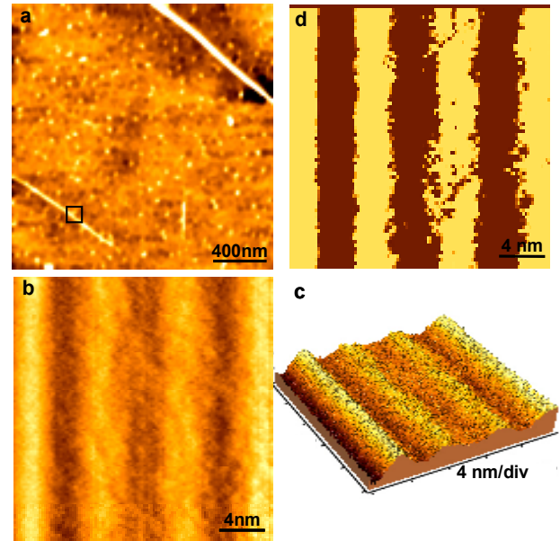
Fig. 2. (a) AFM topographical image of 2\ \mu\text{m} \times 2\ \mu\text{m} scan area, (b) partial atomic resolution AFM topographical image of the area indicated in (a), (c) 3D image of (b) and (d) filtered image of (b) differentiating the topography in two color regime showing the defects in SWNTs.
