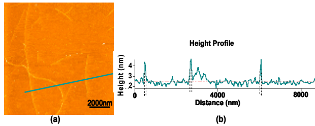
Fig. 1. (a) AFM topographical image ( 10\ \mu\text{m} \times 10\ \mu\text{m} ) of as-grown chemical vapor deposited SWNTs and (b) the related height profile.
