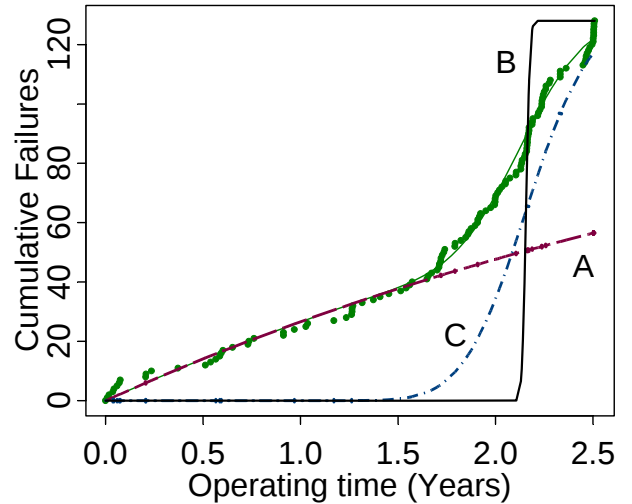
Fig. 5. Model fit to failure data (●) and curves attributed to the different failure components. A) component failure curve with random events only, B) failure curve with evolving heterogeneity in age dependent failure, C) failure curve with the intrinsic heterogeneity in failure components.
