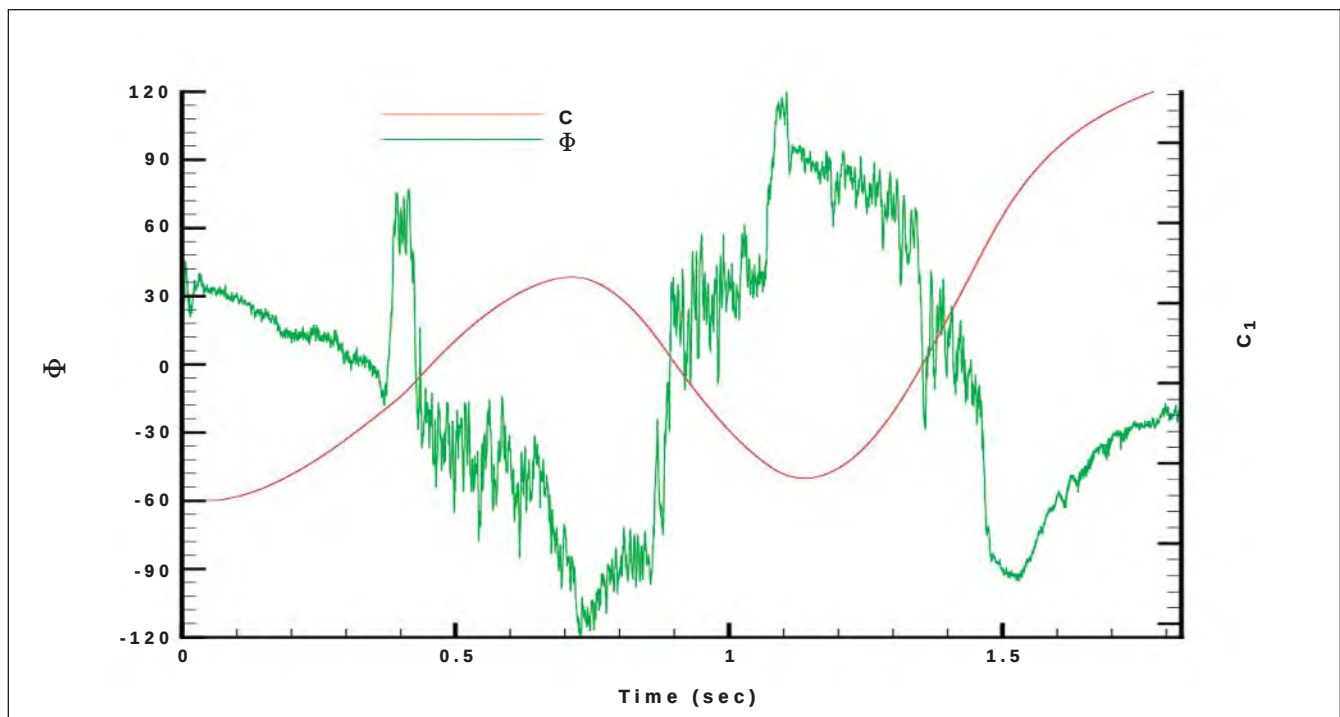
Figure 2. Rolling moment coefficient and bank angle versus time for pitch angle = 6°.
