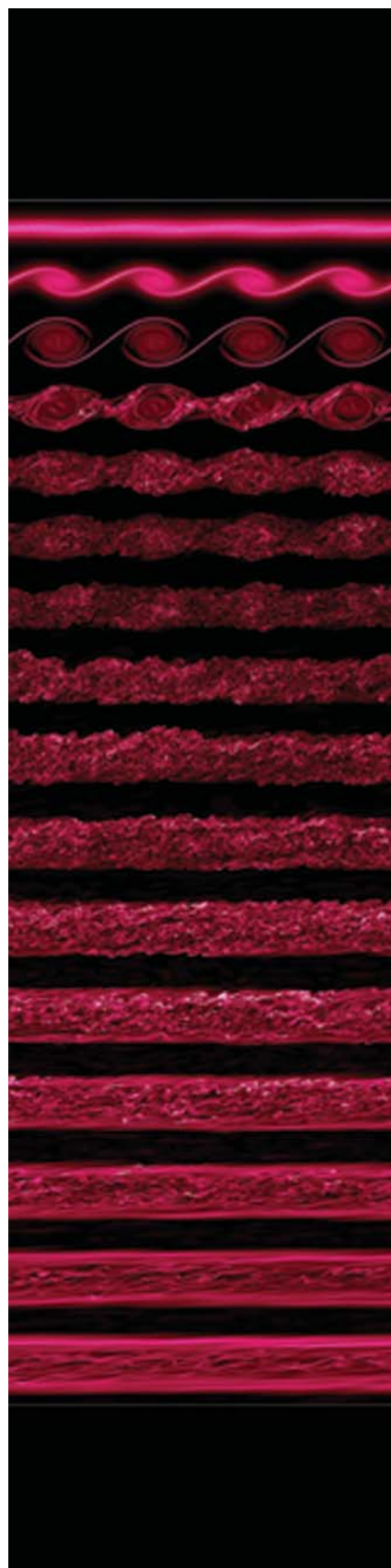
Figure 2. Sequence of images showing vorticity viewed from the side from a wind-shear event encompassing four Kelvin-Helmholtz (KH) billows. Each image is separated by 20 advection time units. The entire event spanned roughly 300 advection units.
