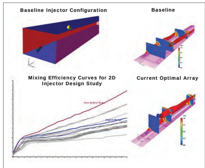
Figure 7. Fuel injector optimization study.
