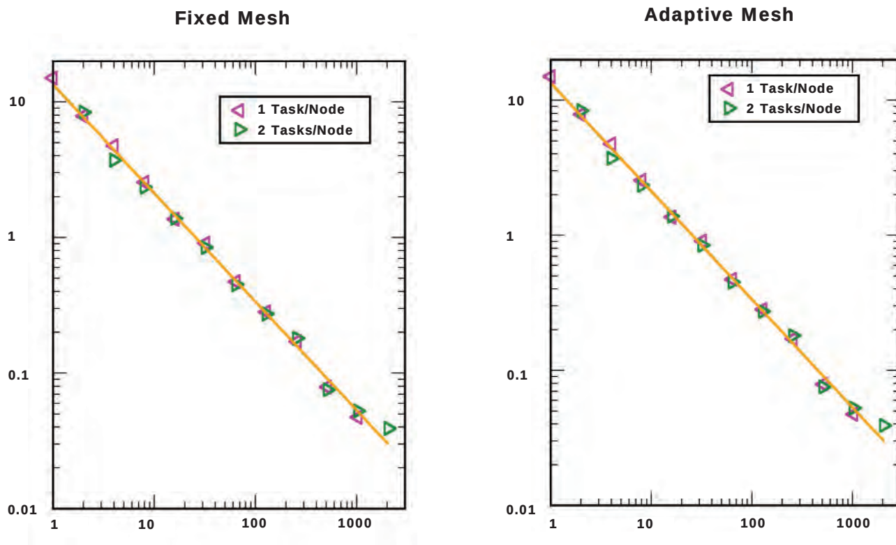
Figure 2. CTH scalability on IBM SP Power 3 and SGI Origin 3800 systems.
