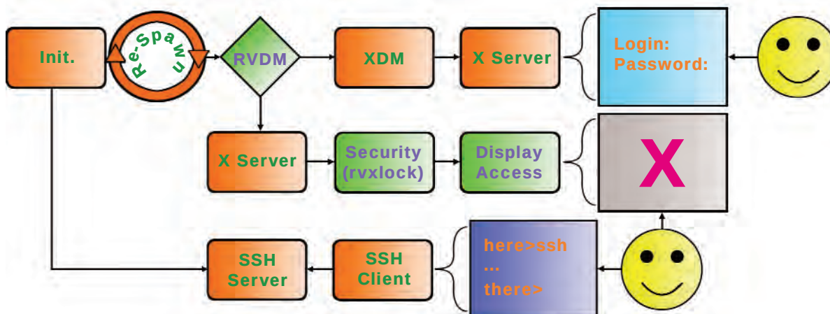
Figure 3. A diagram of the modified initialization procedure using RVRM.
