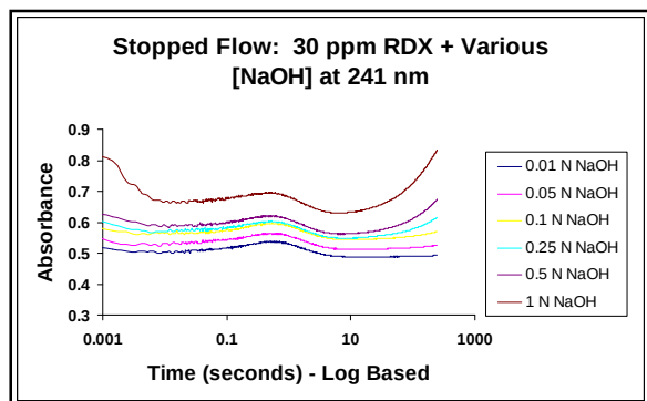
Figure 1. Alkaline hydrolysis of RDX via sodium hydroxide (NaOH)
