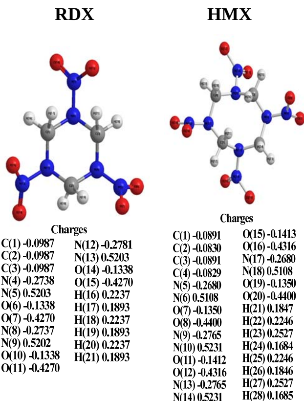
Figure 3. Comparison of charge densities for RDX and HMX
