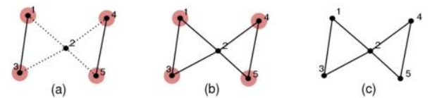
Figure 5. Schematic for finding the marginal contributions of vertex 2 to the overall graph.
