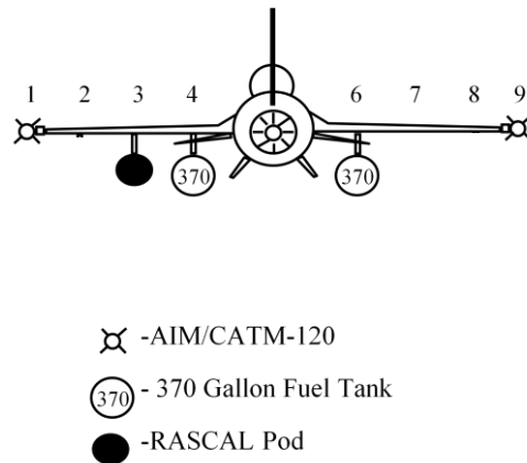
Figure 3: F-16 Configuration for RASCAL CFP and Characterization Flights
