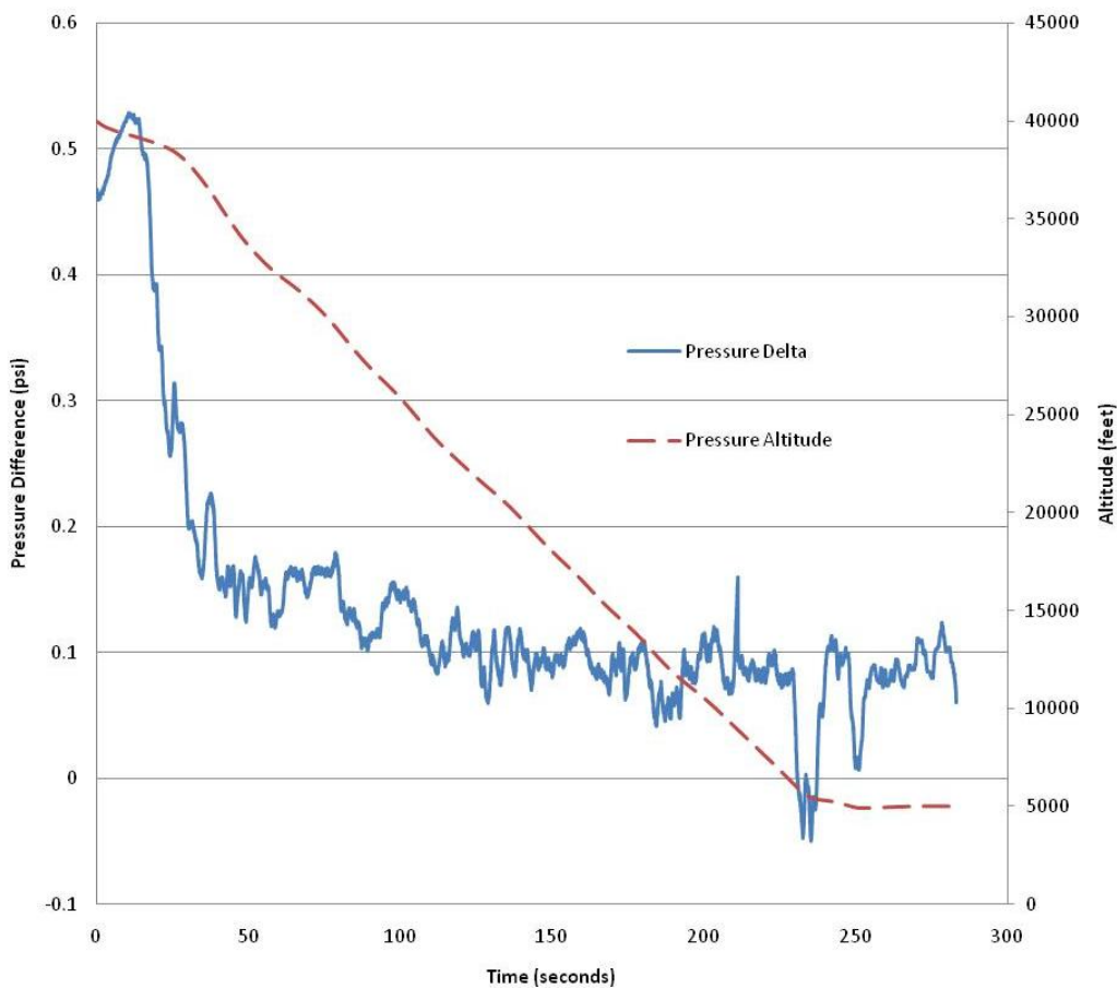
Figure 10: Pressure Difference Between RASCAL Internal and Ambient Pressure during Penetration Descent
