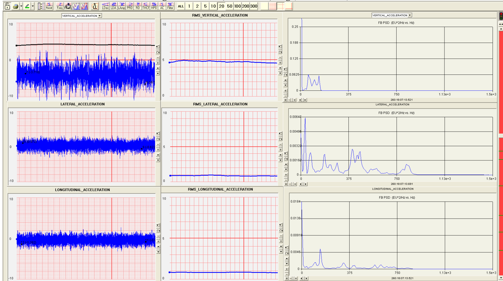
Figure A52: 25K, 312 KCAS, 4.3g (AOA limited)
