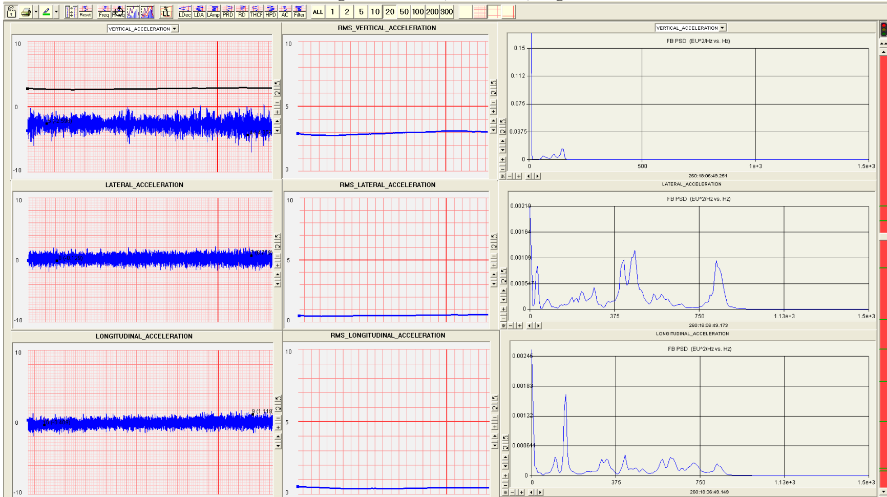
Figure A51: 25K, 312 KCAS, 2.9g
