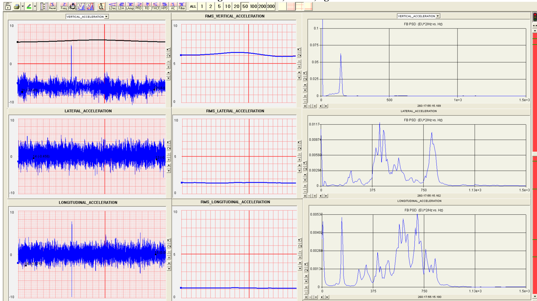
Figure A67: 25K, 1.17M, 6g
