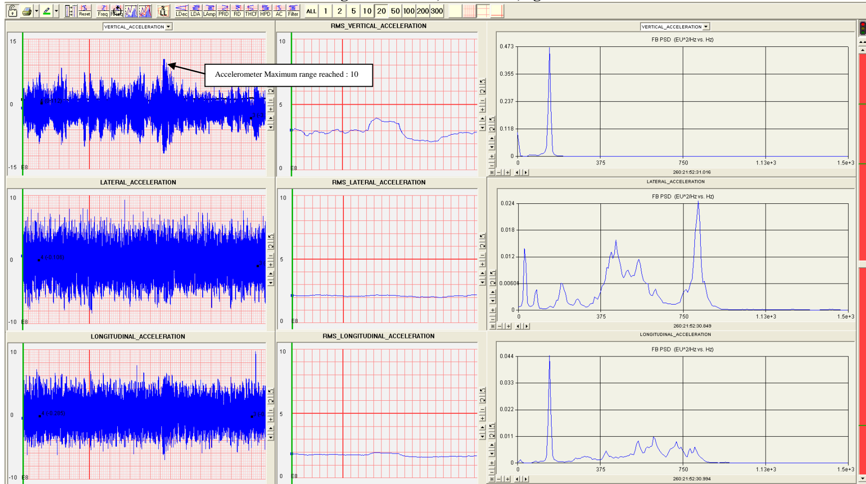
Figure A16: 5K, 535 KCAS, 1g
