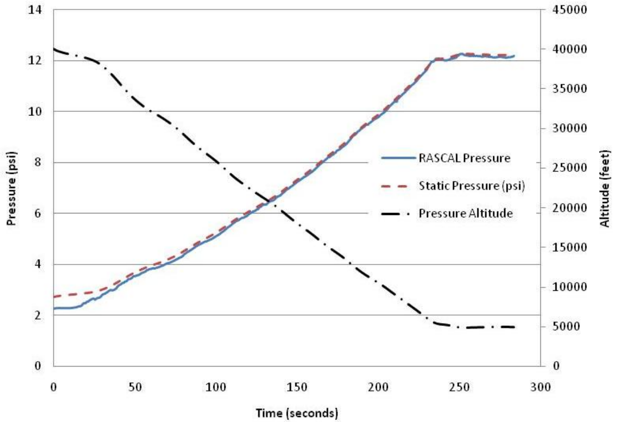
Figure C2: RASCAL Internal and Static (Ambient) Pressure during Penetration Descent
