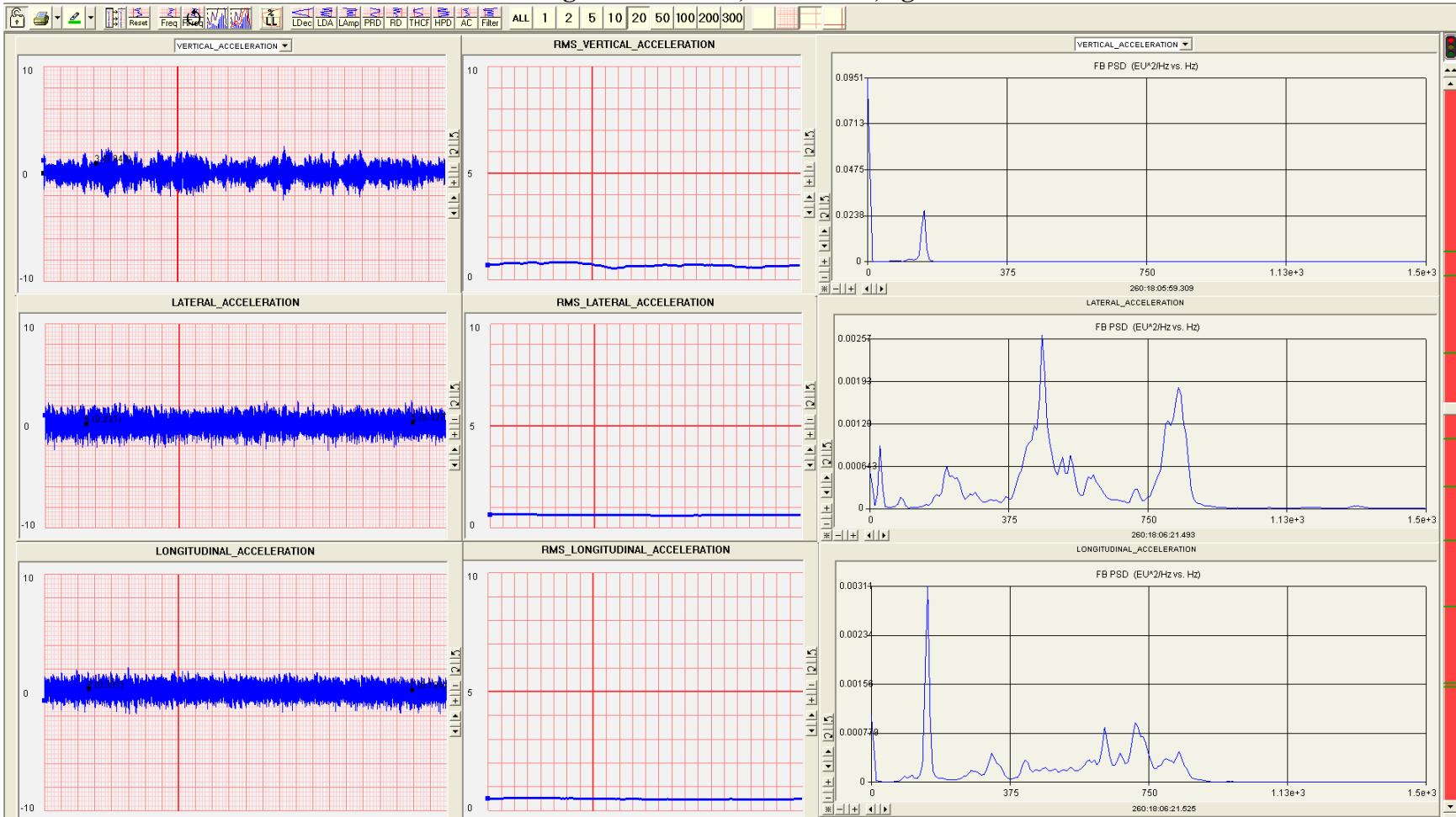
Figure A50: 25K, 312 KCAS, 0g
