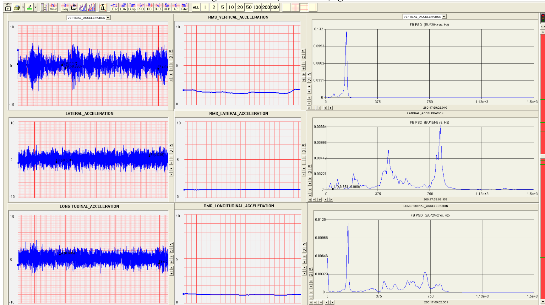
Figure A60: 25K, 428 KCAS, 0g
