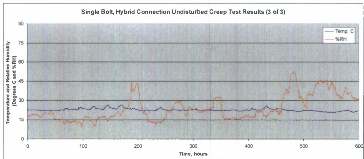
Figure 4.2 – Undisturbed Stress Relaxation Results for All Specimens
