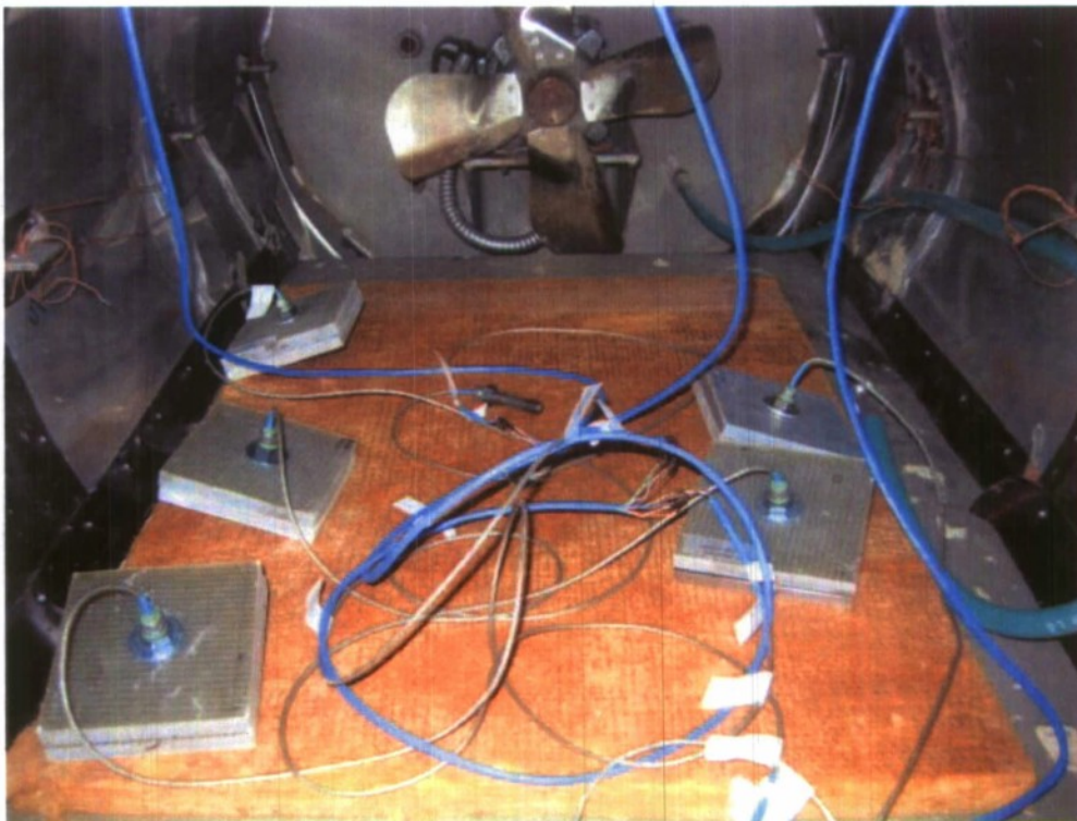
Figure 3.3 – Autoclave Test Setup
