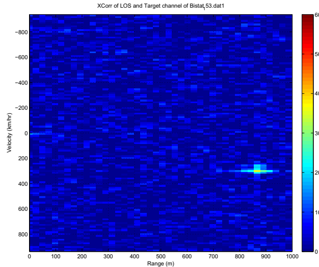
Figure 51: Range/Doppler Surface Plot
