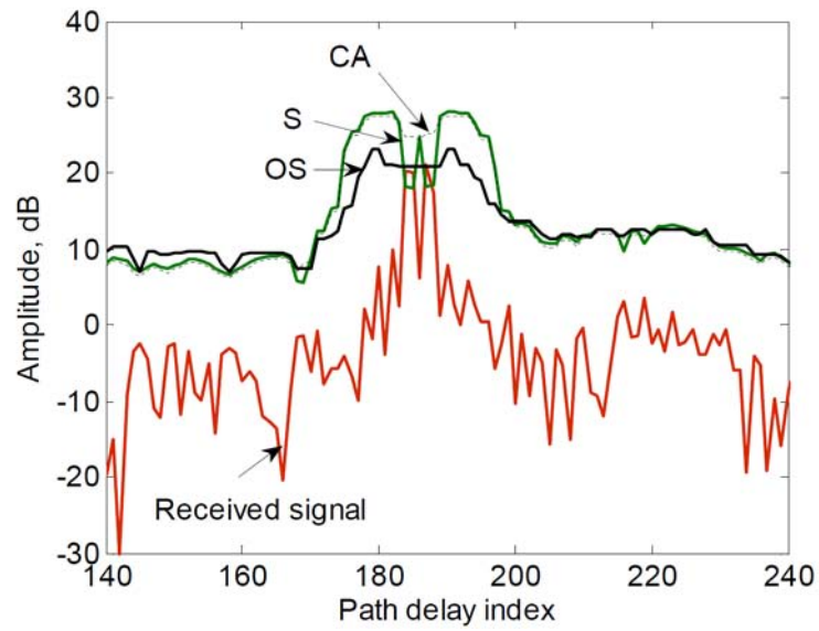
Figure 47: CFAR detection at Doppler 30 Hz
