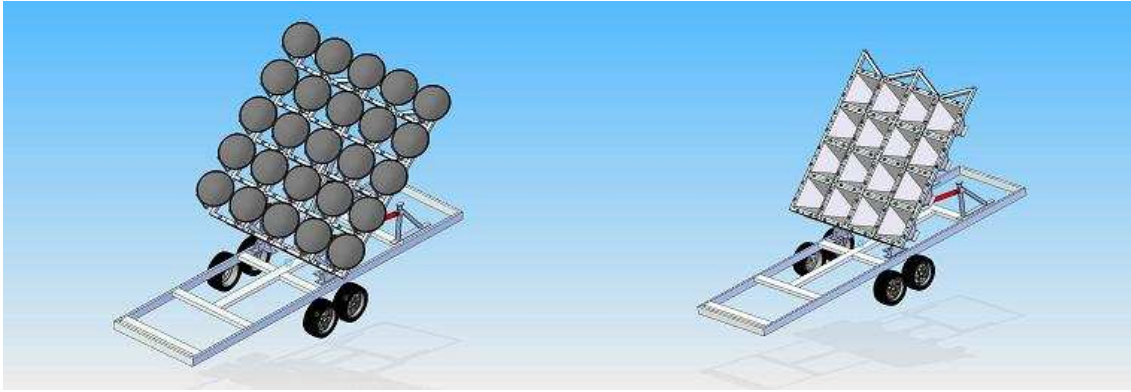
Figure 2: Trailer Array Antenna
