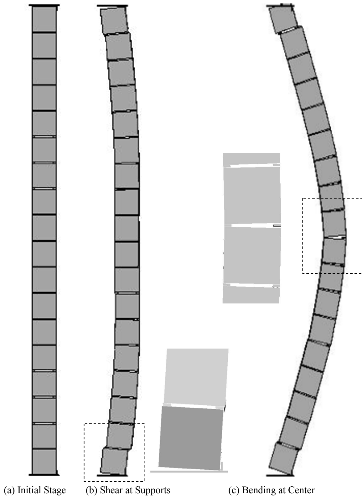
Fig. 7. General Wall Behavior
