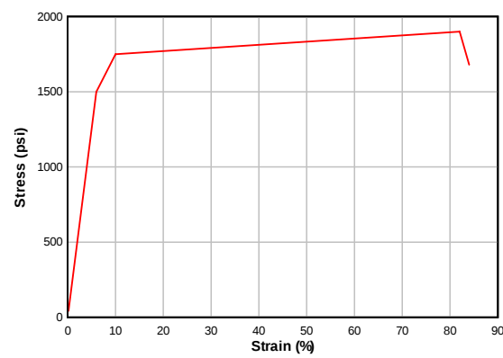
Fig. 5. Static stress-strain curve for the spray-on polymer
