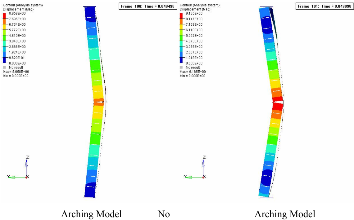
Fig. 16. Wall deflected shape for Test 3
