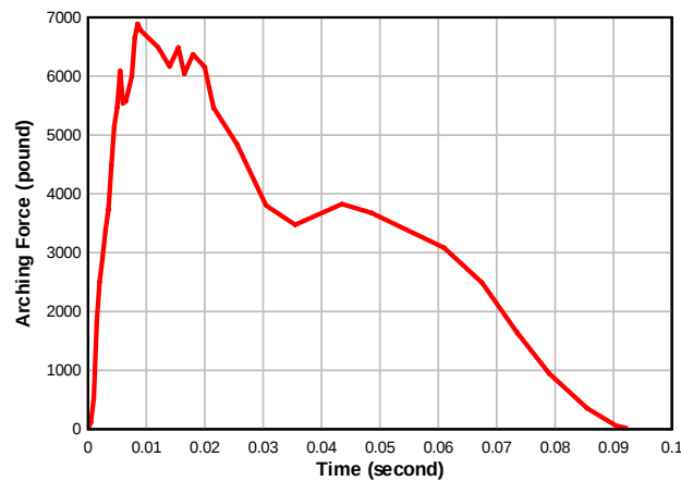
Fig. 14. Arching forces for Test 3
