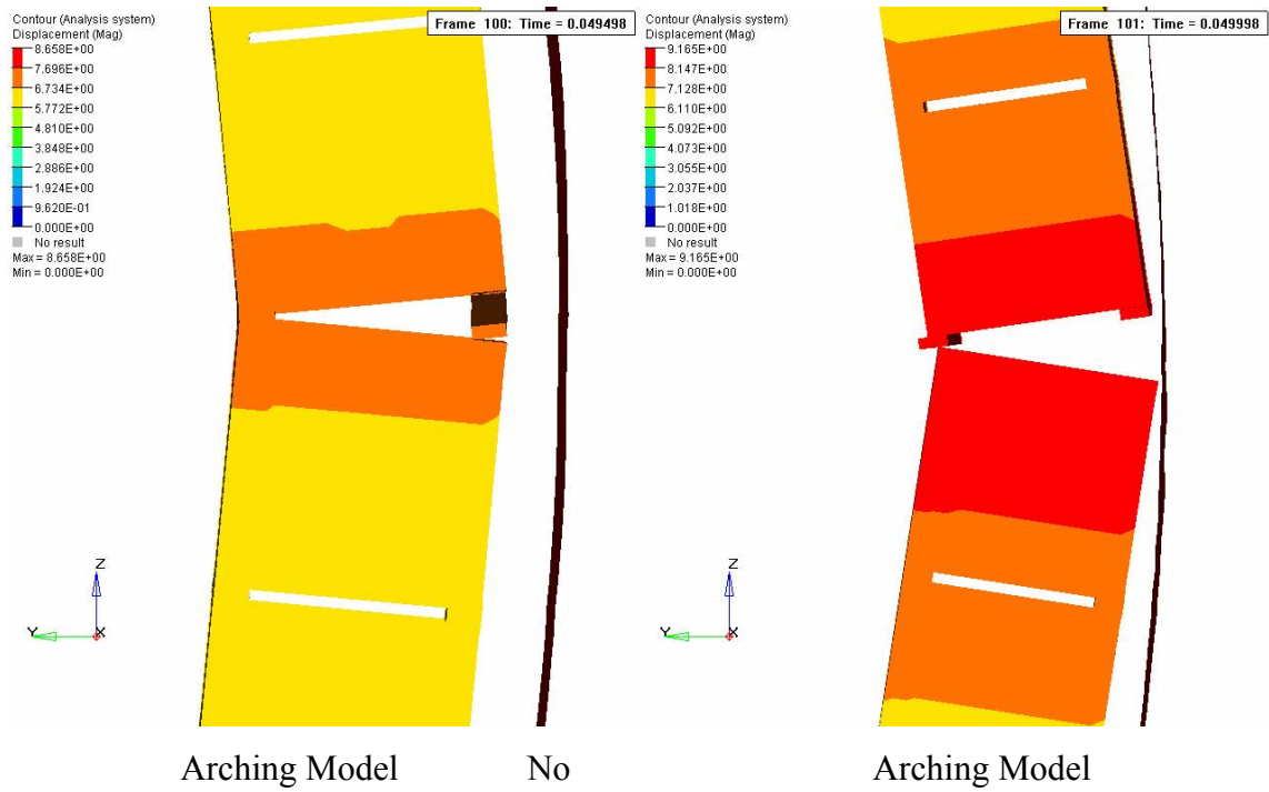
Fig. 17. Mid-point crack details for Test 3
