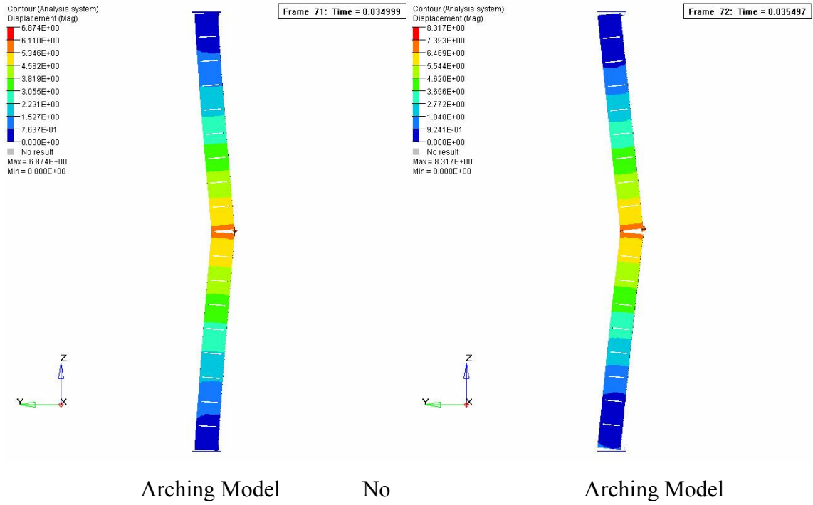
Fig. 12. Wall deflected shape for Test 1
