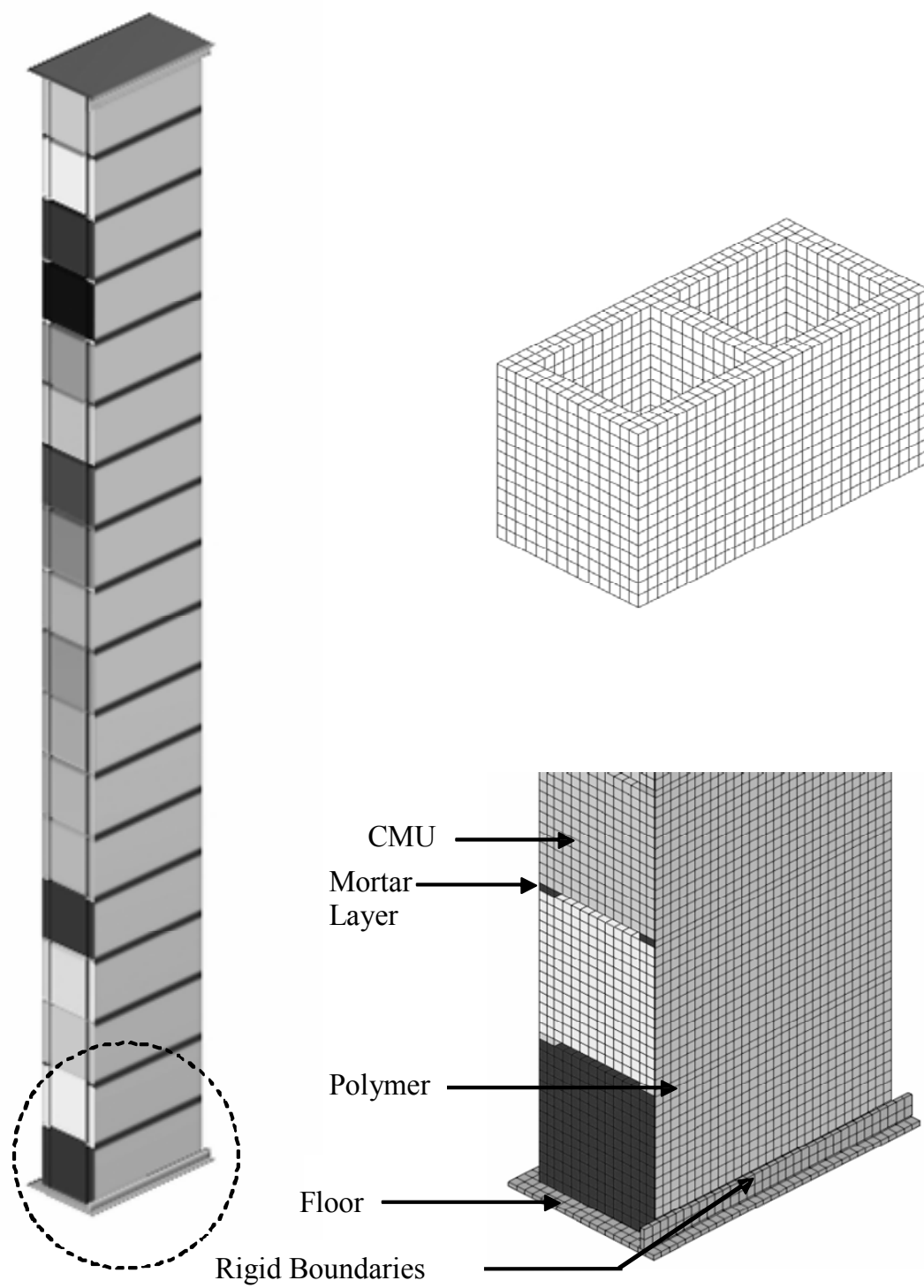
Fig. 6. Baseline model setup
