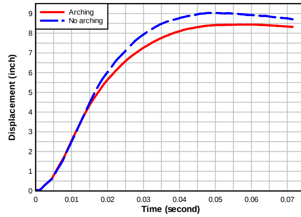
Fig. 15. Wall midpoint maximum displacements for Test 3
