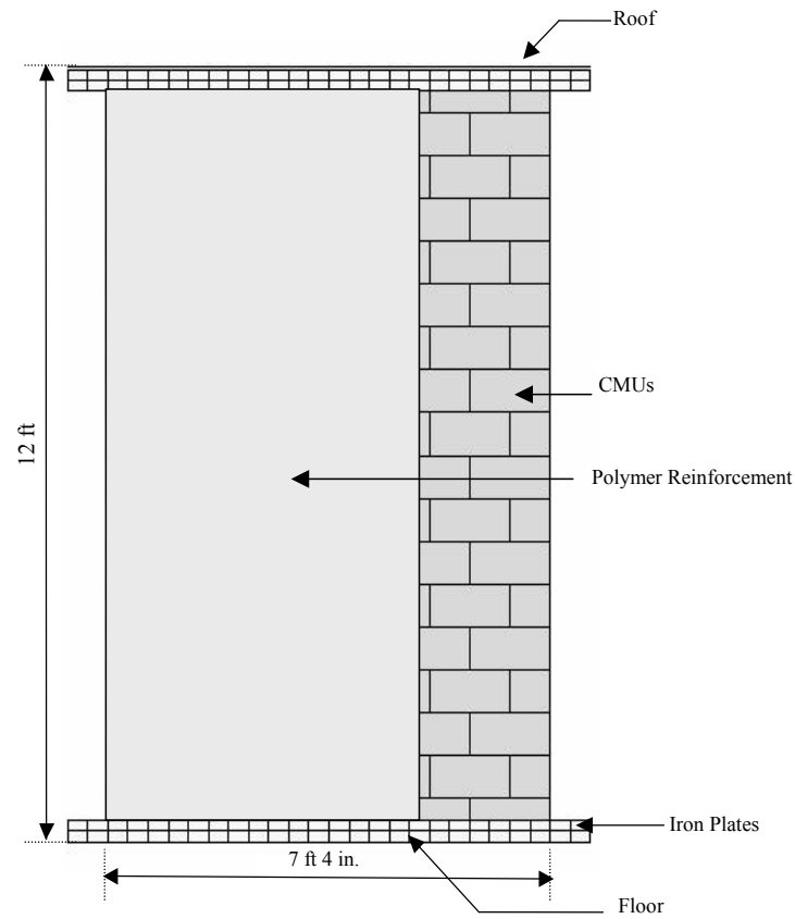
Fig. 4. Schematic of wall setup
