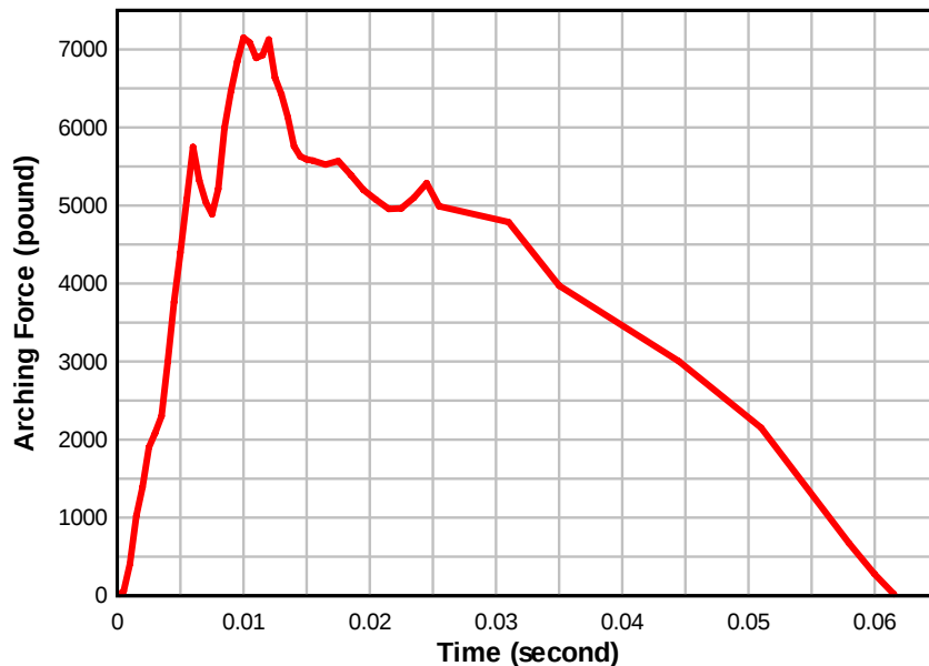
Fig. 10. Arching forces for Test 1
