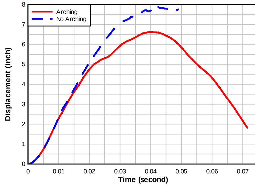
Fig. 11. Wall midpoint maximum displacements for Test 1
