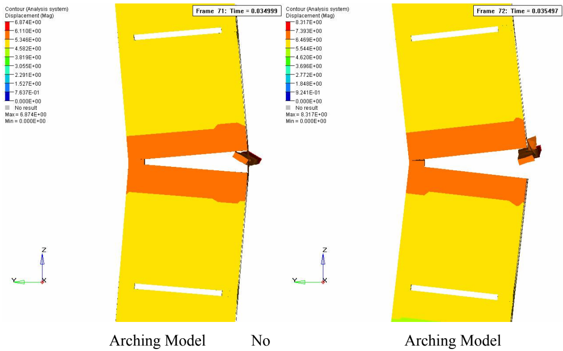
Fig. 13. Mid-point crack details for Test 1
